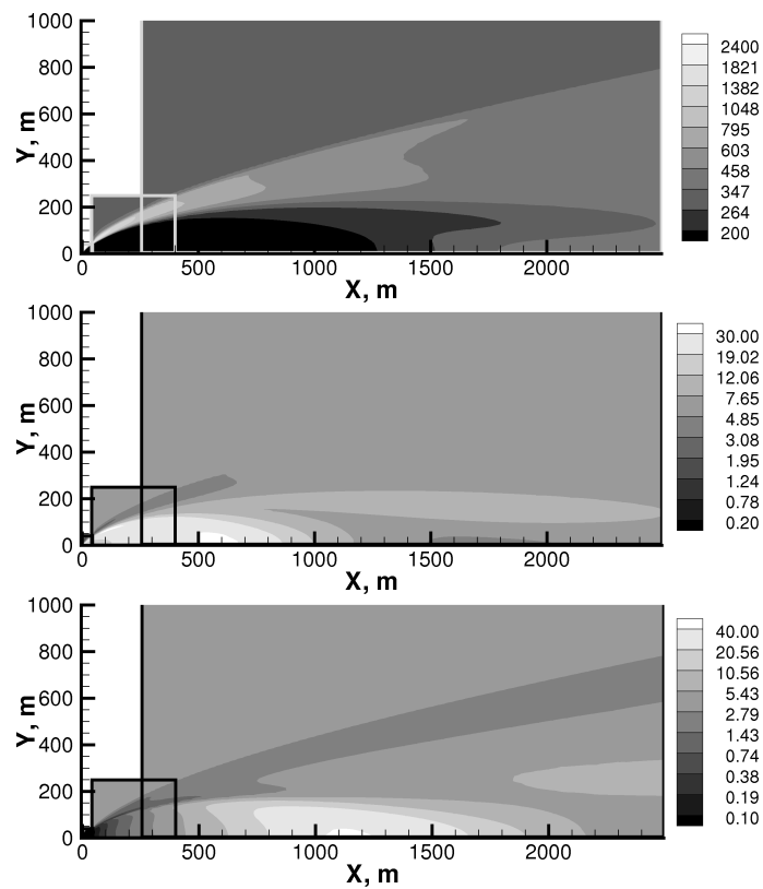
Figure 4. Plume translational temperature in Kelvin (top), Mach number (middle), and gas mean free path in meters.
