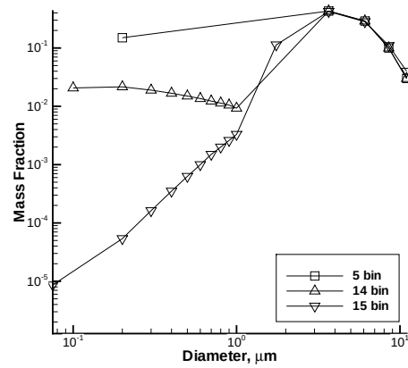
Figure 2. Three particle size distributions.
