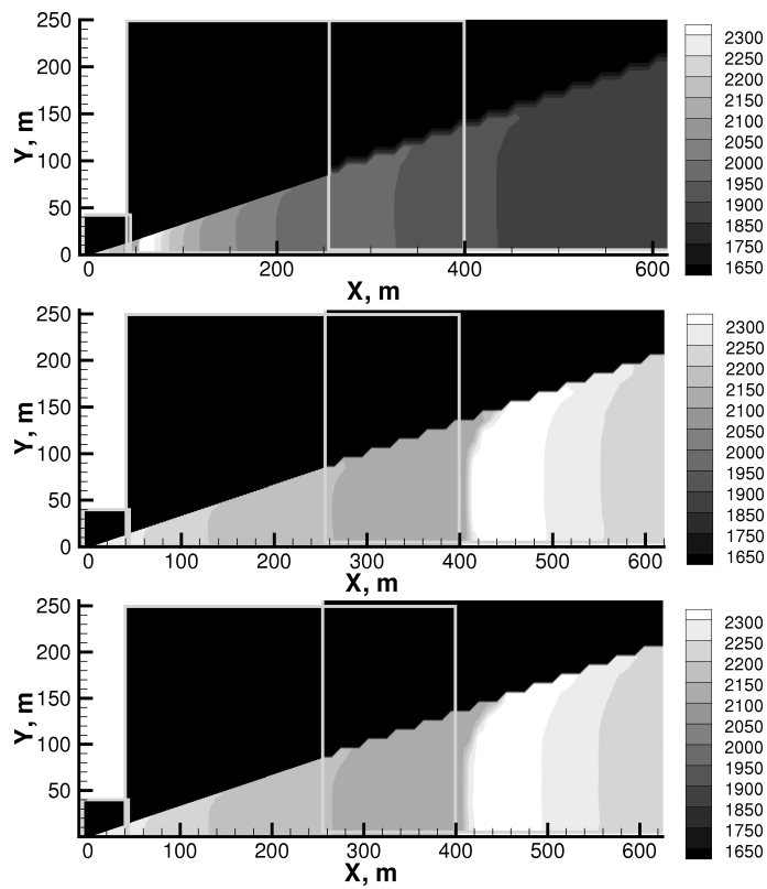
Figure 5. Surface temperature field of 3.66\mu\text{m} particles for Case 1, top; Case 2, middle; Case 3, bottom.
