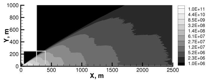
Figure 6. Number density field in \text{kg}/\text{m}^3 of 0.2\mu\text{m} particles.
