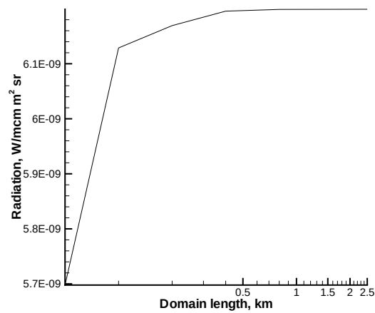
Figure 9. The impact of the far field on the total radiance at 230 \text{ nm} , Case 2.
