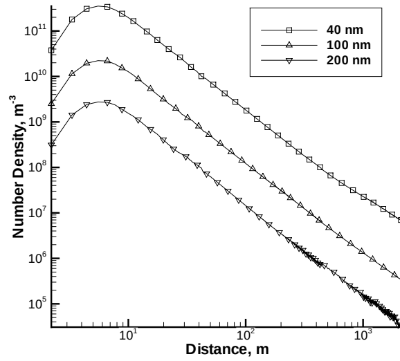
Figure 8. Soot number density along the 25^\circ line of sight.
