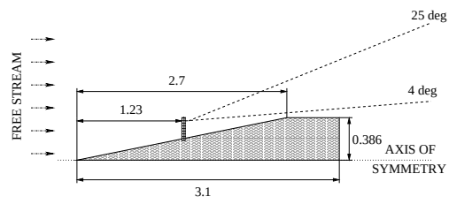
Figure 1. Schematics of the geometrical setup.
