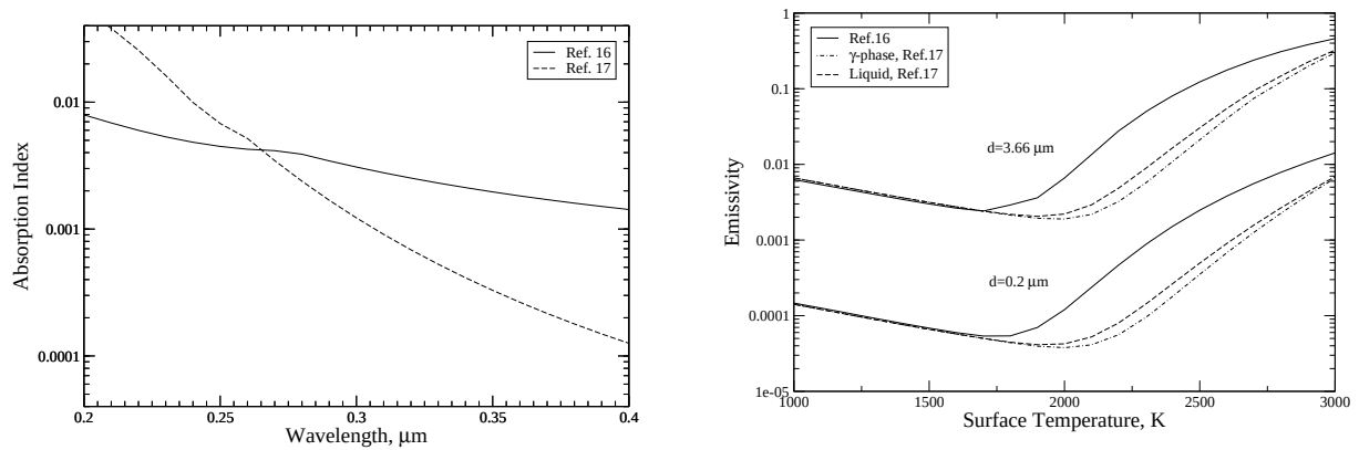
Figure 3. Alumina absorption index calculated with two different sets of expressions, Ref. 16 and Ref. 17 ( \gamma phase), for a surface temperature of 2,200 K (left). Emissivities for two particle diameters computed with these two sets (right).
