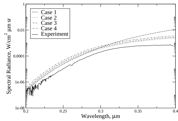
Figure 10. Comparison of spectral radiance for different cases with experimental data.
