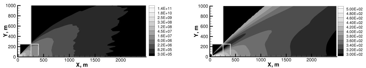
Figure 7. Number density in \text{particle}/\text{m}^3 (left) and surface temperature in Kelvin of 0.1\mu\text{m} diameter soot particles.
