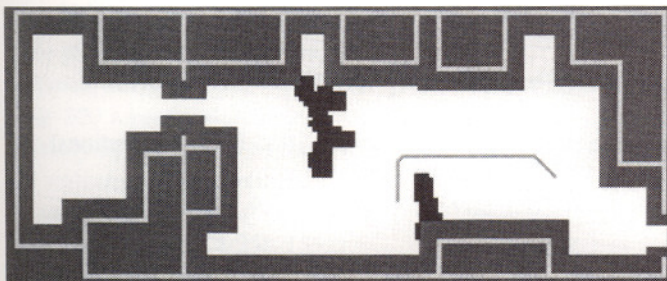
Figure 10: Revised path from robot's new position to accommodate the discovery of the cart.
