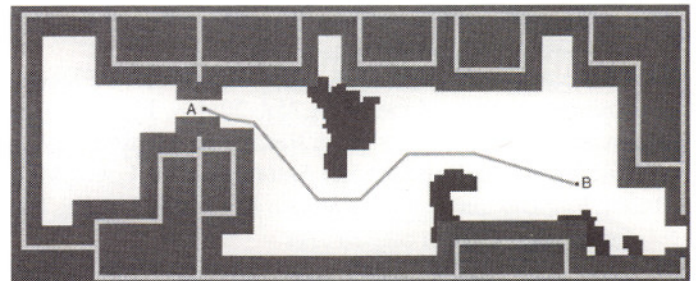
Figure 11: Return path generated by the Planner avoids the previously discovered objects.
