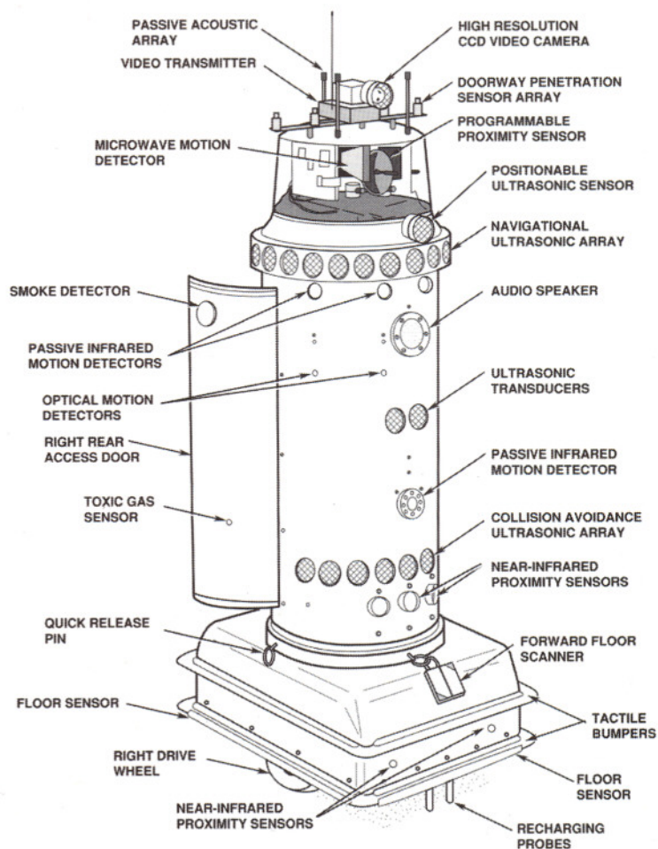
Figure 1: Location of the various security, navigation, and collision avoidance sensors employed on ROBERT II (1982-1992).
