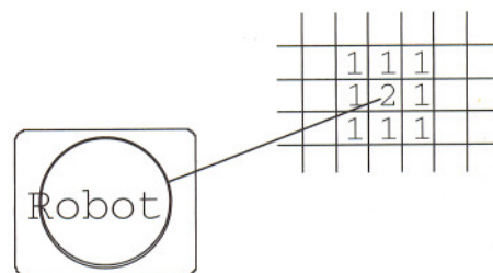
Figure 4: For any objects detected within five feet, the certainty value assigned to the cell at the indicated sonar range and bearing is incremented twice, while the eight neighboring cells are each incremented once.
