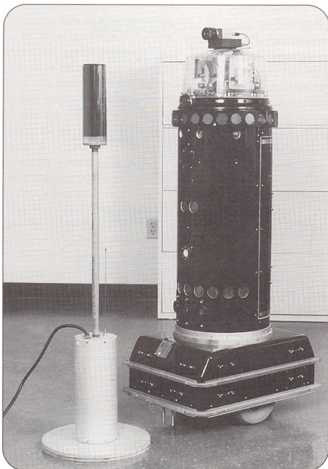
Figure 2: The last known location of the free-standing recharging station is represented in the world model as a special case of a transient object.
