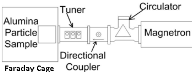
Figure 2. Experimental Setup.
