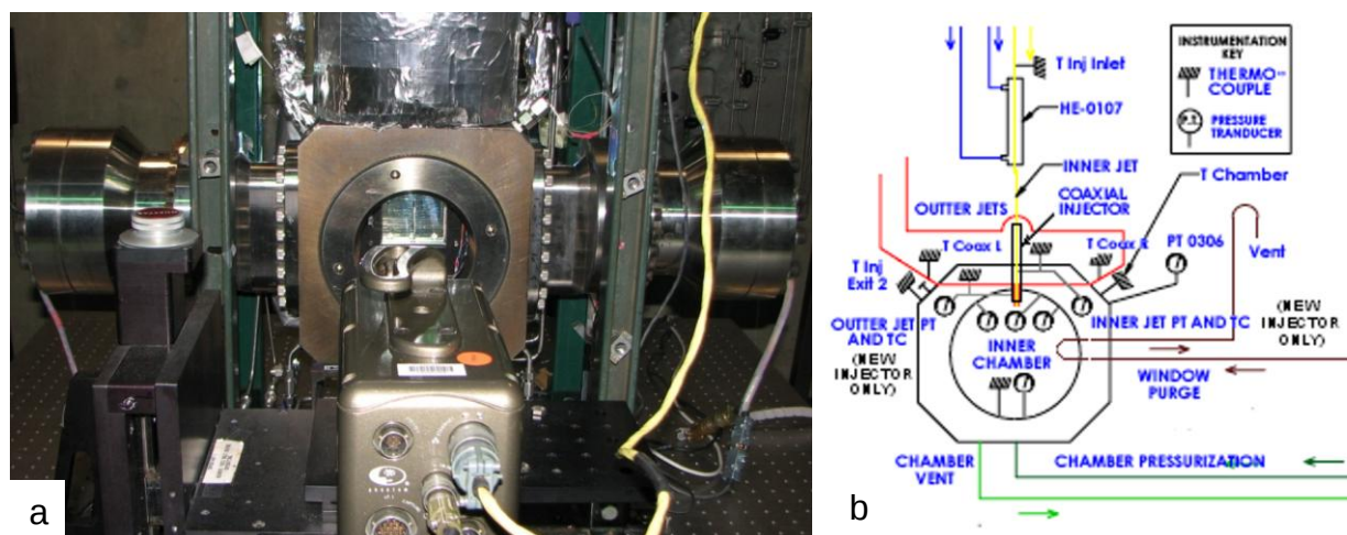
Figure 1a. Experimental test chamber and supporting systems of the Experimental Cell 4 at AFRL, Edwards AFB, CA. b. Chamber section view of the flow schematic for Experimental Cell 4.
