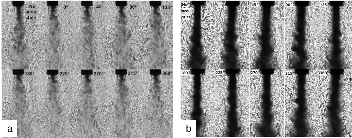
Figure 11.a. Collection of supercritical coaxial jet images at P_{\text{chamber}} = 4.96 MPa, J = 2.4 with original injector geometry. b. Images at P_{\text{chamber}} = 4.95 MPa, J = 2.6 with the new injector geometry.
