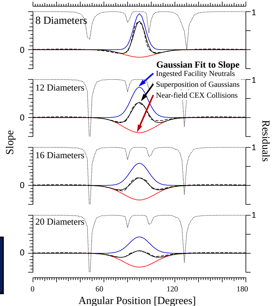
Slope, Residuals, and Gaussian Fit of Linear Extrapolation to Vacuum
