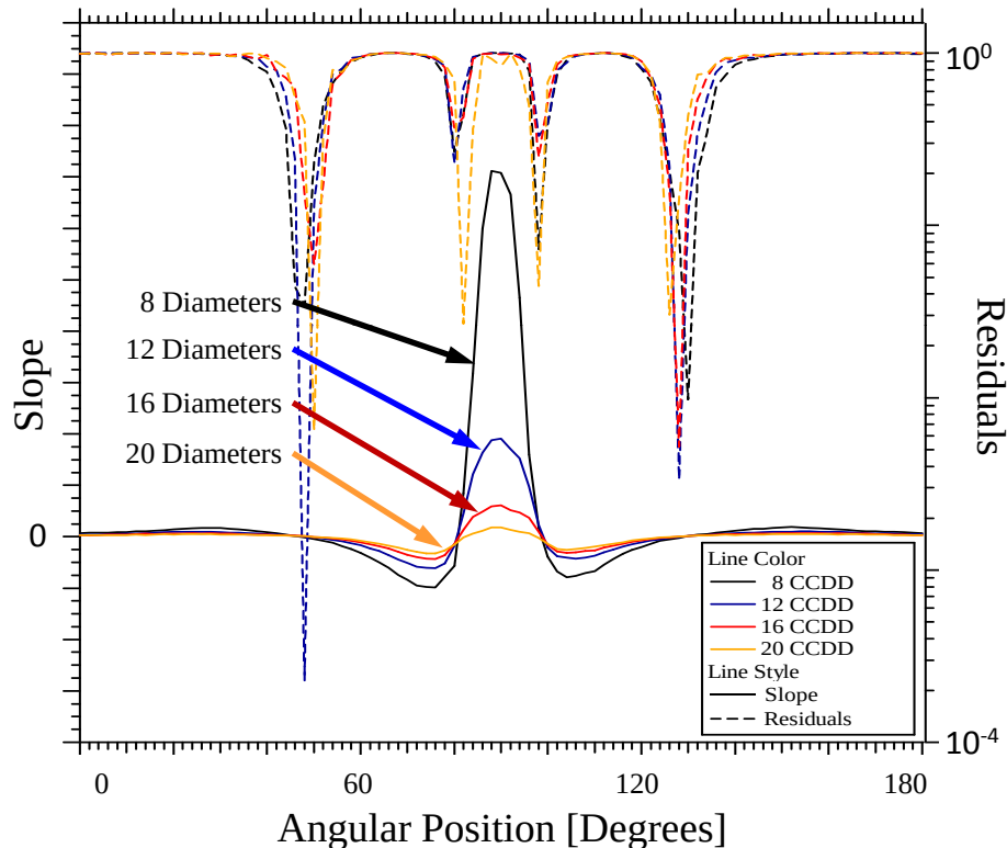
Slope and Residuals of Linear Extrapolation to Vacuum
