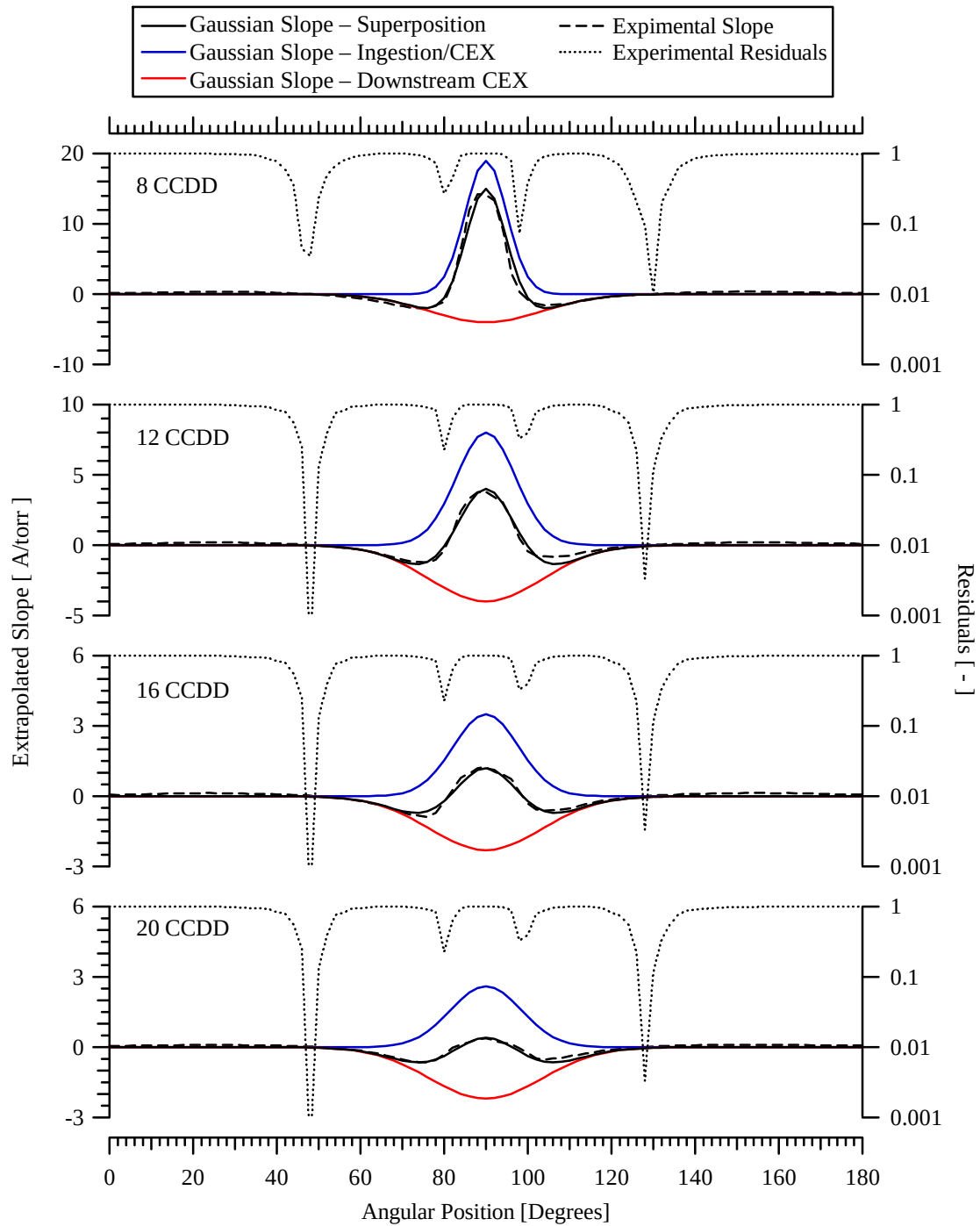
Figure 12. Residuals and slope of the extrapolated collected ion current of the nested Faraday probe Configuration 1 as a function of angular position at 8, 12, 16, and 20 CCDD. A superposition of two Gaussian curves is fit to the experimental slope.
