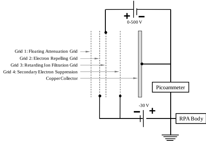
Figure 6. Electrical diagram of the RPA grid power electronics and DAQ system.
