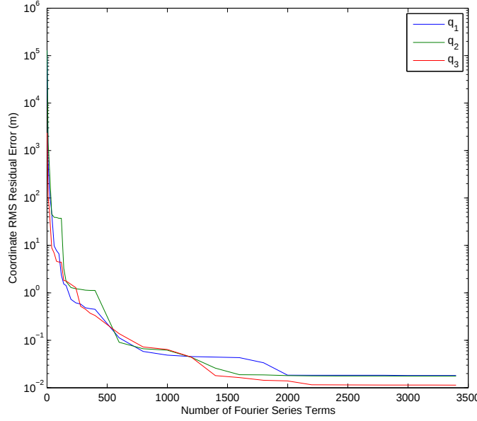
Figure 4.3. Coordinate RMS residuals over 1 year vs. number of series terms for 320km, 30^\circ orbit
