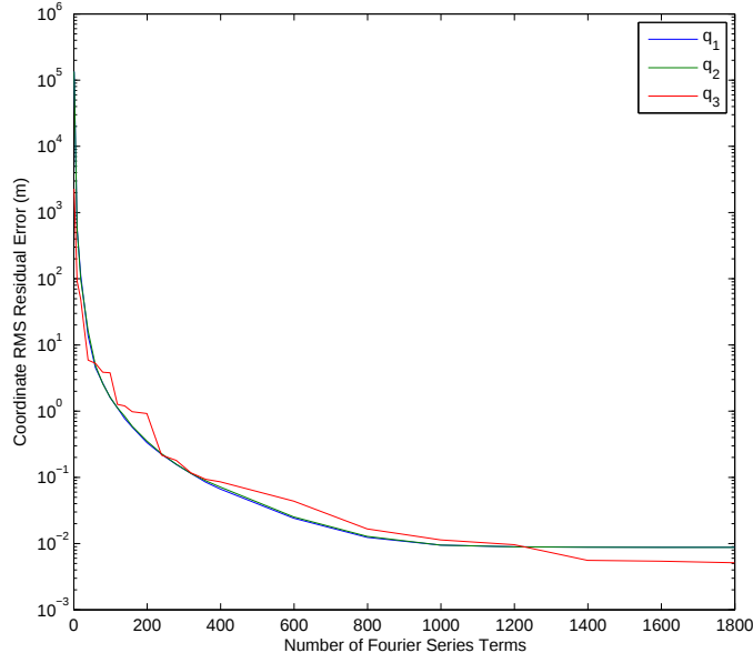
Figure 4.5. Coordinate RMS residuals over 1 year vs. number of series terms for 630km, 30° orbit
