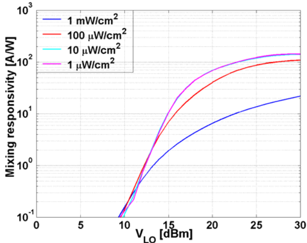
Fig. 3. Predicted mixing responsivity vs. LO voltage for the device of figure 2.
