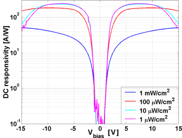
Fig. 2. DC responsivity of a sample OEM device, simulated with SimWindows.
