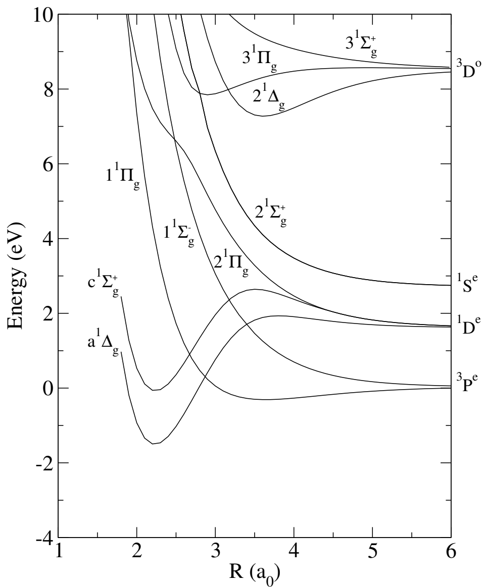
Figure 13. Potential energy curves for singlet methylene states in symmetric collinear (H-C-H) arrangement obtained in valence-shell multiplet carbon 1s^2(2s^22p^2 + 2s2p^3 + 2p^4) and hydrogen ( 1s ) atomic states. The state designations of the curves are as in Figure 11.
