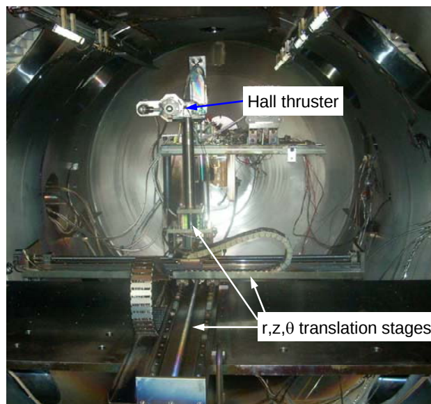
Figure 8. Setup of the 200 W Hall thruster and probe positioning system at the AFIT facility.
