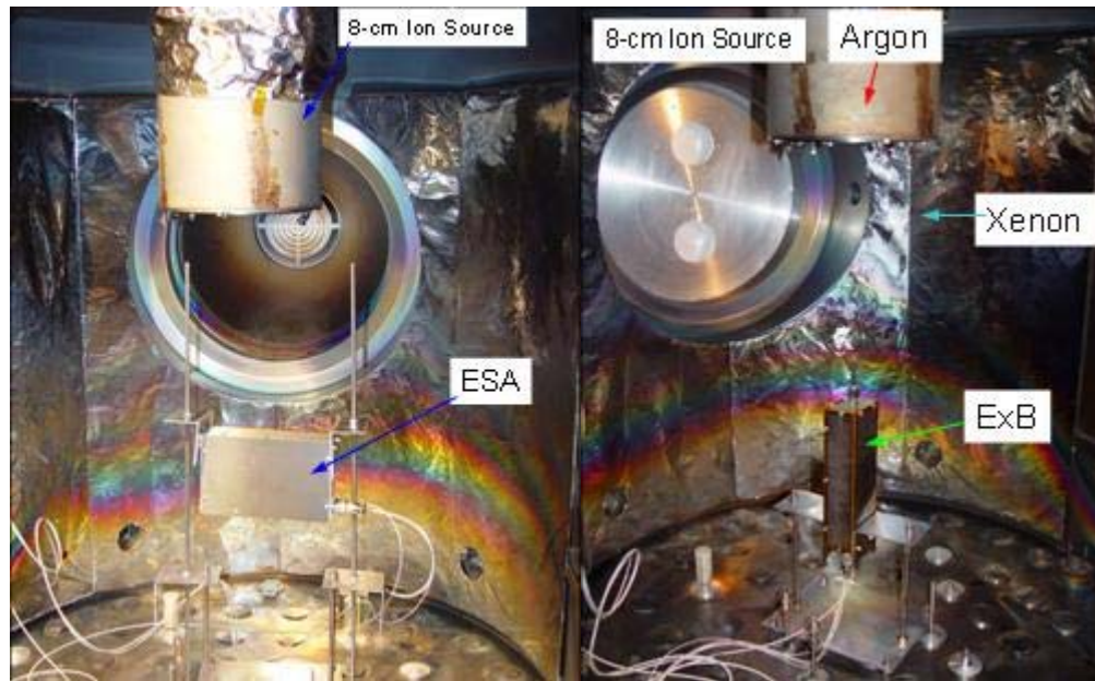
Figure 3: Setup of the ESA (left picture) and ExB (right picture) relative to an 8-cm diameter ion source.
