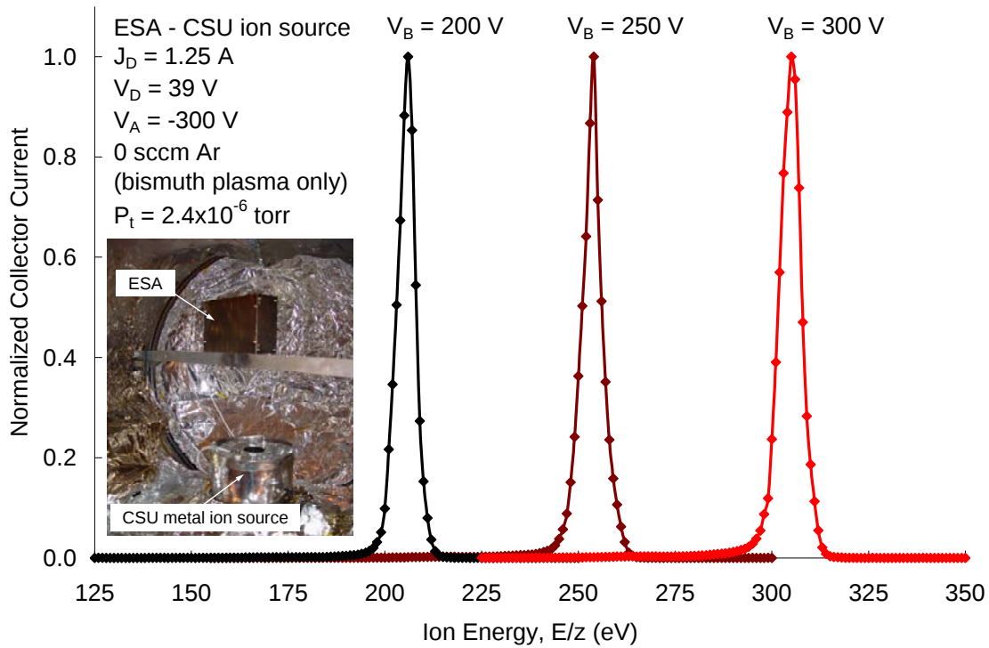
Figure 6: IEDFs of ions produced within a CSU metal ion source. The ion source was operated on bismuth propellant at beam voltages of 200, 250, and 300V.
