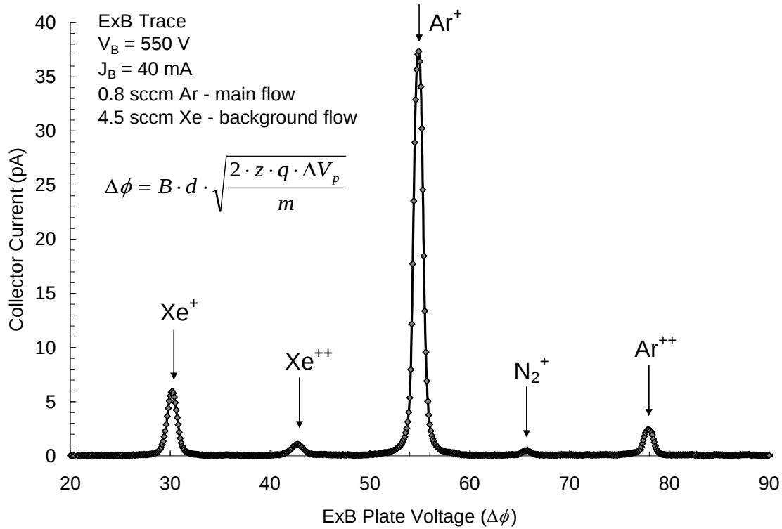
Figure 5. Data taken with the ExB probe of argon and xenon ions from an 8-cm diameter argon ion source at CSU.
