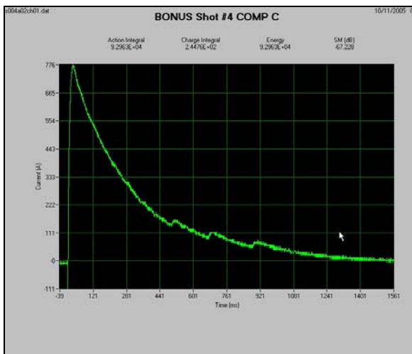
Figure N-10. Example component C Test Waveform.
