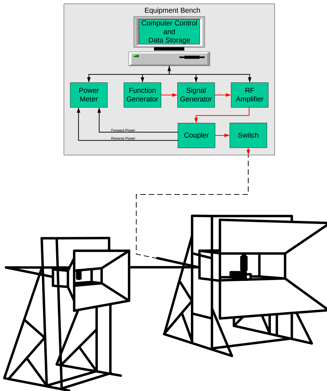
Figure B-1. Typical EME Transmission Equipment and Antennas.
