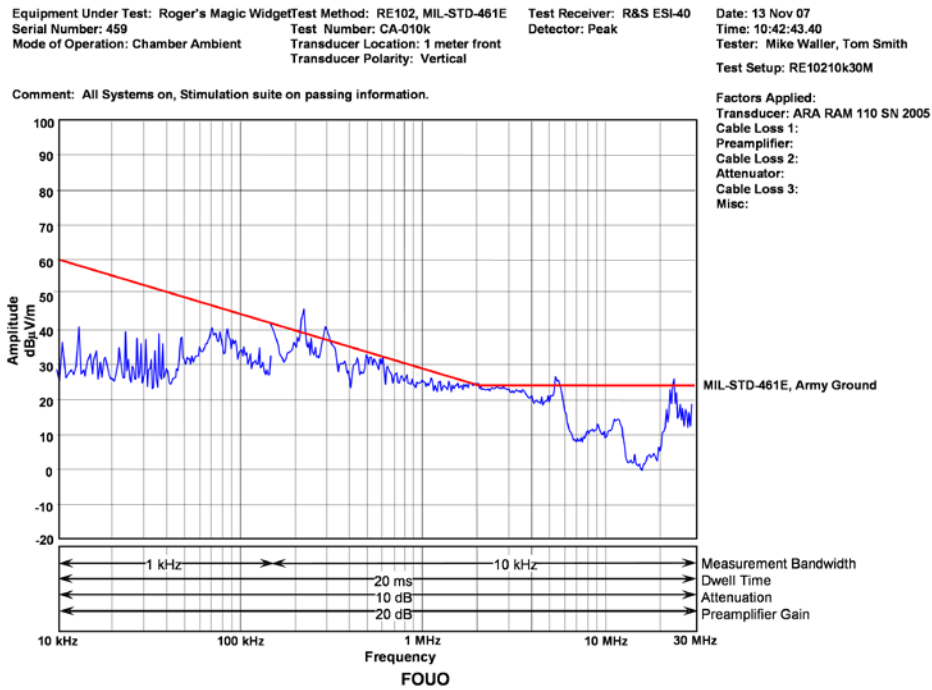
Figure K-4. Sample Emissions Data Plot.
