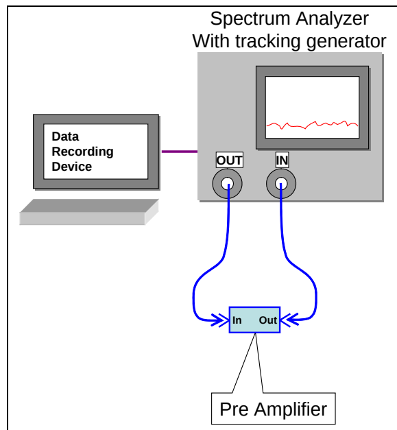
Figure A-2. Preamplifier Check and Gain Test Setup.
