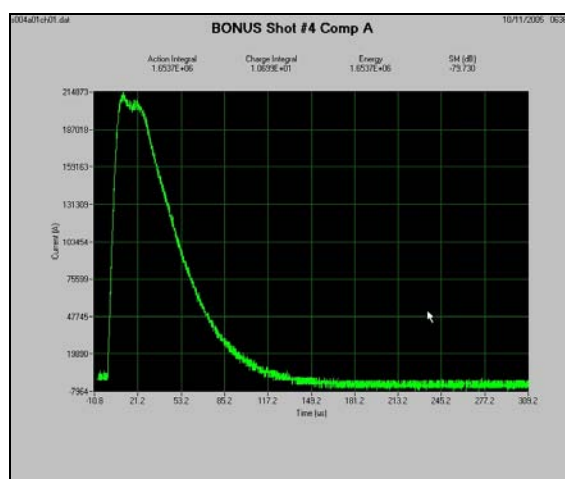
Figure N-9. Example component A Test Waveform.
