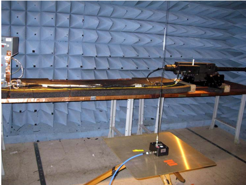
Figure K-6. Sample Emissions Set-up Photo for MIL-STD-461F.
