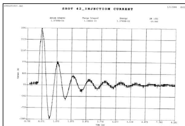
Figure E-7. Typical Injection Current Plot.
