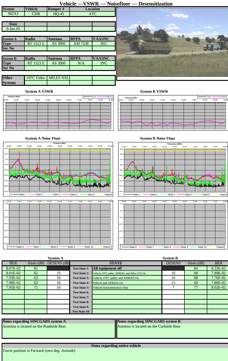
Figure A-7. Example SINGARS Desensitization Data Sheet.
