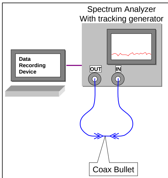
Figure A-1. Receiver Check Test Setup.
