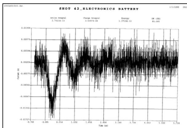
Figure E-8. Typical Battery EID Data Plot.
