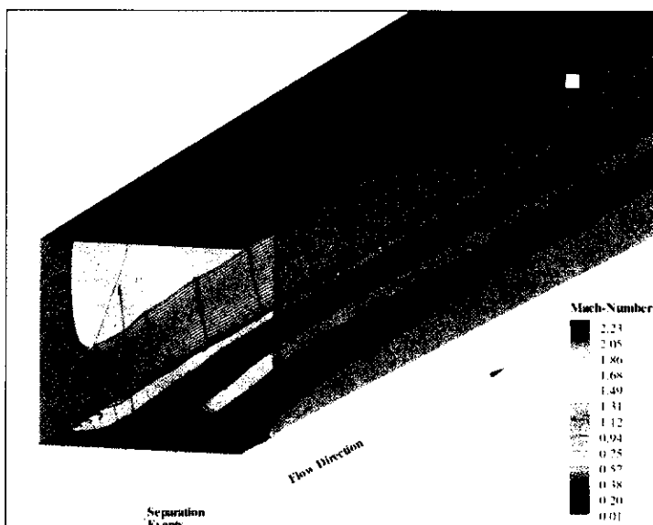
Figure 7. Mach number contours, vortex cores, and streamlines from a 3-D, reacting flow simulation of a COIL supersonic diffuser.
