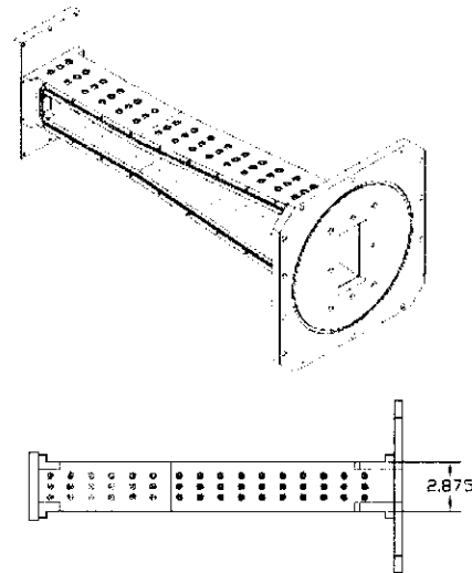
Figure 1. A schematic of the diffuser. The direction of the gas flow is from left to right.
