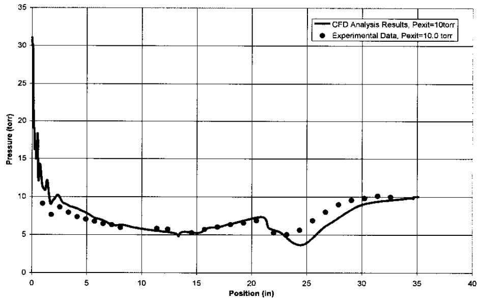
Figure 10. Baseline diffuser static pressure (centerline, top wall) versus streamwise distance from the nozzle throat (10 Torr back pressure).
