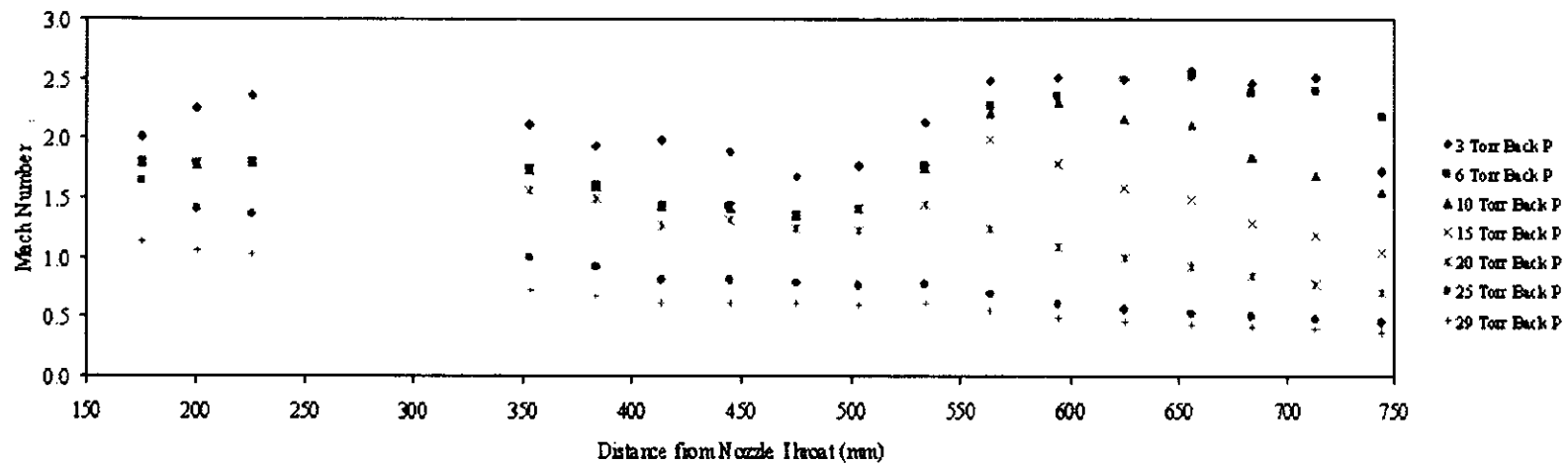
Figure 5. Mach number versus downstream distance from the nozzle throat for varying back pressure.
