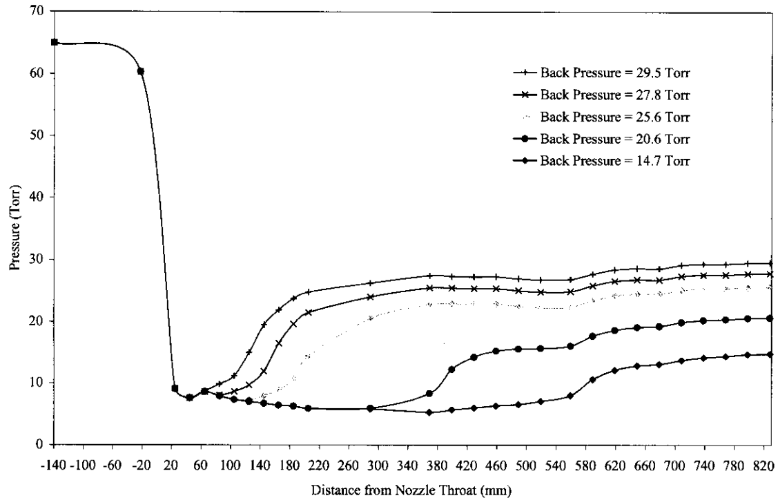
Figure 4. Static pressure versus downstream distance from the nozzle throat, with varying back pressure.
