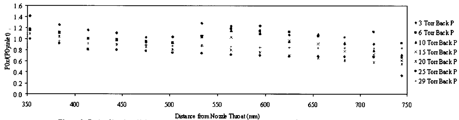
Figure 6. Ratio of local and inlet stagnation pressures versus downstream distance from the nozzle throat for varying back pressure.
