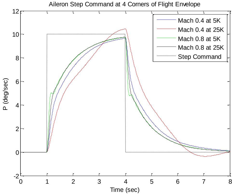
Figure 40. Disturbance Observer Aileron Step Response ( K_q = 3 )
