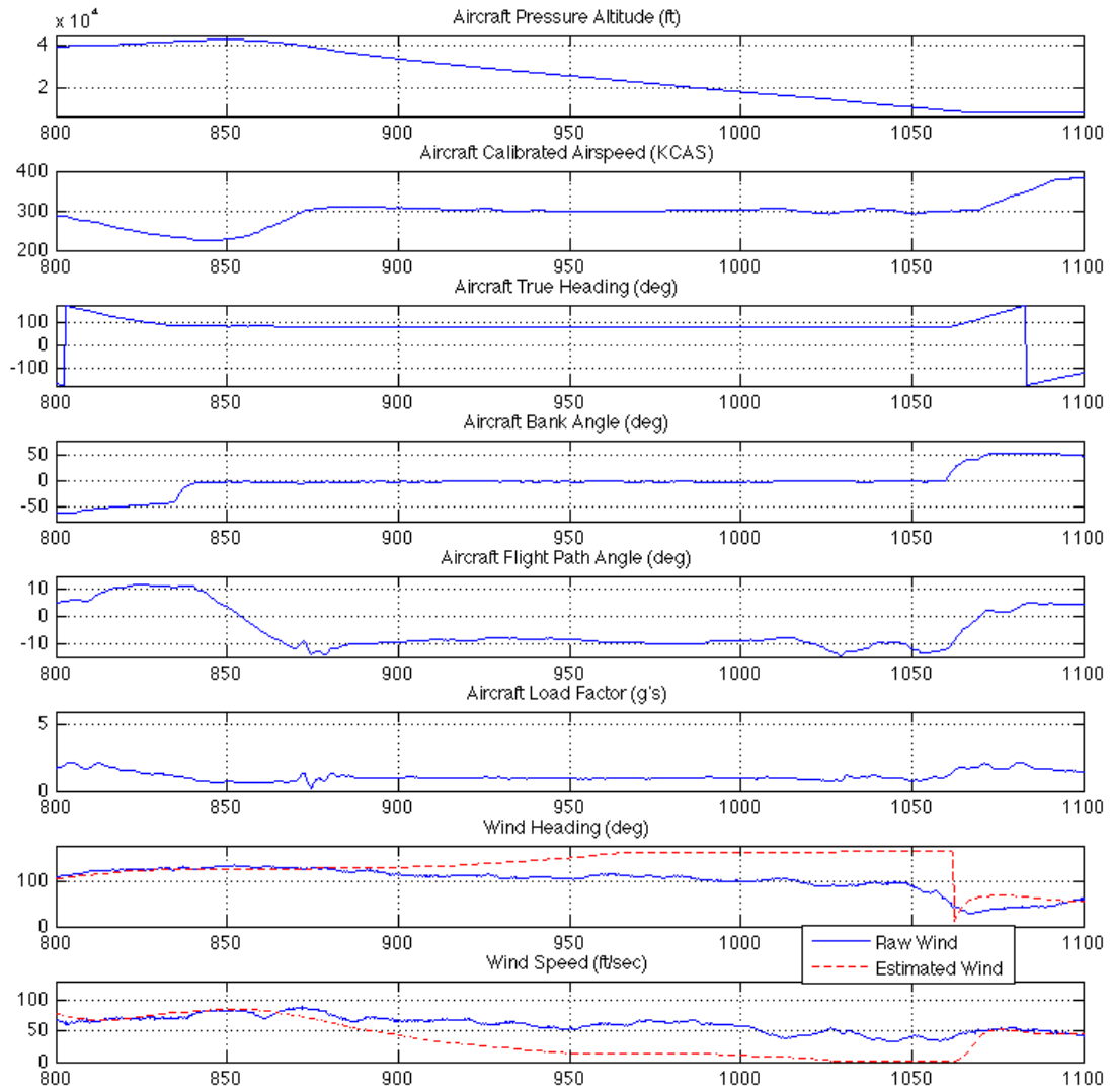
Figure 138. Penetration Descent (VEST - No Residual Logic)
