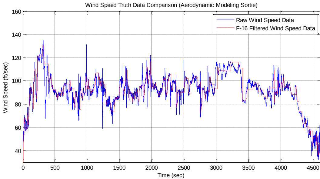
Figure 103. Aerodynamic Modeling Wind Speed Truth Data
