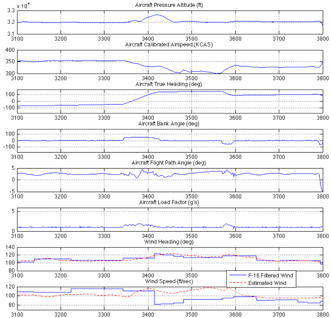
Figure 121. Cruise Points (VEST 2)
