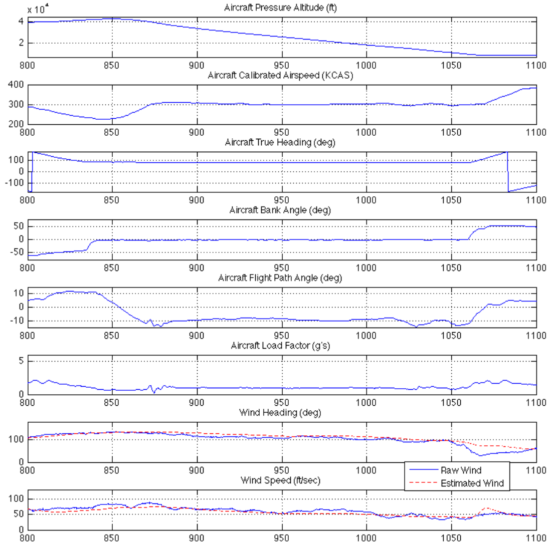
Figure 139. Penetration Descent (VEST TAS - No Residual Logic)
