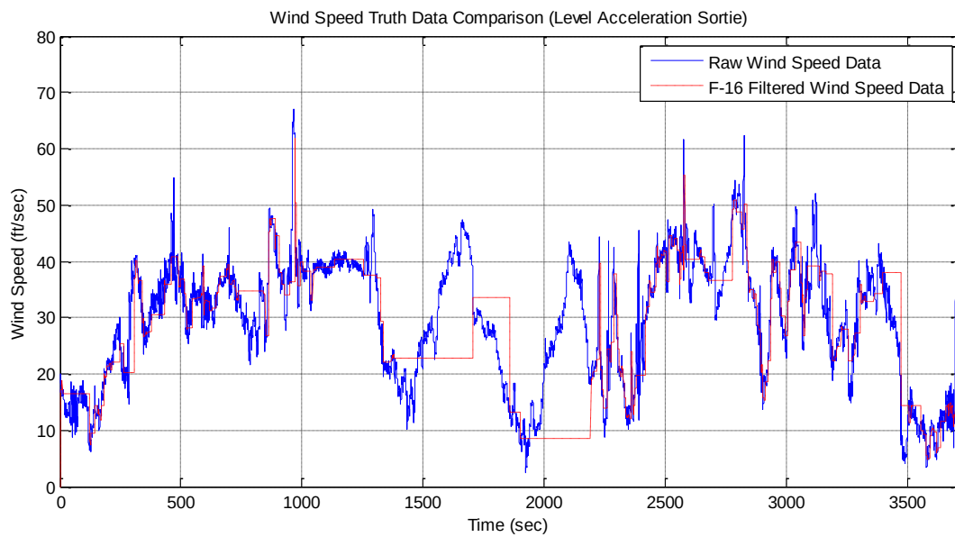
Figure 107. Level Acceleration Wind Speed Truth Data
