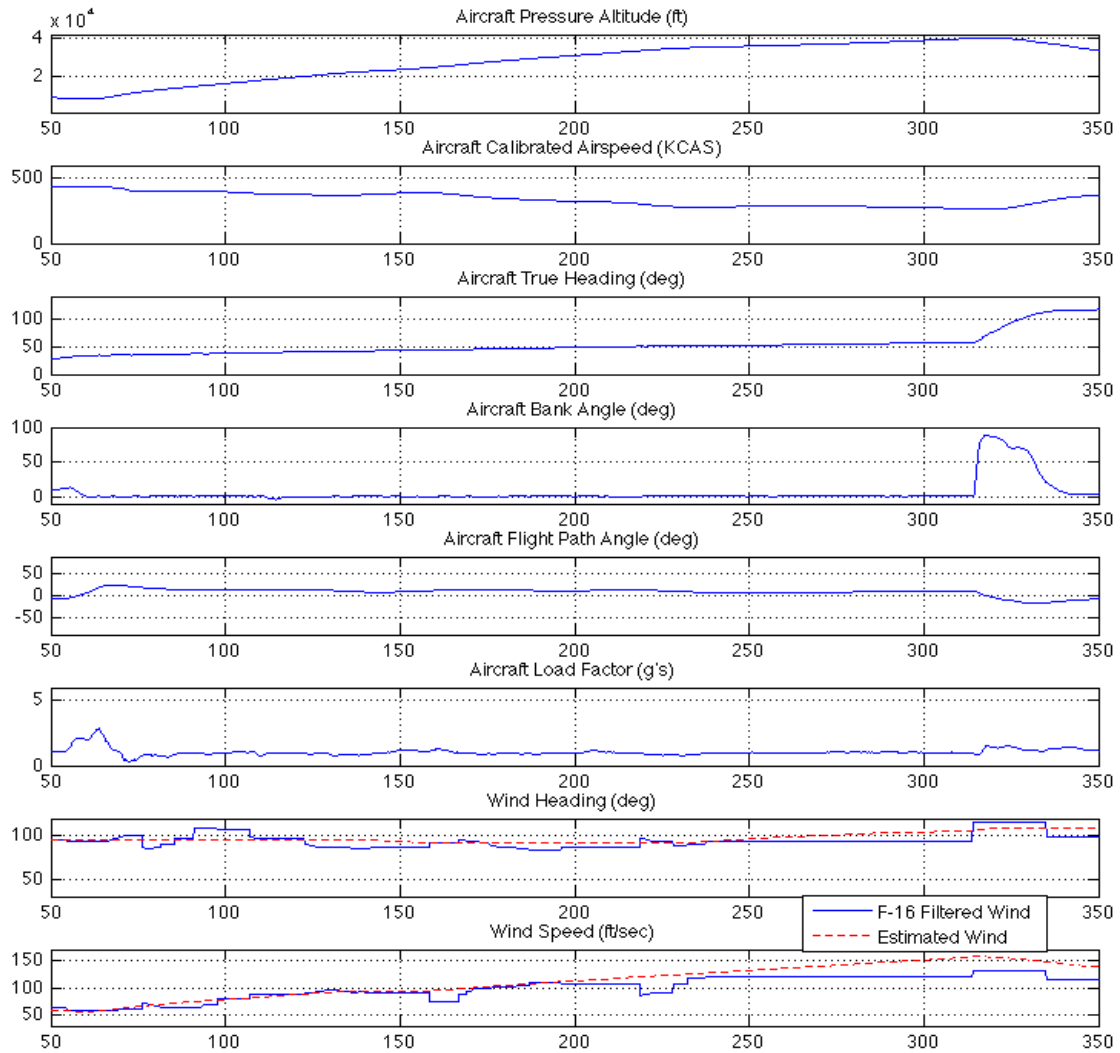
Figure 110. Bleed Rate Climb (VEST 2)
