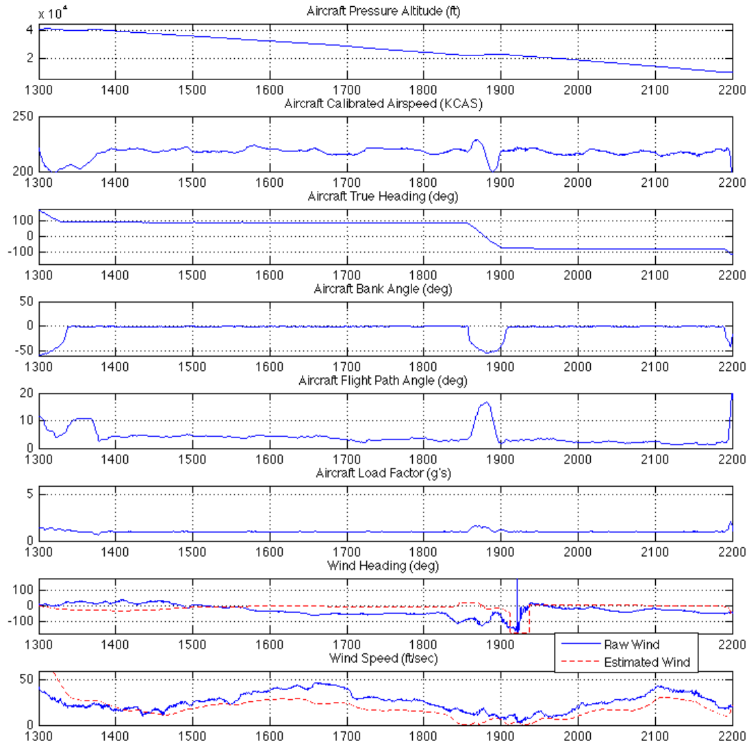
Figure 156. Maximum Range Descent (VEST)
