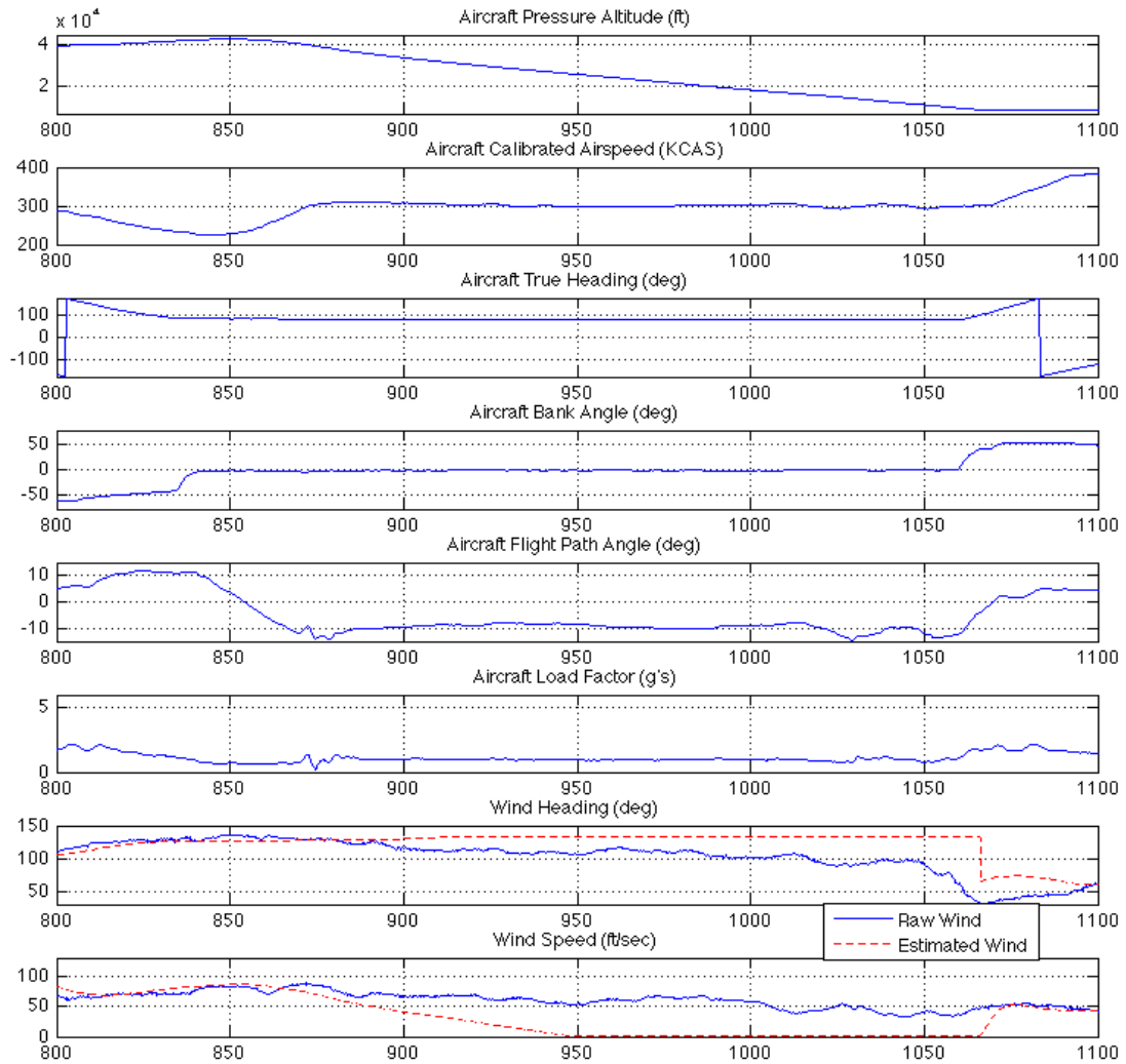
Figure 136. Penetration Descent (VEST)
