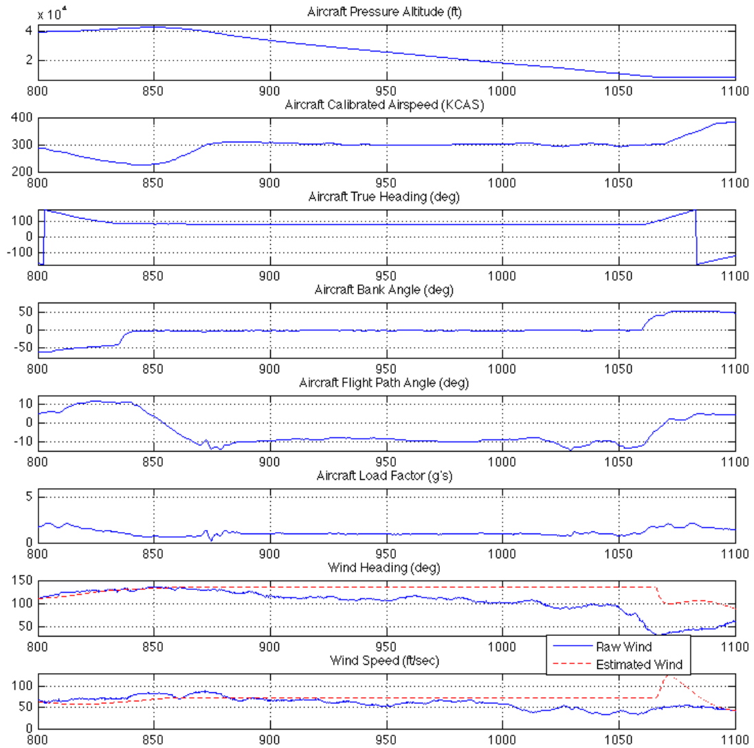
Figure 137. Penetration Descent (VEST TAS)
