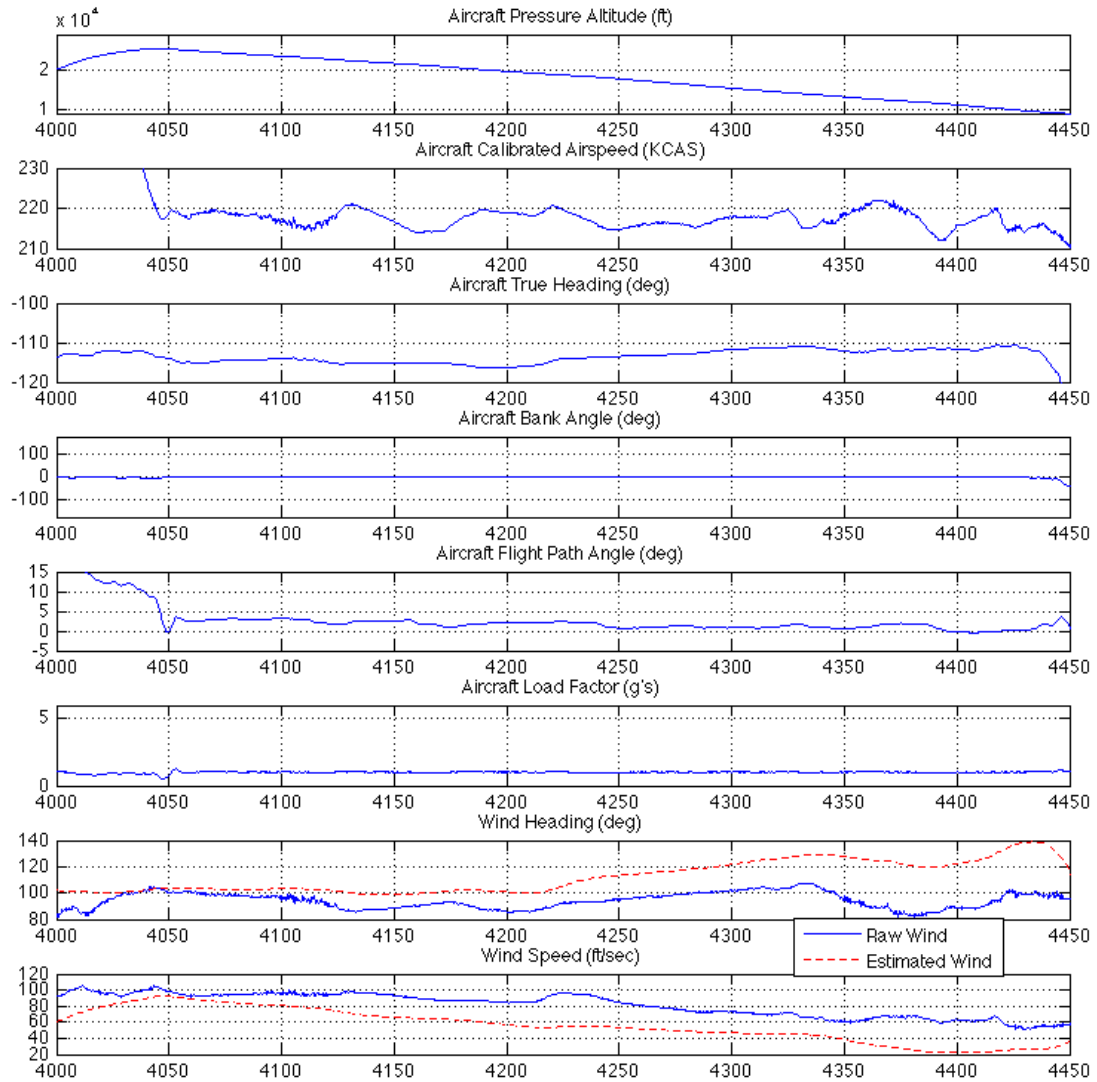
Figure 124. Maximum Range Descent (VEST)
