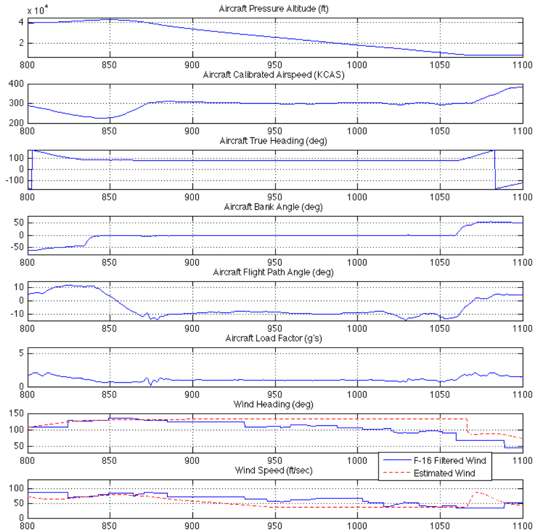
Figure 135. Penetration Descent (VEST 2)
