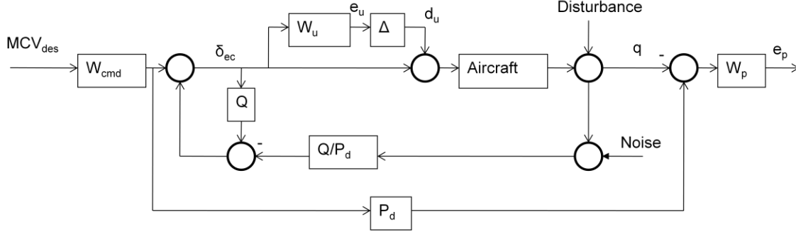
Figure 11. Pitch Axis Disturbance Observer Model and Controller
