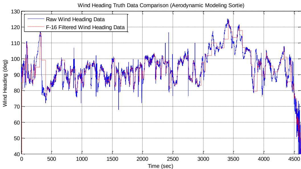
Figure 104. Aerodynamic Modeling Wind HDG Truth Data
