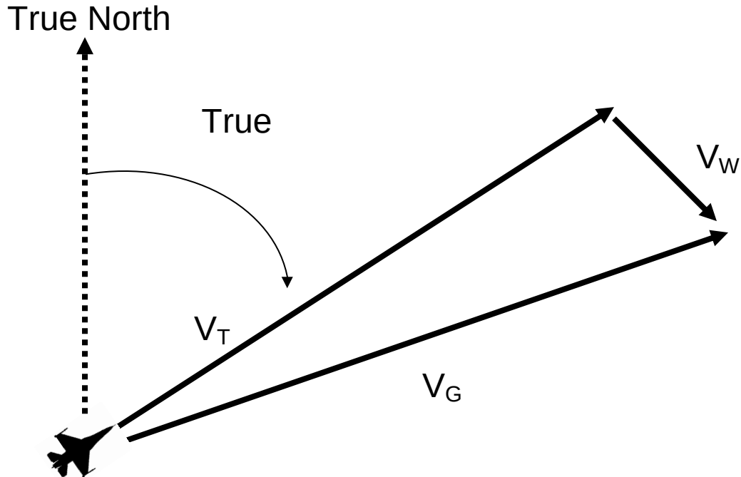
Figure 5. Velocity Triangle
