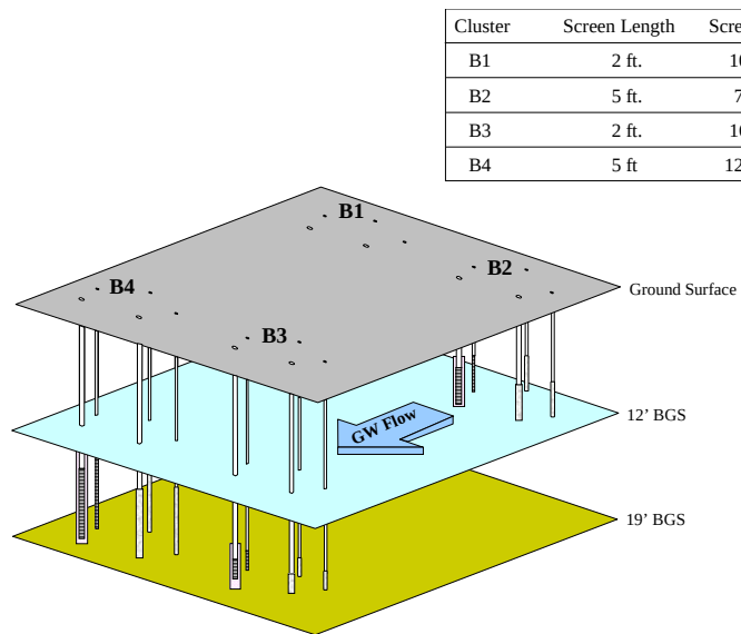
Figure 2-3. Three Dimensional Cell B Layout (Kram, 2001)
