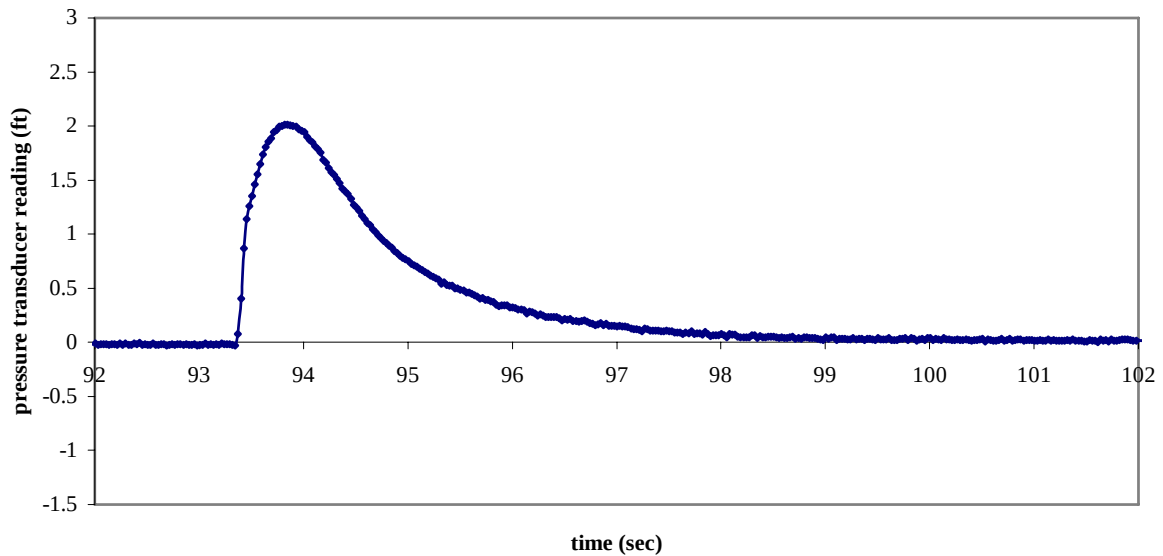
Figure 5-2. Momentary Delay in Recovery (B13 Post Development)
