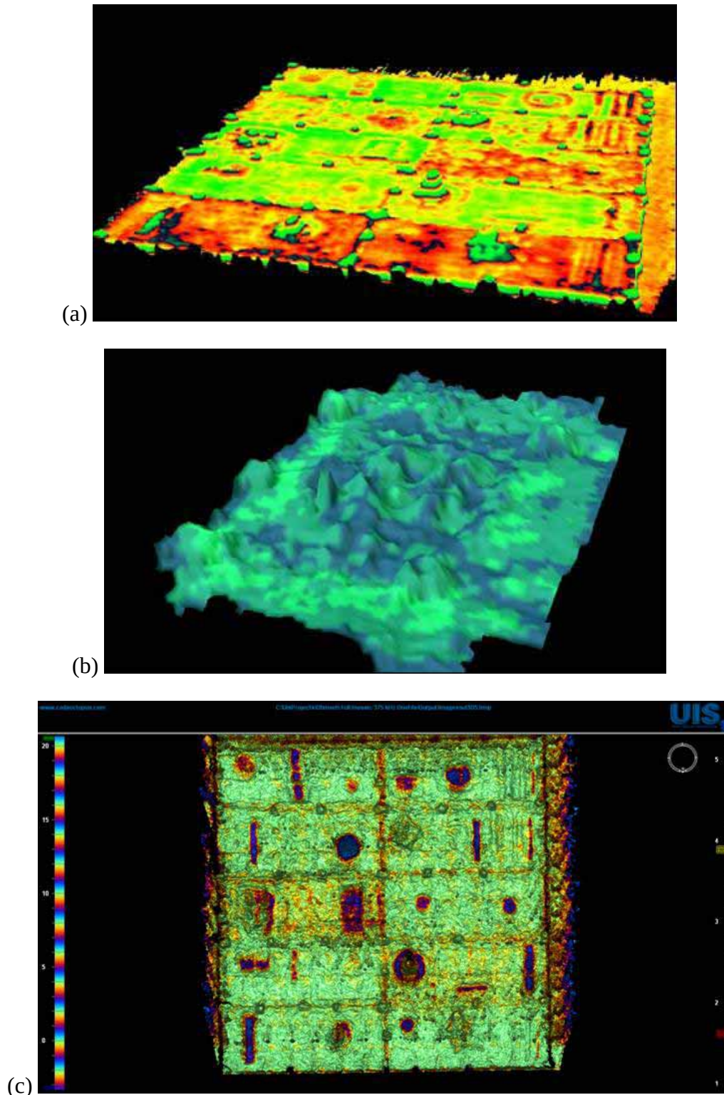
Figure 28. CodaOctopus sample results. (a) shaded mosaic showing bathymetry (color palette wraps around so red to red spans 20 cm elevation); (b) raw data of area containing oil, rock, and seaweed; and (c) data after UIS software processing (blue is oil).
