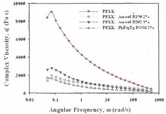
Figure 6. Complex viscosity plotted as a function of angular frequency for PEKK and nano-modified blends.
