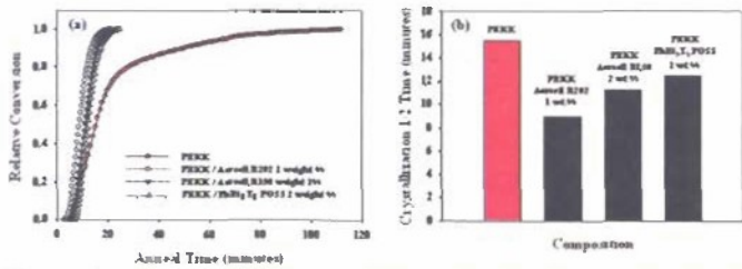
Figure 4. (a) Development of relative crystallinity of the nano-modified blends in comparison with that of the homopolymer, and (b) a comparison of their crystallization half-times. Both sets of data were measured at the lowest-measurable crystallization temperature of the subject grade of PEKK (204°C).
