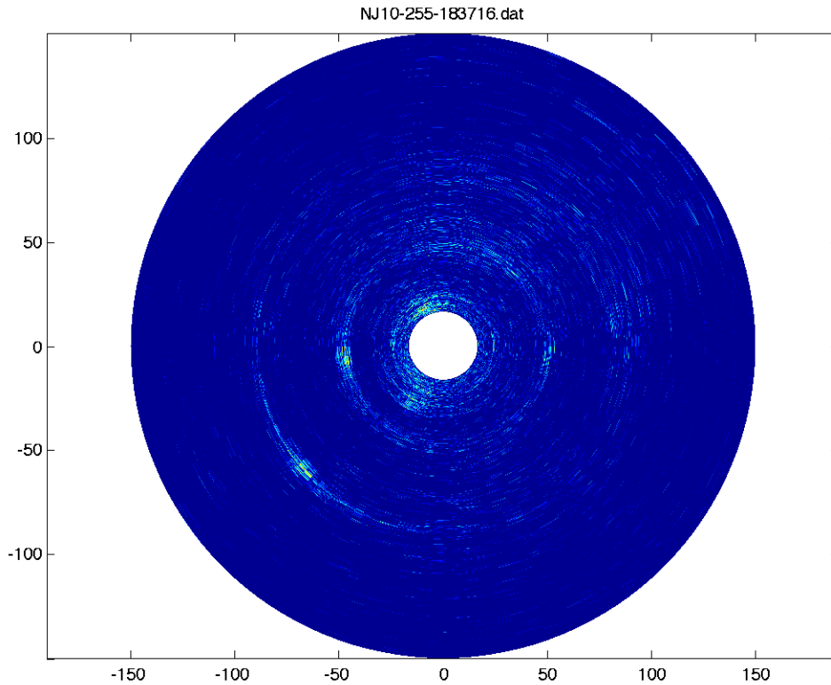
Figure 4. Image of aggregations of bay anchovies in the Chesapeake Bay. Several aggregations are shown in the backscatter image at ranges up to 100 meters from the PIMS array. The water depth was 10-20 meters. The color scale is in units of dB
