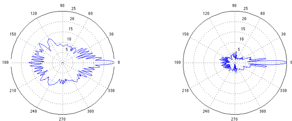
Figure 3: Two type of beamforming developed for the PIMS array. The left figure shows a fast beamforming method developed of near real-time imaging that has less resolution and higher side and back lobes. The right figure shows an improved beamforming method that can be used in postprocessing to improve image quality.
