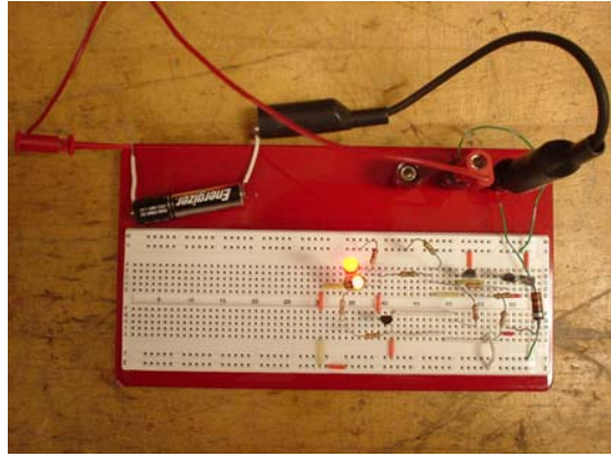
Figure 1. Breadboard of circuit simulation of low-power sensor.
