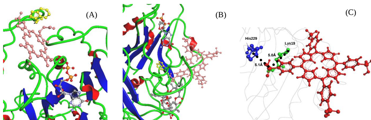
Figure 13 (A) Molecular simulations using ArgusLab show that the location of the most stable binding site for PPIX (pink) is located proximal, but not overlapped, to the nucleotide (CPK color) site and places PPIX in contact with Trp407 in the \beta -monomer (yellow). (B) The site of TSPP (pink) places it between the location of GTP and taxol (both in CPK colors) and at \sim 8 Å from Trp21 in the \beta -monomer (yellow). In both (A) and (B) the indole ring is nearly perpendicular to the porphyrin ring. (C) One of the SO 3 - groups of TSPP (red) is in proximity and equidistant with Lys19 (green) and His229 (blue)
