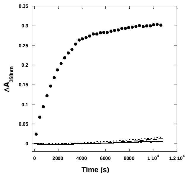
Figure 12 Polymerization of tubulin. The figure shows that under the condition of buffer and temperature of the fluorescence experiments, 5 \mu M tubulin alone (—●—) as well as in the presence of 2.5 \mu M PPIX (•••) or 2.5 \mu M TSPP (— — —) does not polymerize. Under the same conditions the presence of 2.5 \mu M taxol (●) does instead induce polymerization
