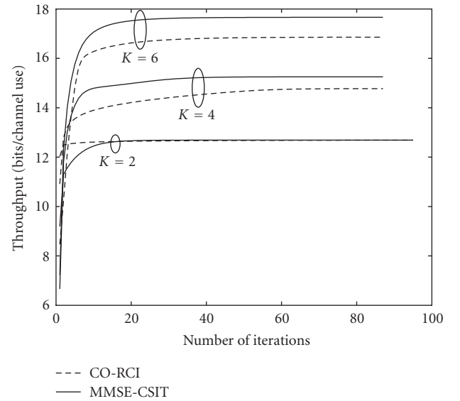
FIGURE 4: Convergence of CO-RCI and MMSE-CSIT beamforming algorithms for N_t = 4 , N_r = 4 , P = 10 , and different number of users for a channel realization from the measured data.
