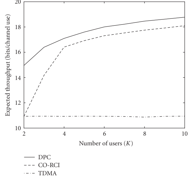
FIGURE 1: Expected throughput versus number of users for fixed N_r = N_t = 4 antennas and P = 10 in Rayleigh, flat-fading channel model. All nodes have perfect channel knowledge for all realizations of the channel.
