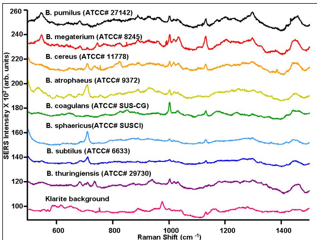
Figure 12. Comparison of SERS spectra from several Bacillus spore samples collected on Klarite substrates collected on Renishaw system.
