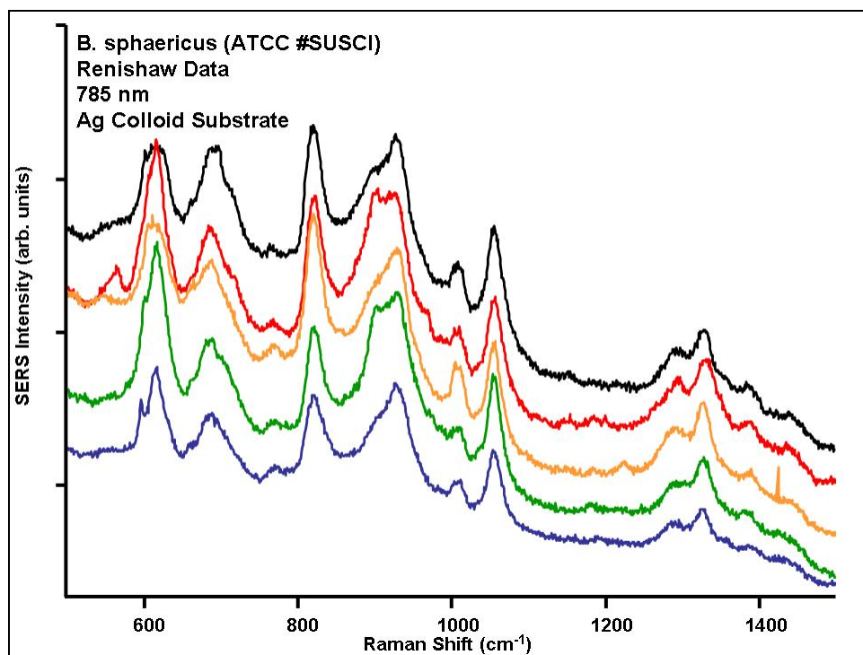
Figure B-33. Example SERS spectra of B. sphaericus collected using Ag colloids on Renishaw system using 785 nm laser.
