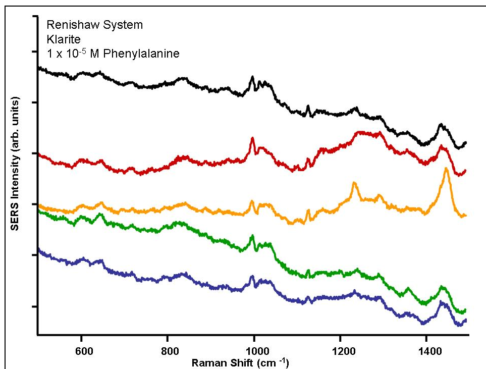
Figure C-24. SERS of 1 \times 10^{-5} M PHE as measured on Klarite substrate with the Renishaw system.
