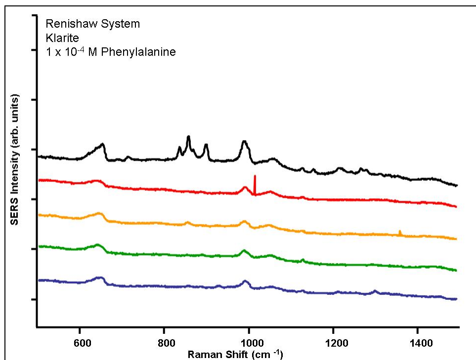
Figure C-23. SERS of 1 \times 10^{-4} M PHE as measured on Klarite substrate with the Renishaw system.
