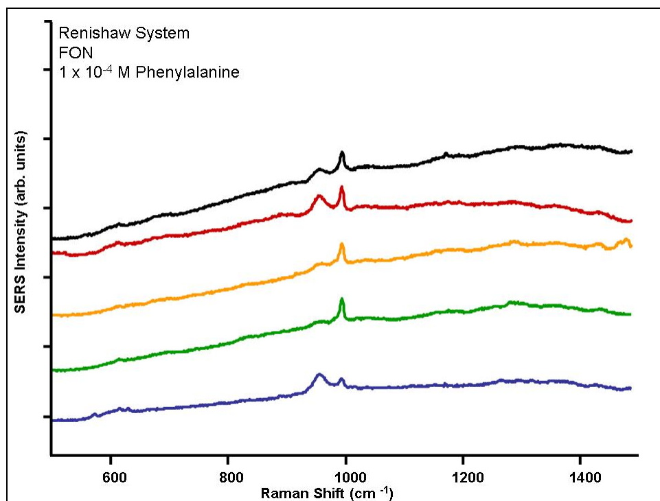
Figure C-15. SERS of 0.0001 M PHE as measured with FON substrate with the Renishaw system.
