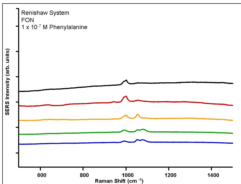
Figure C-18. SERS of 1 x 10 -7 M PHE as measured with FON substrate with the Renishaw system.
