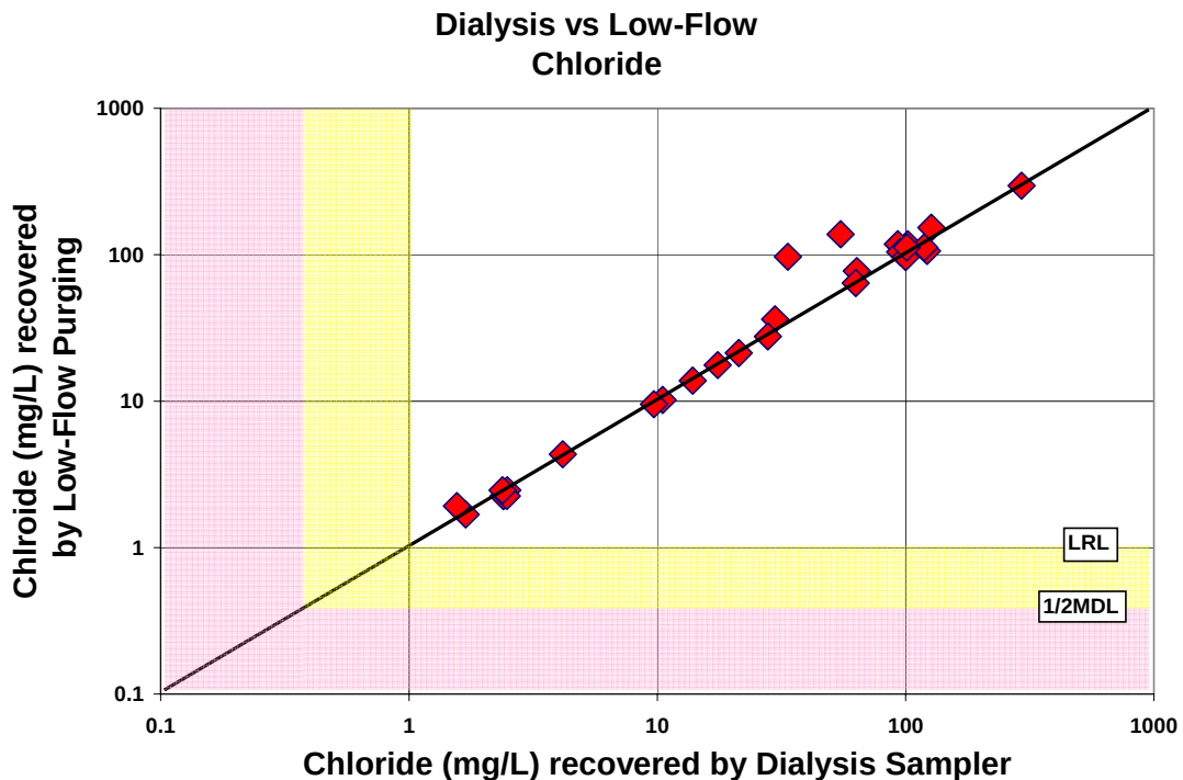
Figure 5-2. Example of a 1:1 Correspondence Plot of Dialysis Sampler vs. Low-Flow Purging Results for Chloride (from Imbrigiotta et al., 2007) (LRL, lower reporting limit; 1/2MDL, one half minimum detection limit; mg/L, milligrams per liter)
