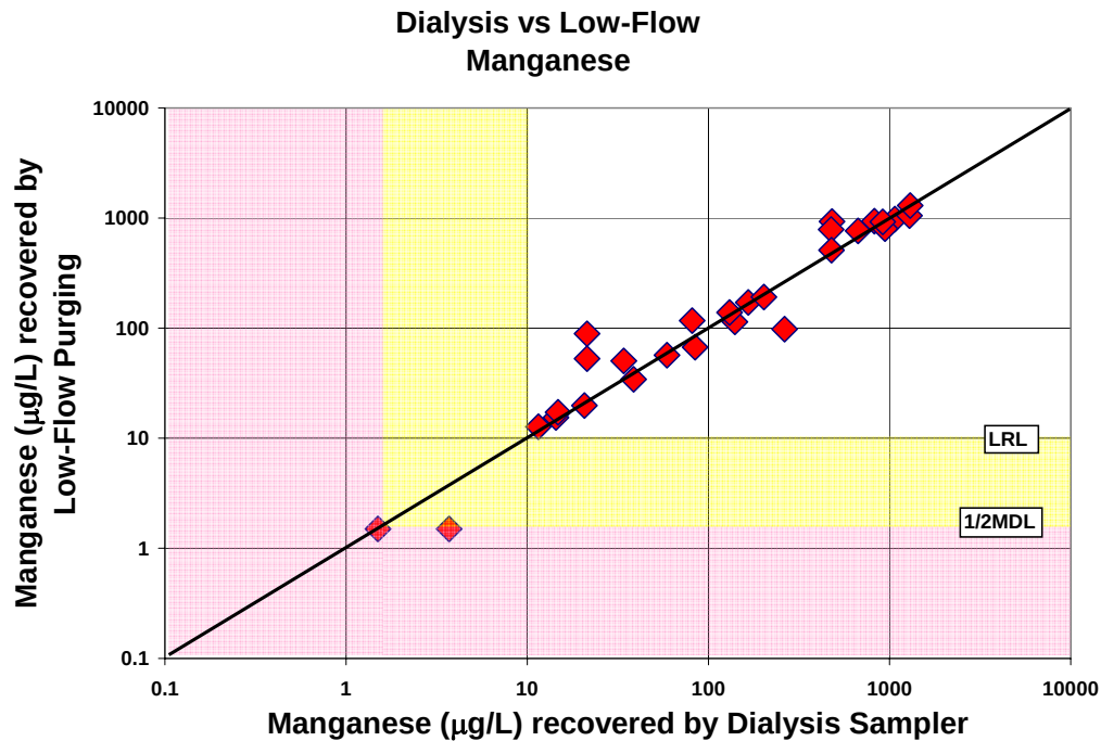
Figure 5-1. Example of a 1:1 Correspondence Plot of Dialysis Sampler vs. Low-Flow Purging Results for Manganese (from Imbrigiotta et al., 2007) (LRL, lower reporting limit; 1/2MDL, one half minimum detection limit; \mu\text{g/L} , micrograms per liter)
