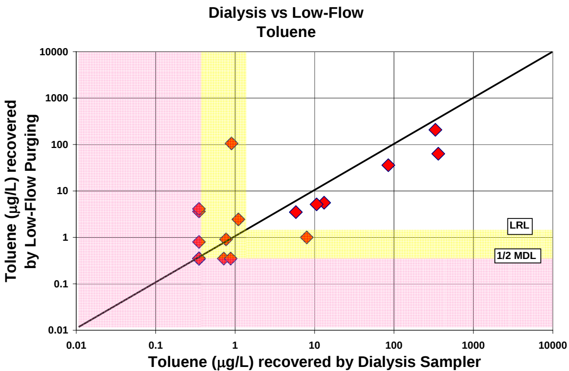
Figure A-44. Comparison of toluene concentrations recovered by the dialysis sampler and low-flow purging.
