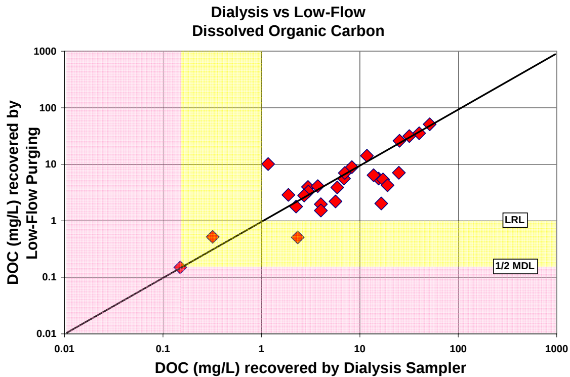
Figure A-78. Comparison of dissolved organic carbon (DOC) concentrations recovered by the dialysis sampler and low-flow purging
