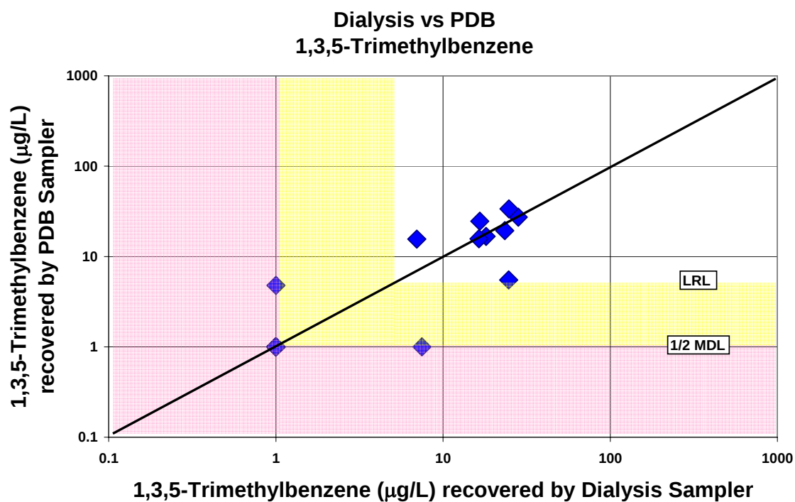
Figure A-7. Comparison of 1,3,5-trimethylbenzene concentrations recovered by the dialysis sampler and the polyethylene diffusion bag (PDB) sampler
