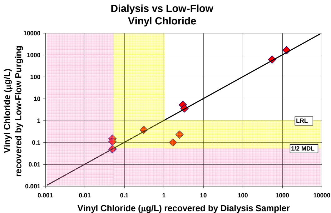
Figure 4-2. Dialysis Sampler Versus Low-Flow Purging Results For Vinyl Chloride.
