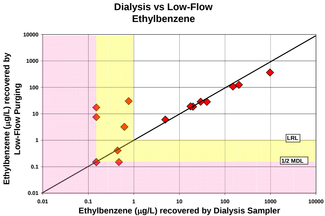
Figure A-18. Comparison of ethylbenzene concentrations recovered by the dialysis sampler and low-flow purging
