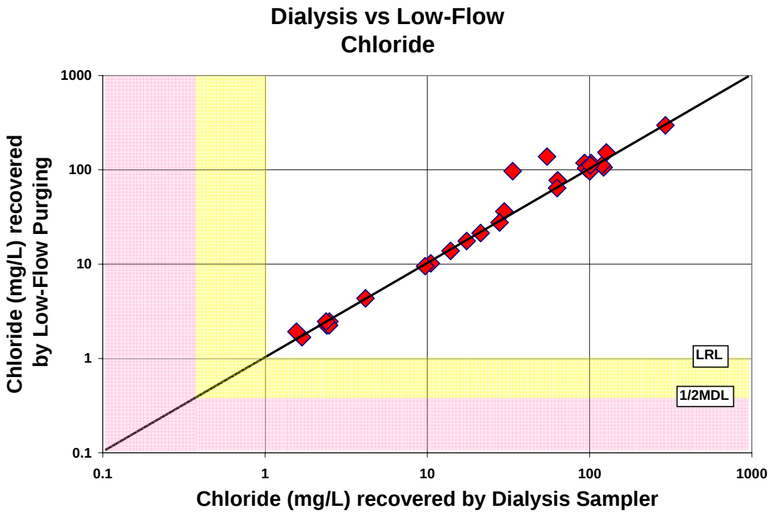
Figure A-55. Comparison of chloride concentrations recovered by the dialysis sampler and low-flow purging
