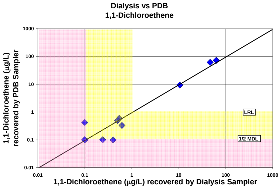
Figure A-3. Comparison of 1,1-dichloroethene concentrations recovered by the dialysis sampler and the polyethylene diffusion bag (PDB) sampler
