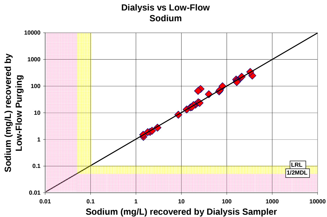
Figure A-52. Comparison of sodium concentrations recovered by the dialysis sampler and low-flow purging
