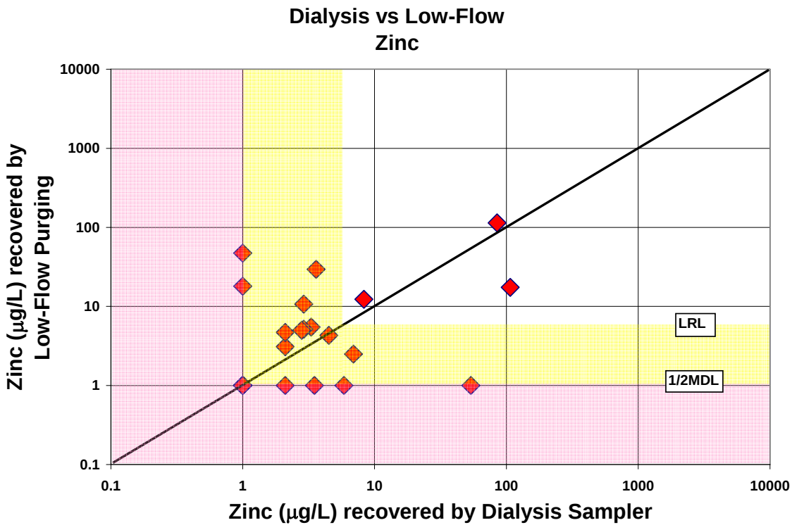
Figure A-73. Comparison of zinc concentrations recovered by the dialysis sampler and low-flow purging
