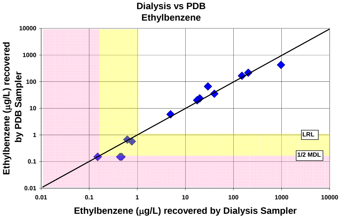
Figure 4-3. Dialysis Sampler Versus Polyethylene Diffusion Bag (PDB) Sampler Results For Ethylbenzene
