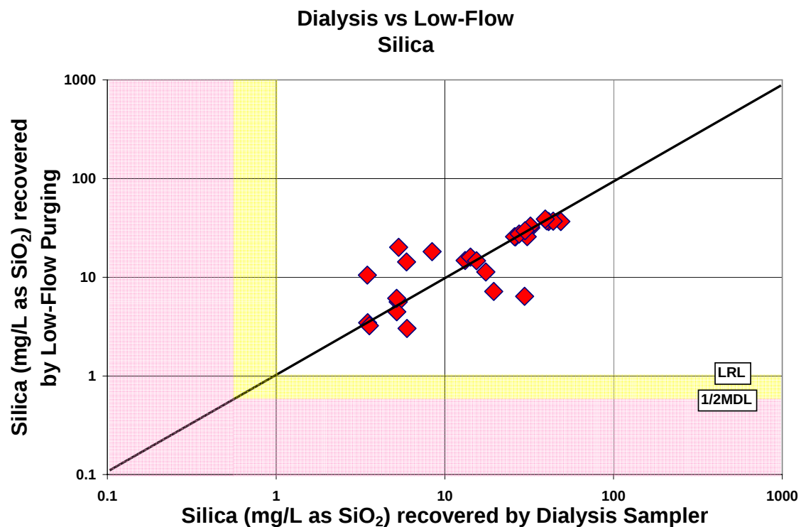
Figure A-60. Comparison of silica concentrations recovered by the dialysis sampler and low-flow purging
