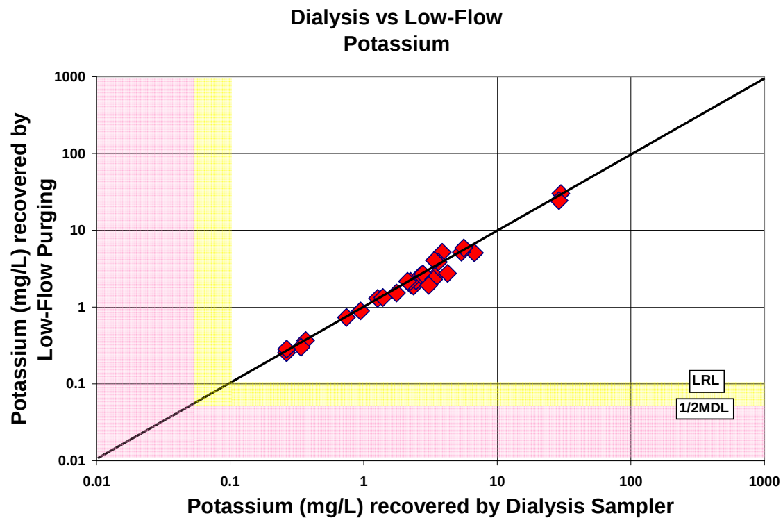
Figure A-53. Comparison of potassium concentrations recovered by the dialysis sampler and low-flow purging
