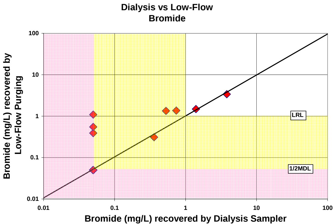
Figure A-58. Comparison of bromide concentrations recovered by the dialysis sampler and low-flow purging
