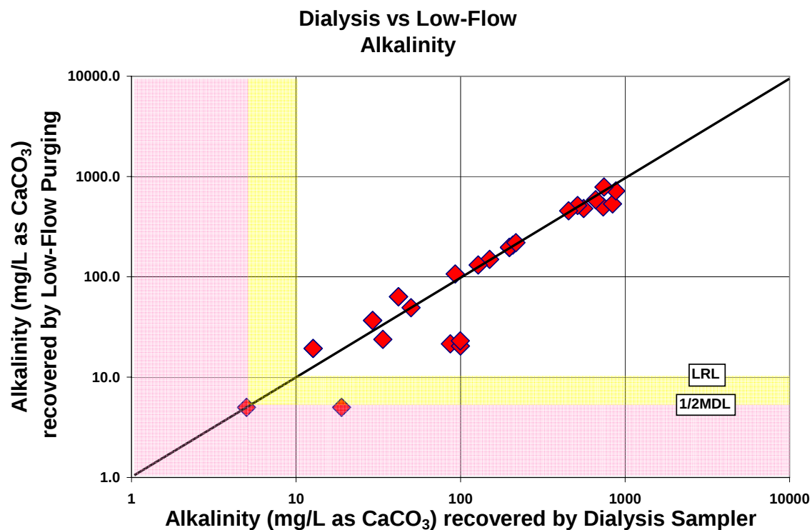
Figure A-54. Comparison of alkalinity (bicarbonate) concentrations recovered by the dialysis sampler and low-flow purging
