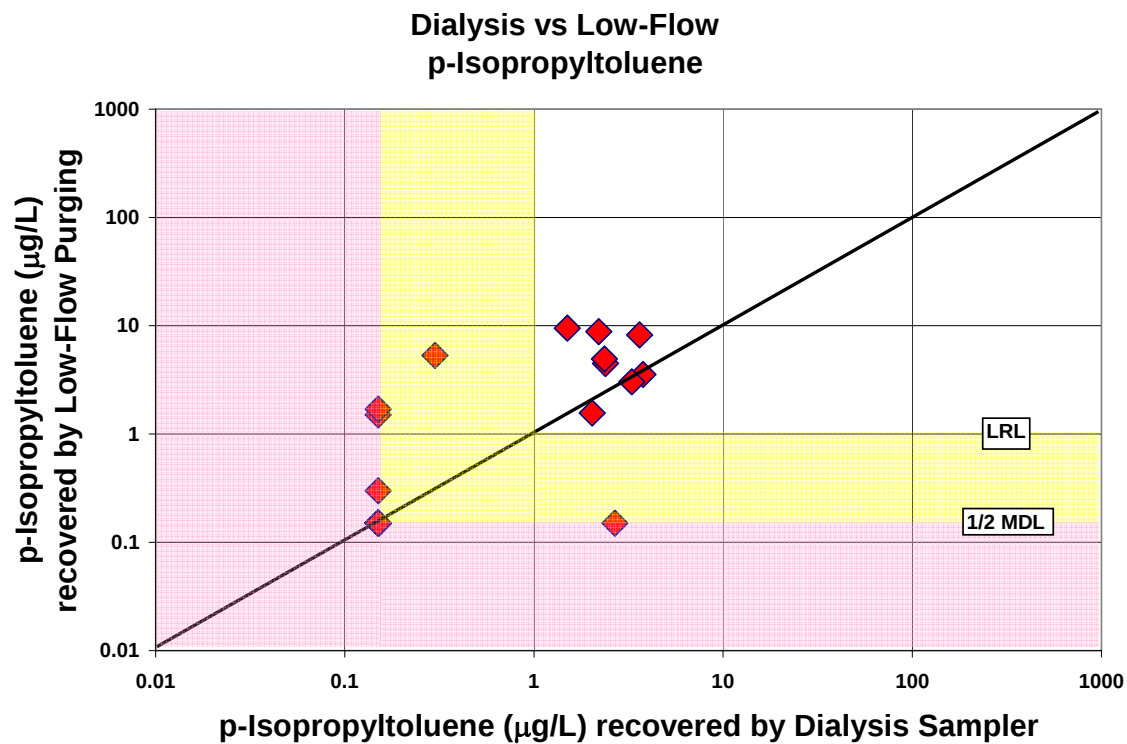
Figure A-34. Comparison of p-isopropyltoluene concentrations recovered by the dialysis sampler and low-flow purging
