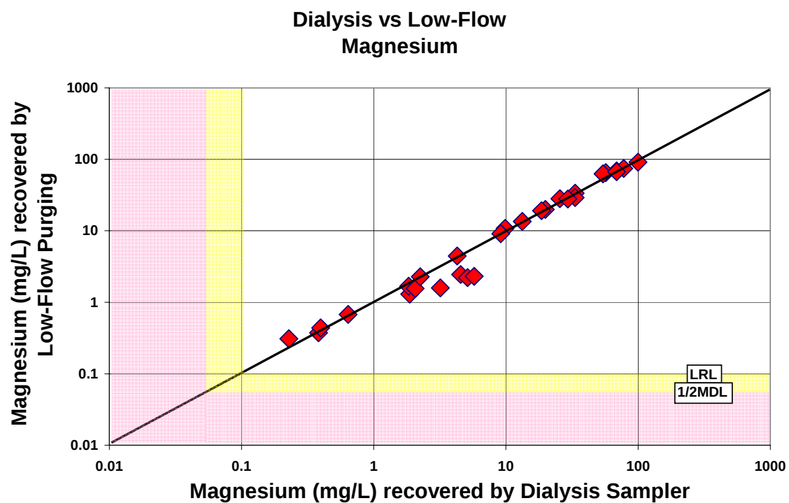
Figure A-51. Comparison of magnesium concentrations recovered by the dialysis sampler and low-flow purging
