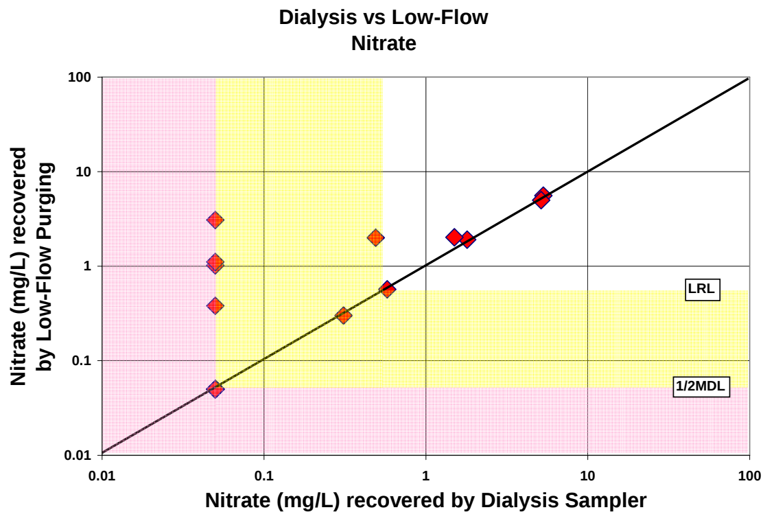
Figure A-59. Comparison of nitrate concentrations recovered by the dialysis sampler and low-flow purging
