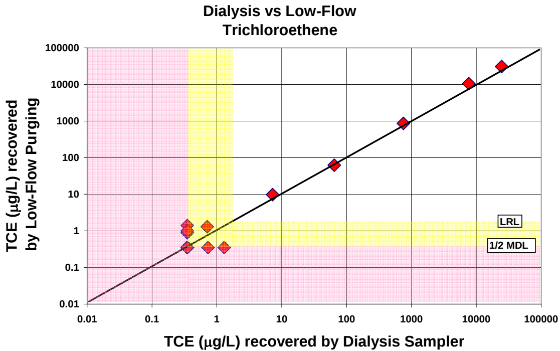
Figure A-42. Comparison of trichloroethene concentrations recovered by the dialysis sampler and low-flow purging
