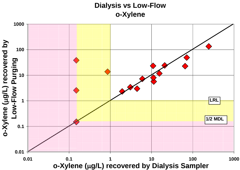
Figure A-32. Comparison of o-xylene concentrations recovered by the dialysis sampler and low-flow purging
