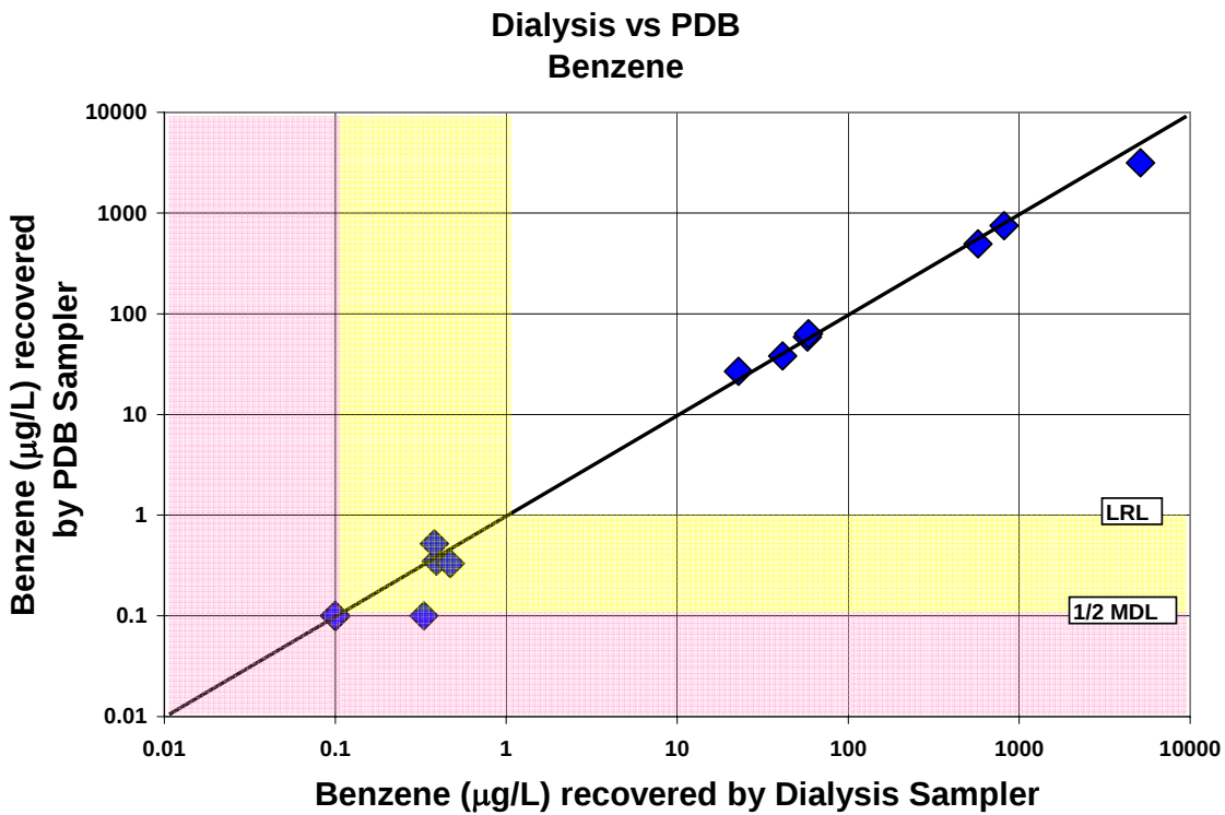
Figure A-9. Comparison of benzene concentrations recovered by the dialysis sampler and the polyethylene diffusion bag (PDB) sampler
