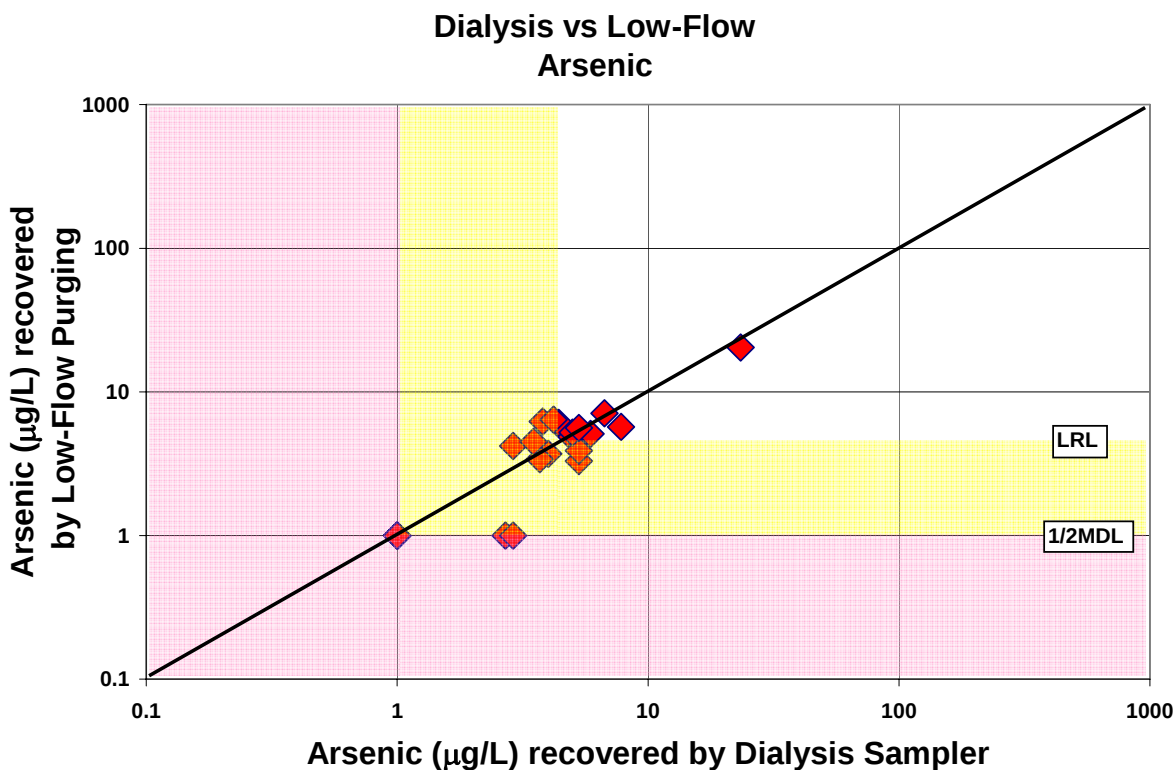
Figure 4-11. Dialysis Sampler Versus Low-Flow Purging Results For Arsenic
