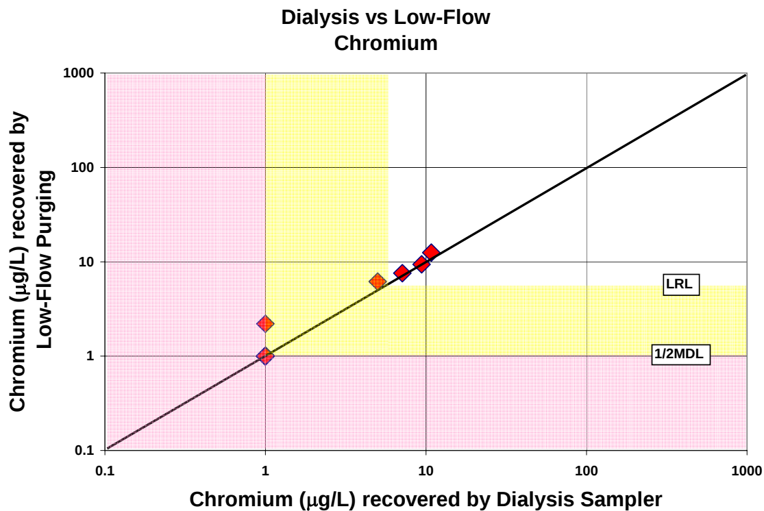
Figure A-65. Comparison of chromium concentrations recovered by the dialysis sampler and low-flow purging
