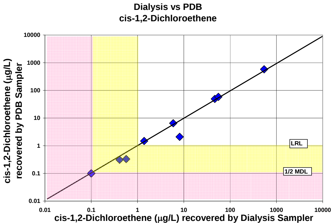
Figure A-11. Comparison of cis-1,2-dichloroethene concentrations recovered by the dialysis sampler and the polyethylene diffusion bag (PDB) sampler
