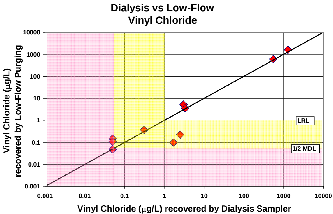
Figure A-48. Comparison of vinyl chloride concentrations recovered by the dialysis sampler and low-flow purging
