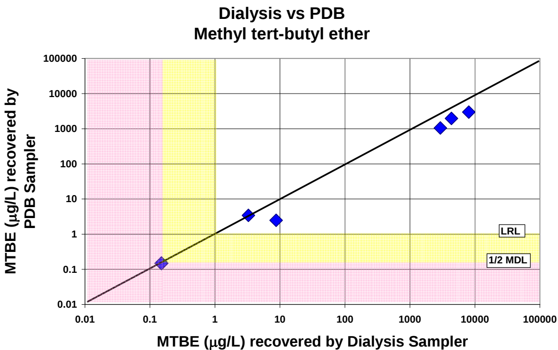
Figure 4-5. Dialysis Sampler Versus Polyethylene Diffusion Bag (PDB) Sampler Results For Methyl Tert-Butyl Ether
