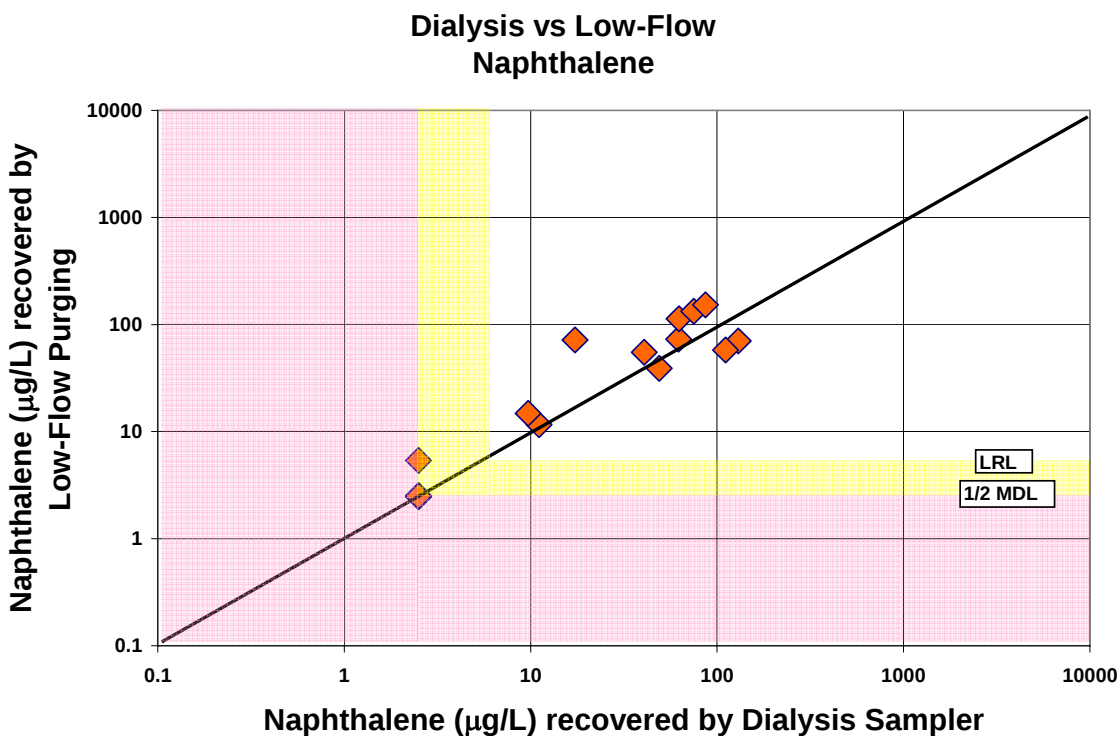
Figure A-26. Comparison of naphthalene concentrations recovered by the dialysis sampler and low-flow purging
