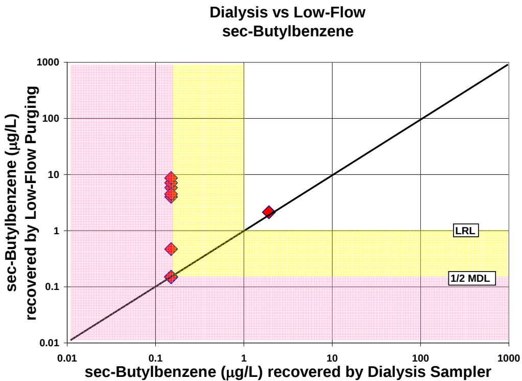
Figure A-36. Comparison of sec-butylbenzene concentrations recovered by the dialysis sampler and low-flow purging
