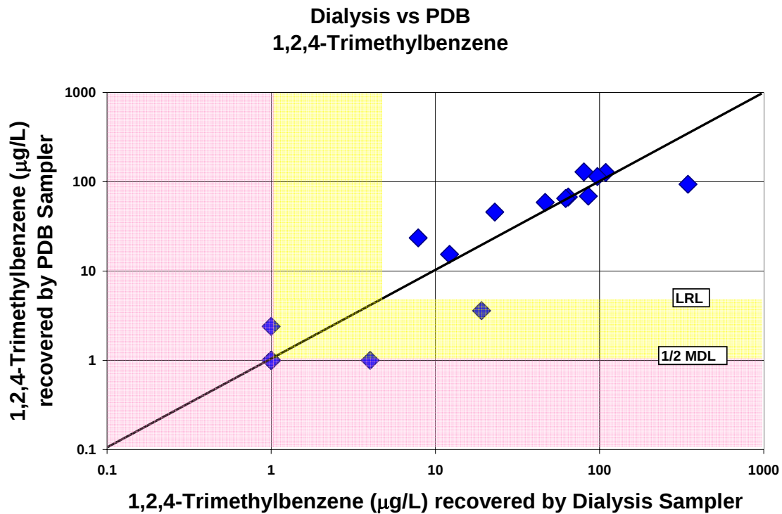
Figure A-5. Comparison of 1,2,4-trimethylbenzene concentrations recovered by the dialysis sampler and the polyethylene diffusion bag (PDB) sampler
