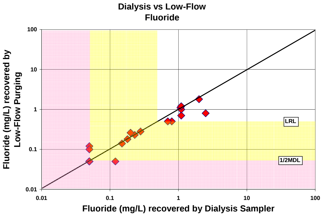
Figure A-57. Comparison of fluoride concentrations recovered by the dialysis sampler and low-flow purging
