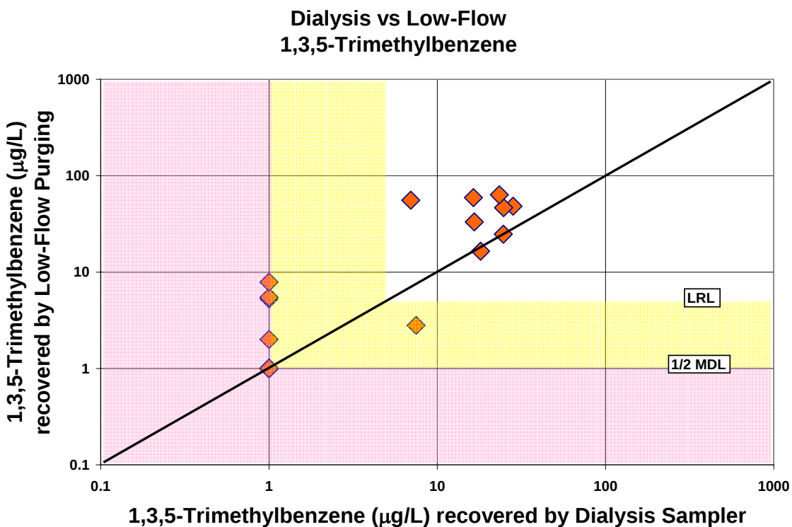
Figure A-8. Comparison of 1,3,5-trimethylbenzene concentrations recovered by the dialysis sampler and low-flow purging
