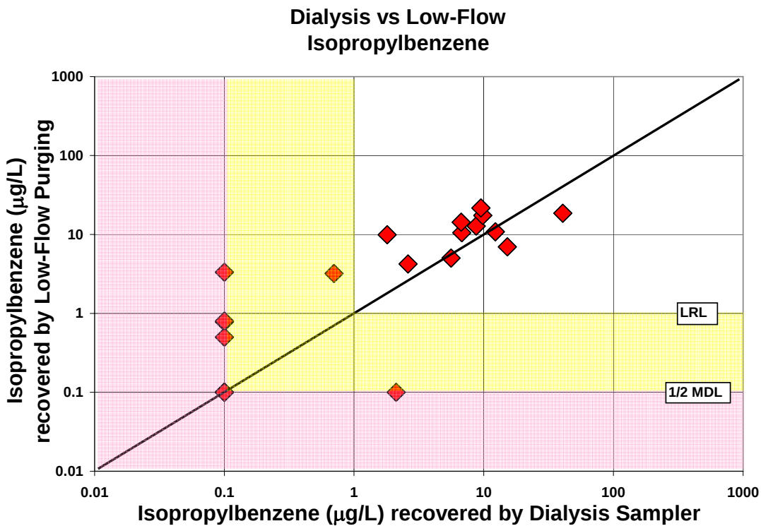
Figure A-20. Comparison of isopropylbenzene concentrations recovered by the dialysis sampler and low-flow purging
