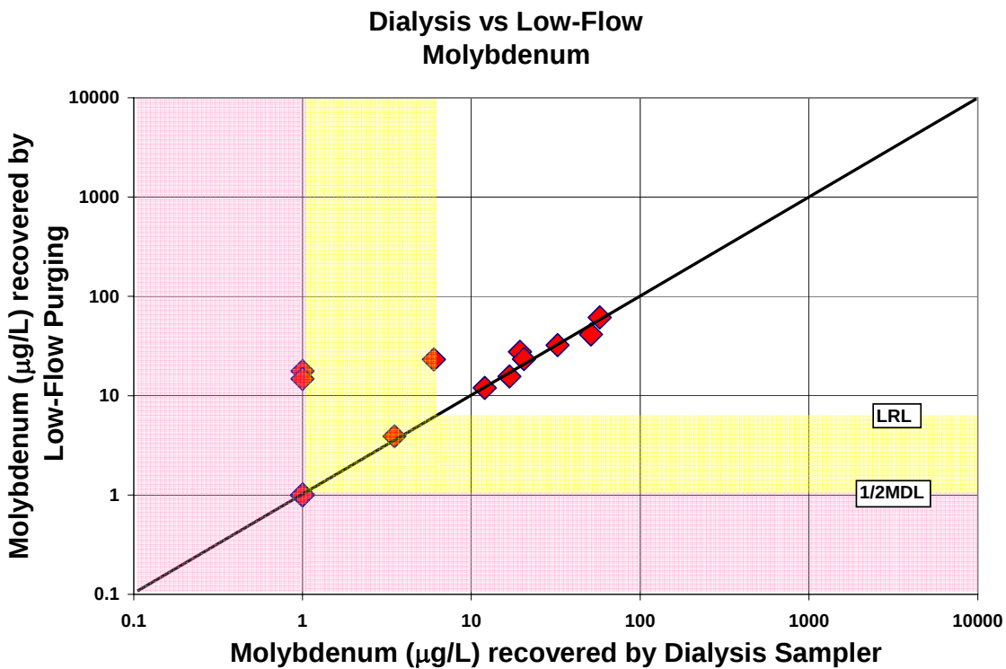
Figure A-68. Comparison of molybdenum concentrations recovered by the dialysis sampler and low-flow purging
