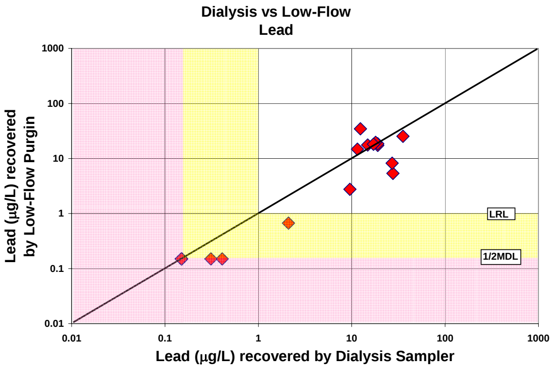
Figure A-70. Comparison of lead concentrations recovered by the dialysis sampler and low-flow purging
