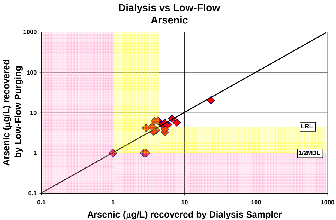
Figure A-62. Comparing of arsenic concentrations recovered by the dialysis sampler and low-flow purging
