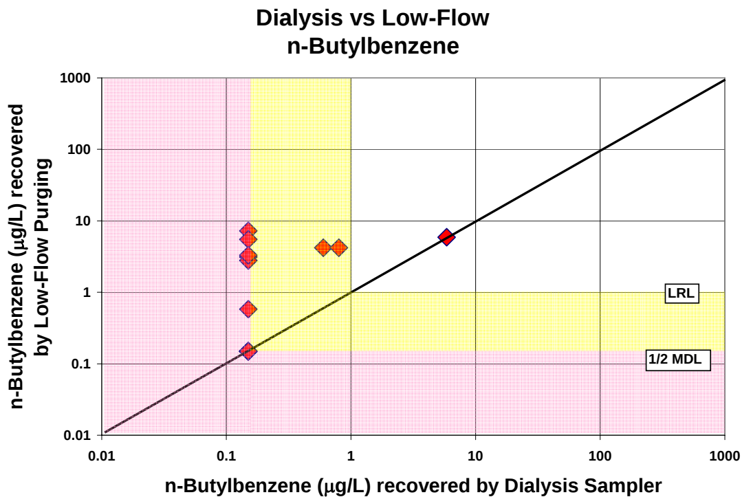
Figure A-28. Comparison of n-butylbenzene concentrations recovered by the dialysis sampler and low-flow purging
