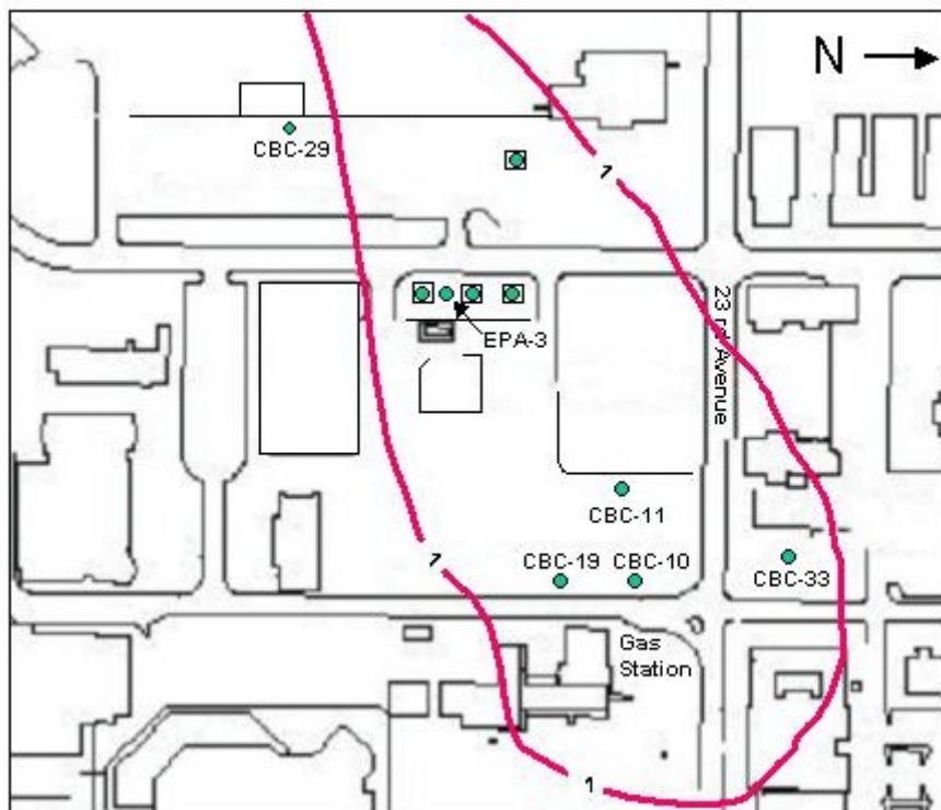
Figure 3-3. Wells Sampled As Part Of The Field Demonstration At Naval Base Ventura County, Port Hueneme, California
