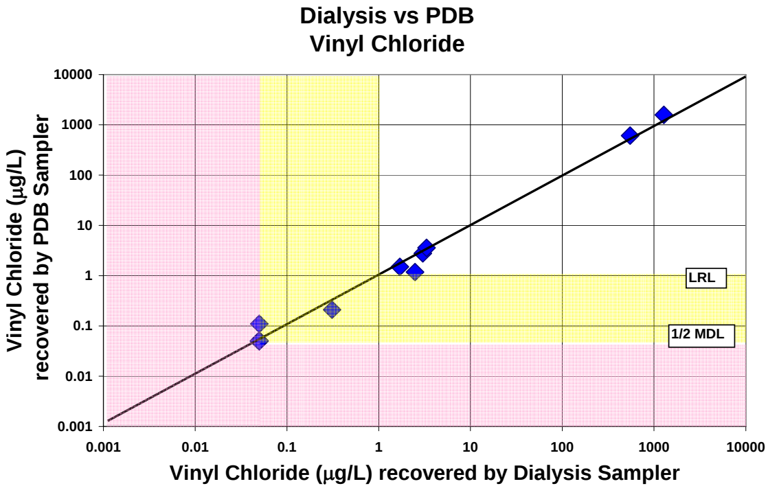
Figure A-47. Comparison of vinyl chloride concentrations recovered by the dialysis sampler and the polyethylene diffusion bag (PDB) sampler
