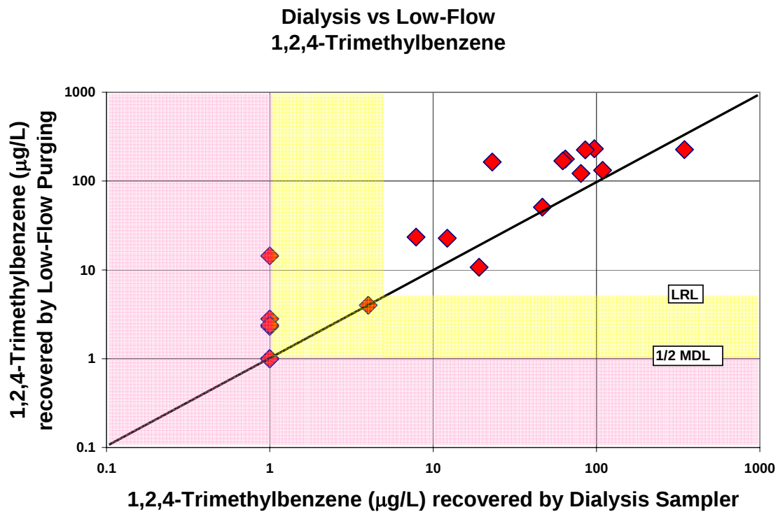
Figure A-6. Comparison of 1,2,4-trimethylbenzene concentrations recovered by the dialysis sampler and low-flow purging
