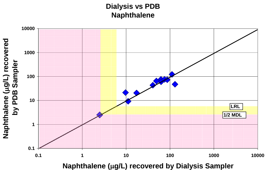
Figure A-25. Comparison of naphthalene concentrations recovered by the dialysis sampler and the polyethylene diffusion bag (PDB) sampler
