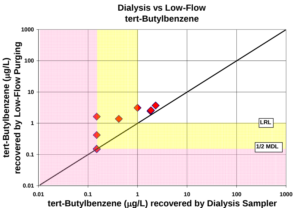
Figure A-40. Comparison of tert-butylbenzene concentrations recovered by the dialysis sampler and low-flow purging
