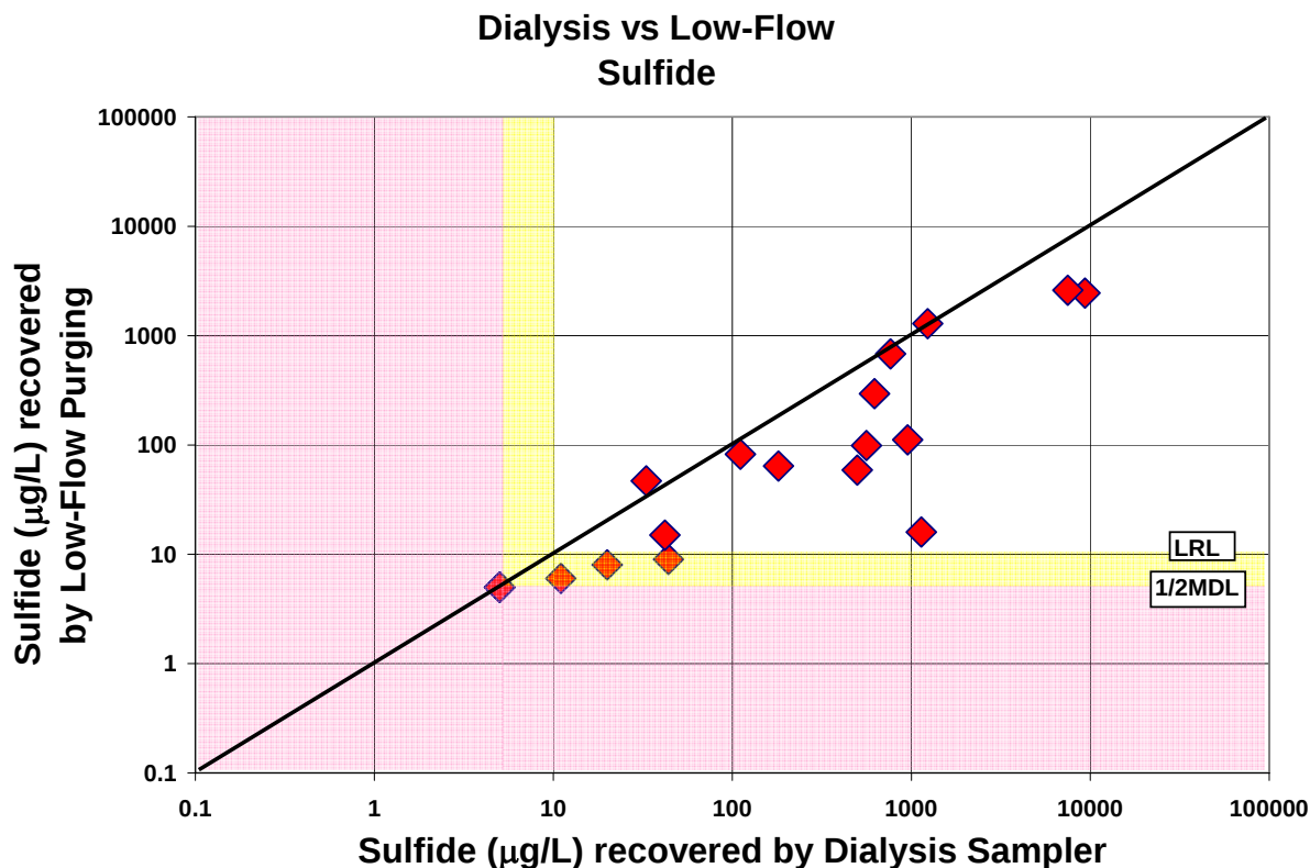
Figure 4-14. Dialysis Sampler Versus Low-Flow Purging Results For Sulfide
