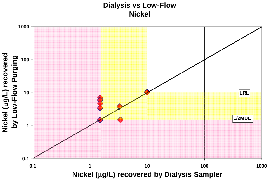
Figure A-69. Comparison of nickel concentrations recovered by the dialysis sampler and low-flow purging
