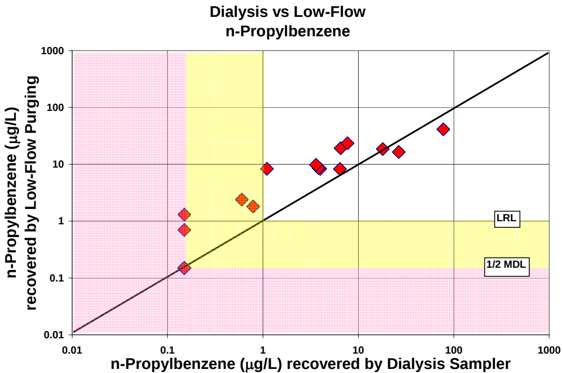
Figure A-30. Comparison of n-propylbenzene concentrations recovered by the dialysis sampler and low-flow purging
