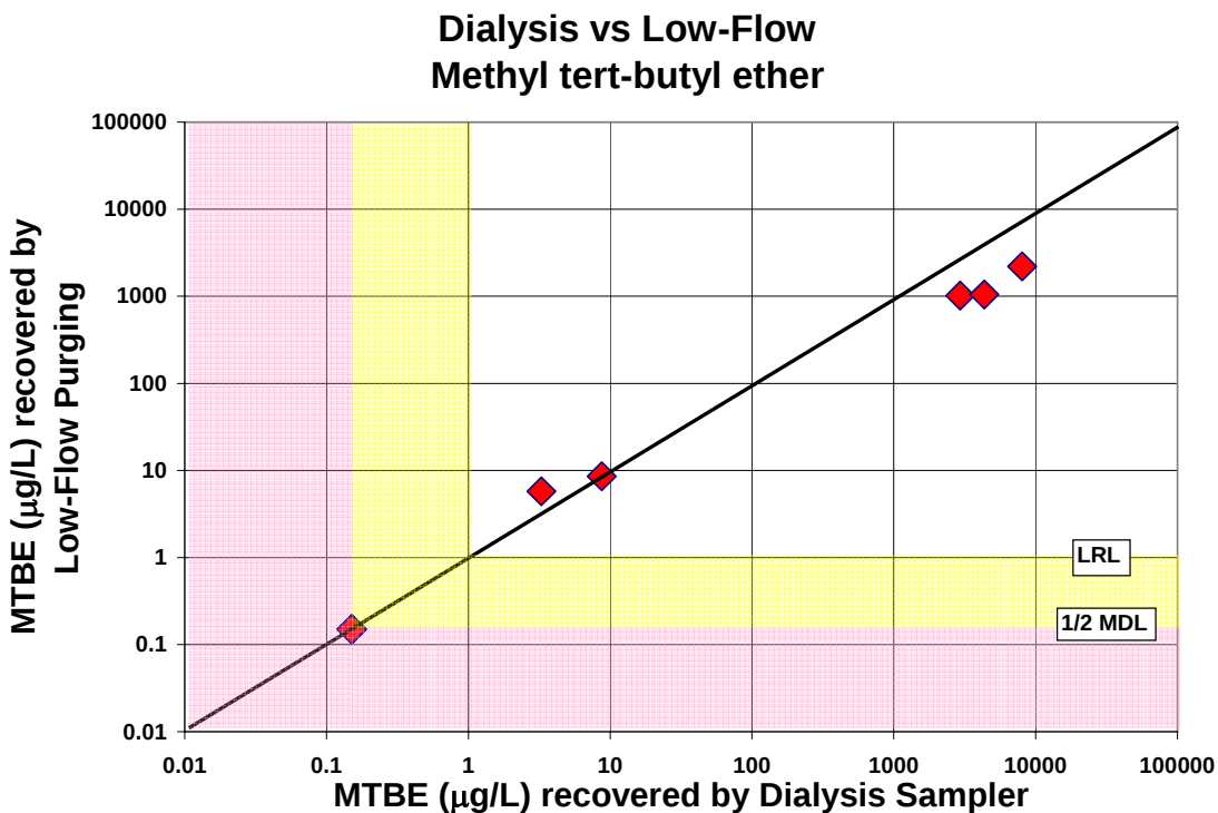
Figure A-24. Comparison of methyl-tert-butyl ether concentrations recovered by the dialysis sampler and low-flow purging
