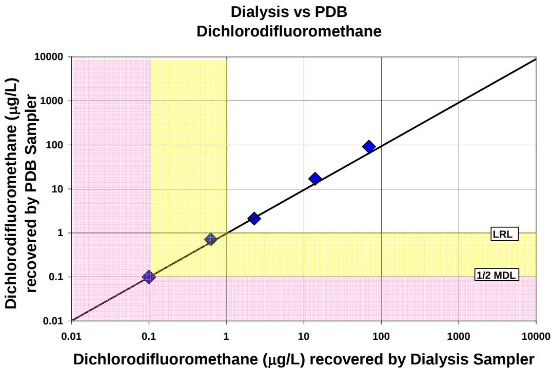
Figure A-15. Comparison of dichlorodifluoromethane concentrations recovered by the dialysis sampler and the polyethylene diffusion bag (PDB) sampler
