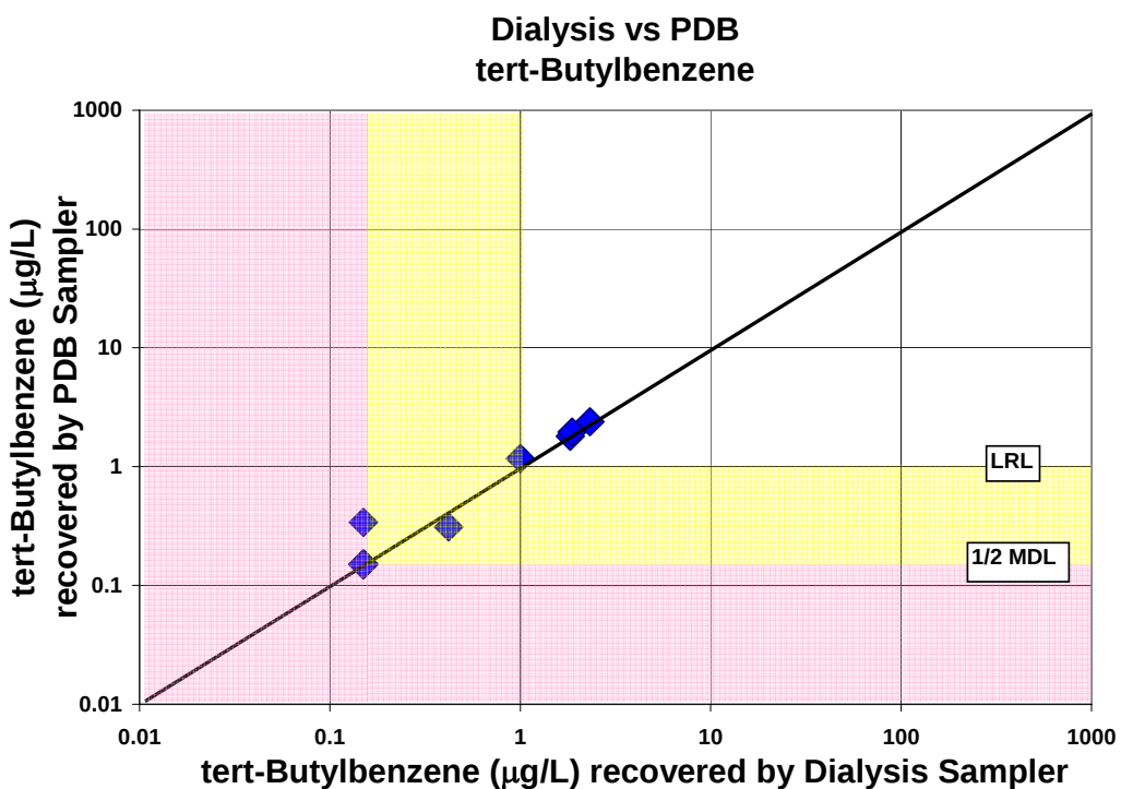
Figure A-39. Comparison of tert-butylbenzene concentrations recovered by the dialysis sampler and the polyethylene diffusion bag (PDB) sampler
