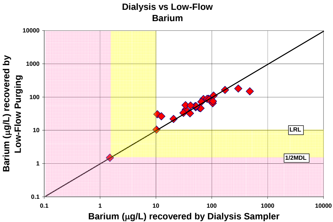
Figure A-63. Comparison of barium concentrations recovered by the dialysis sampler and low-flow purging
