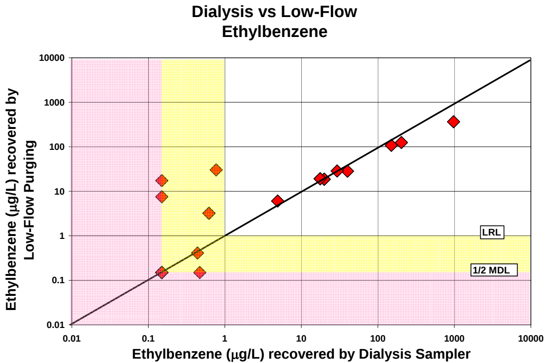
Figure 4-4. Dialysis Sampler Versus Low-Flow Purging Results For Ethylbenzene
