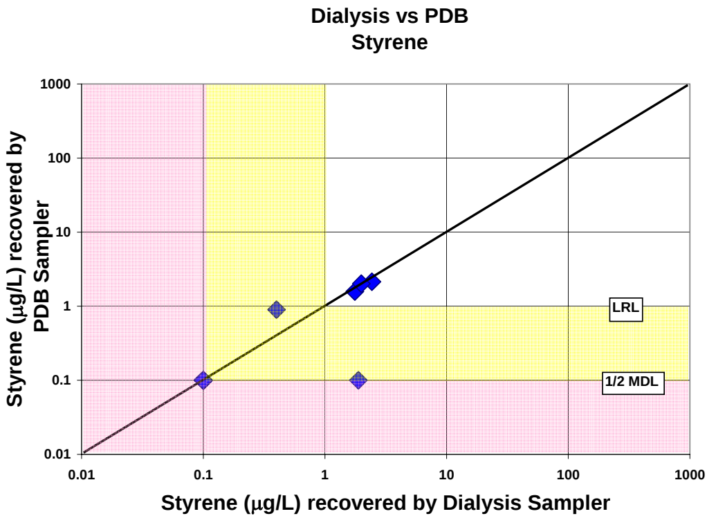
Figure A-37. Comparison of styrene concentrations recovered by the dialysis sampler and the polyethylene diffusion bag (PDB) sampler
