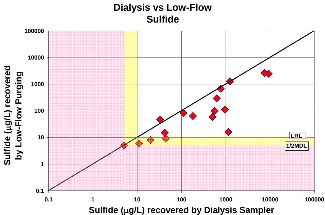
Figure A-77. Comparison of sulfide concentrations recovered by the dialysis sampler and low-flow purging
