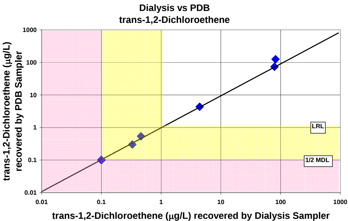
Figure A-45. Comparison of trans-1,2-dichloroethene concentrations recovered by the dialysis sampler and the polyethylene diffusion bag (PDB) sampler
