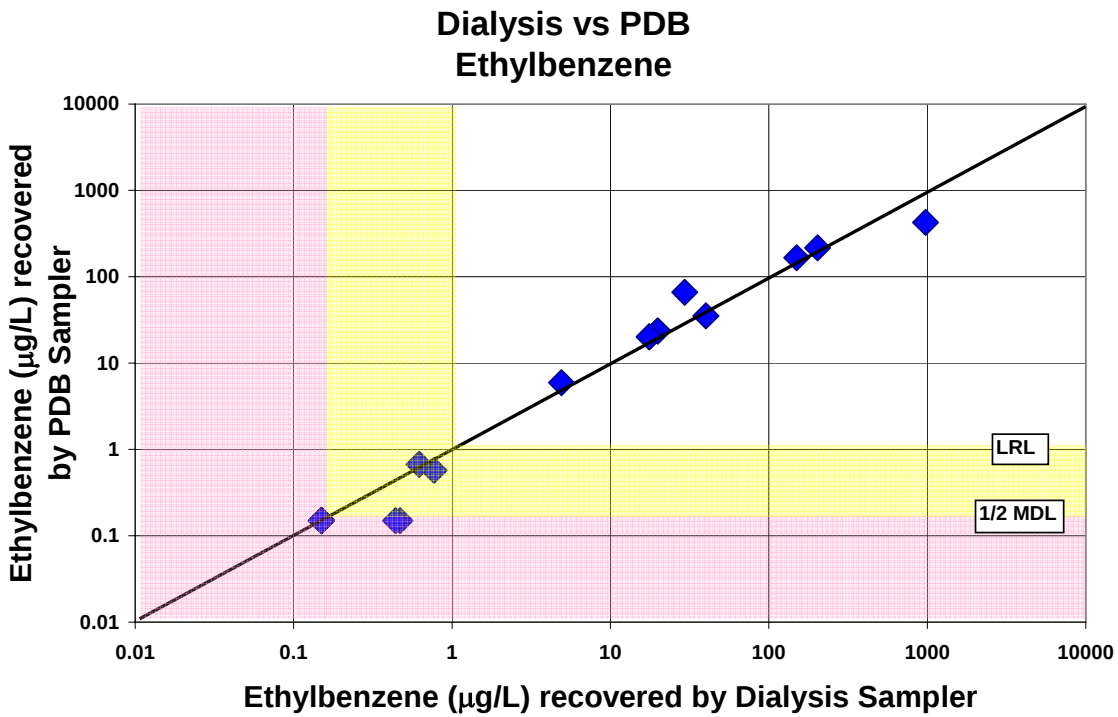
Figure A-17. Comparison of ethylbenzene concentrations recovered by the dialysis sampler and the polyethylene diffusion bag (PDB) sampler
