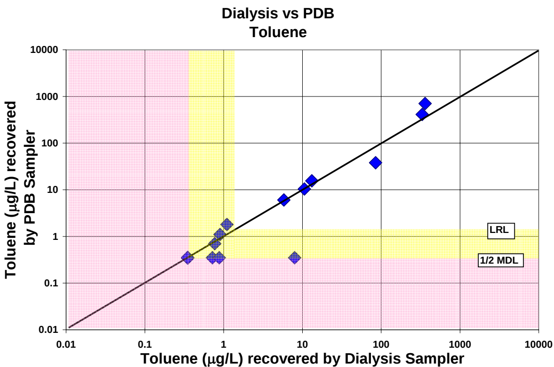
Figure A-43. Comparison of toluene concentrations recovered by the dialysis sampler and the polyethylene diffusion bag (PDB) sampler
