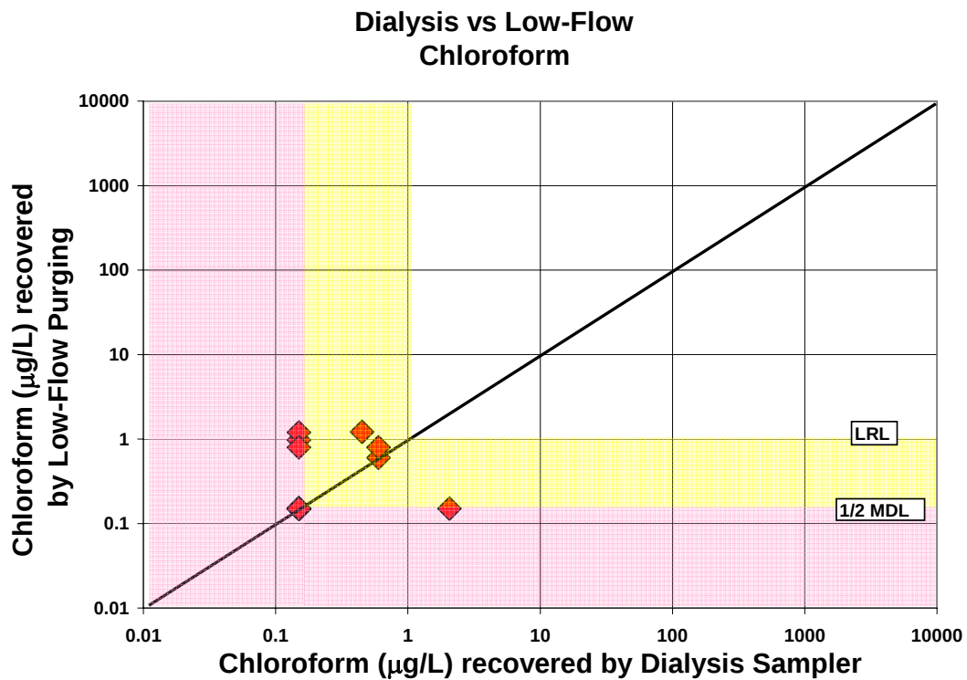
Figure A-14. Comparison of chloroform concentrations recovered by the dialysis sampler and low-flow purging
