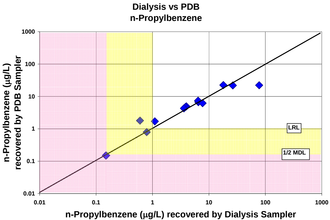
Figure A-29. Comparison of n-propylbenzene concentrations recovered by the dialysis sampler and the polyethylene diffusion bag (PDB) sampler
