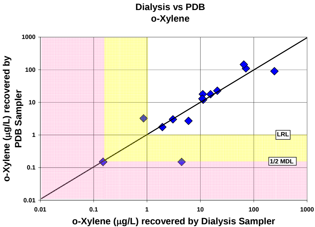
Figure A-31. Comparison of o-xylene concentrations recovered by the dialysis sampler and the polyethylene diffusion bag (PDB) sampler
