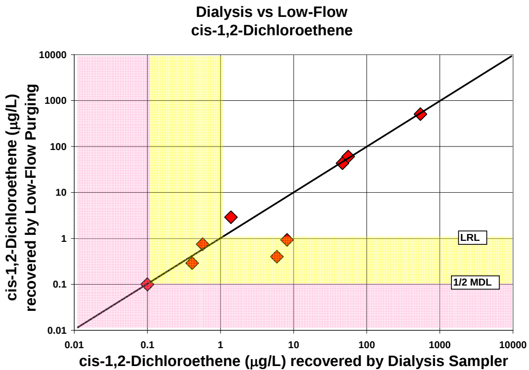
Figure A-12. Comparison of cis-1,2-dichloroethene concentrations recovered by the dialysis sampler and low-flow purging
