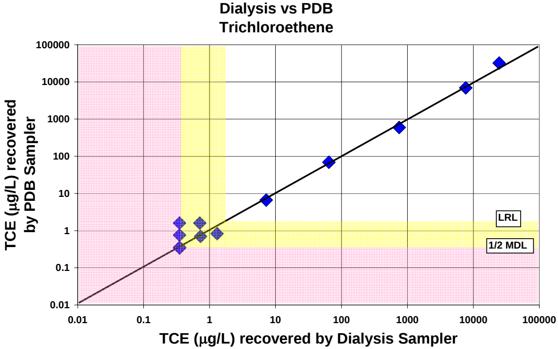
Figure A-41. Comparison of trichloroethene concentrations recovered by the dialysis sampler and the polyethylene diffusion bag (PDB) sampler
