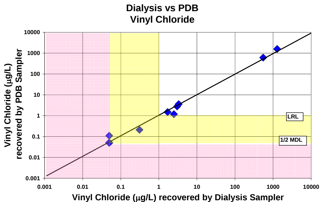
Figure 4-1. Dialysis Sampler Versus Polyethylene Diffusion Bag (PDB) Sampler Results For Vinyl Chloride
