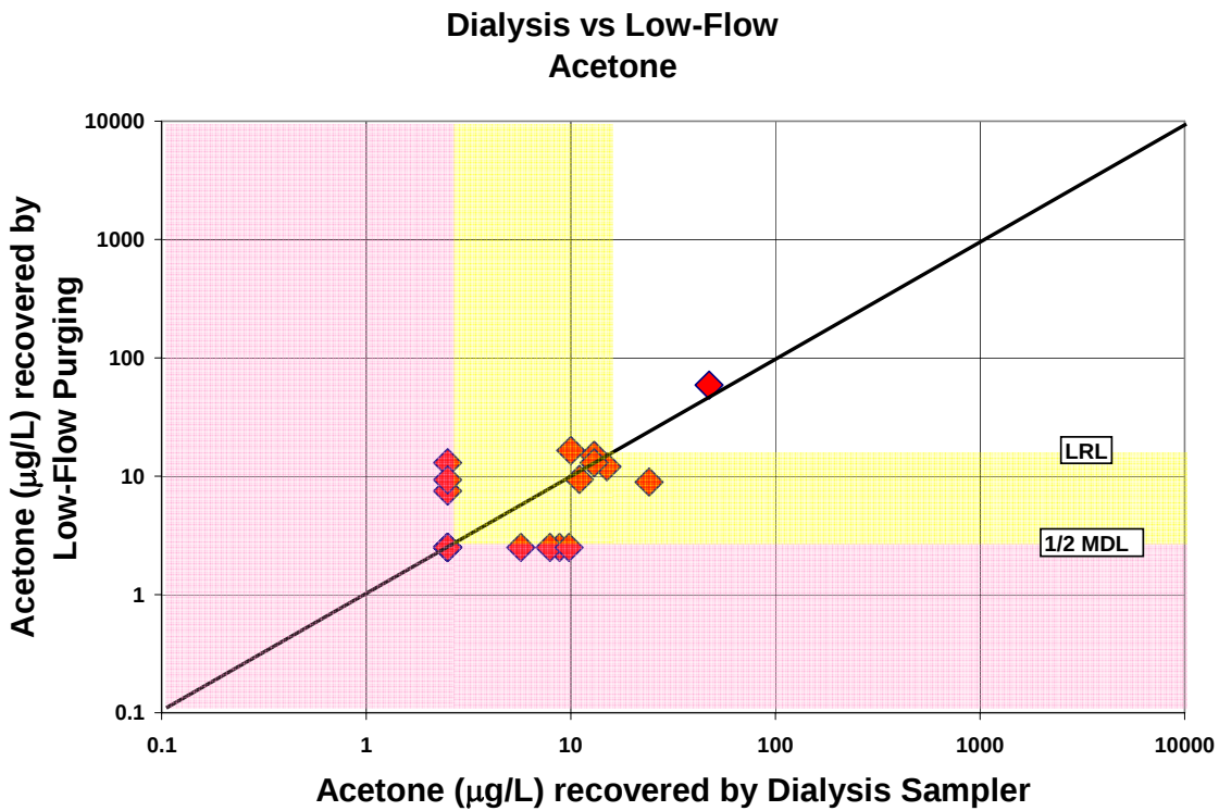
Figure A-49. Comparison of acetone concentrations recovered by the dialysis sampler and low-flow purging
