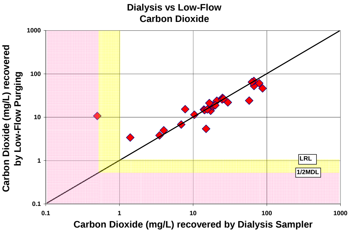
Figure A-74. Comparison of carbon dioxide concentrations recovered by the dialysis sampler and low-flow purging
