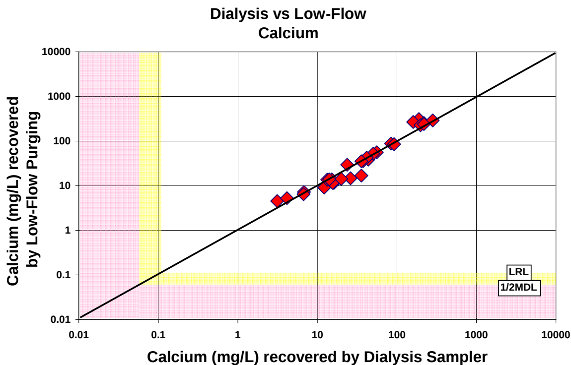
Figure 4-9. Dialysis Sampler Versus Low-Flow Purging Results For Calcium
