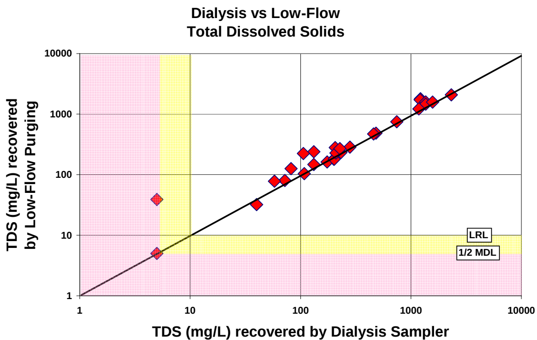
Figure A-79. Comparison of total dissolved solids (TDS) concentrations recovered by the dialysis sampler and low-flow purging
