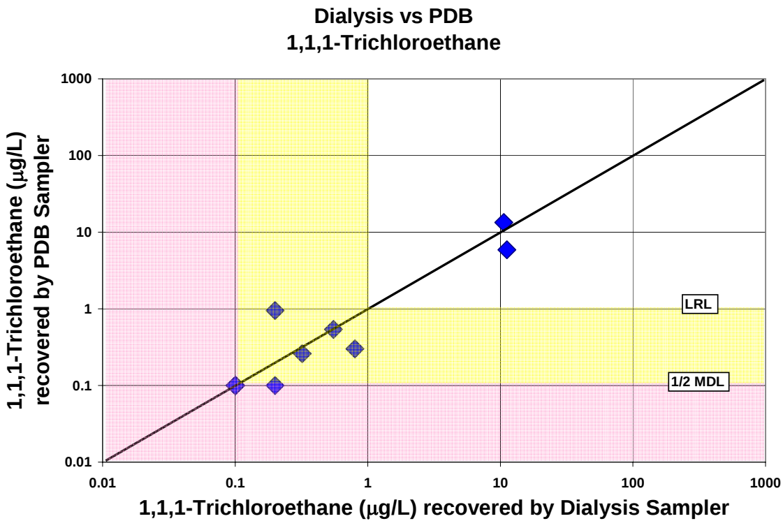
Figure A-1. Comparison of 1,1,1-trichloroethane concentrations recovered by the dialysis sampler and the polyethylene diffusion bag (PDB) sampler
