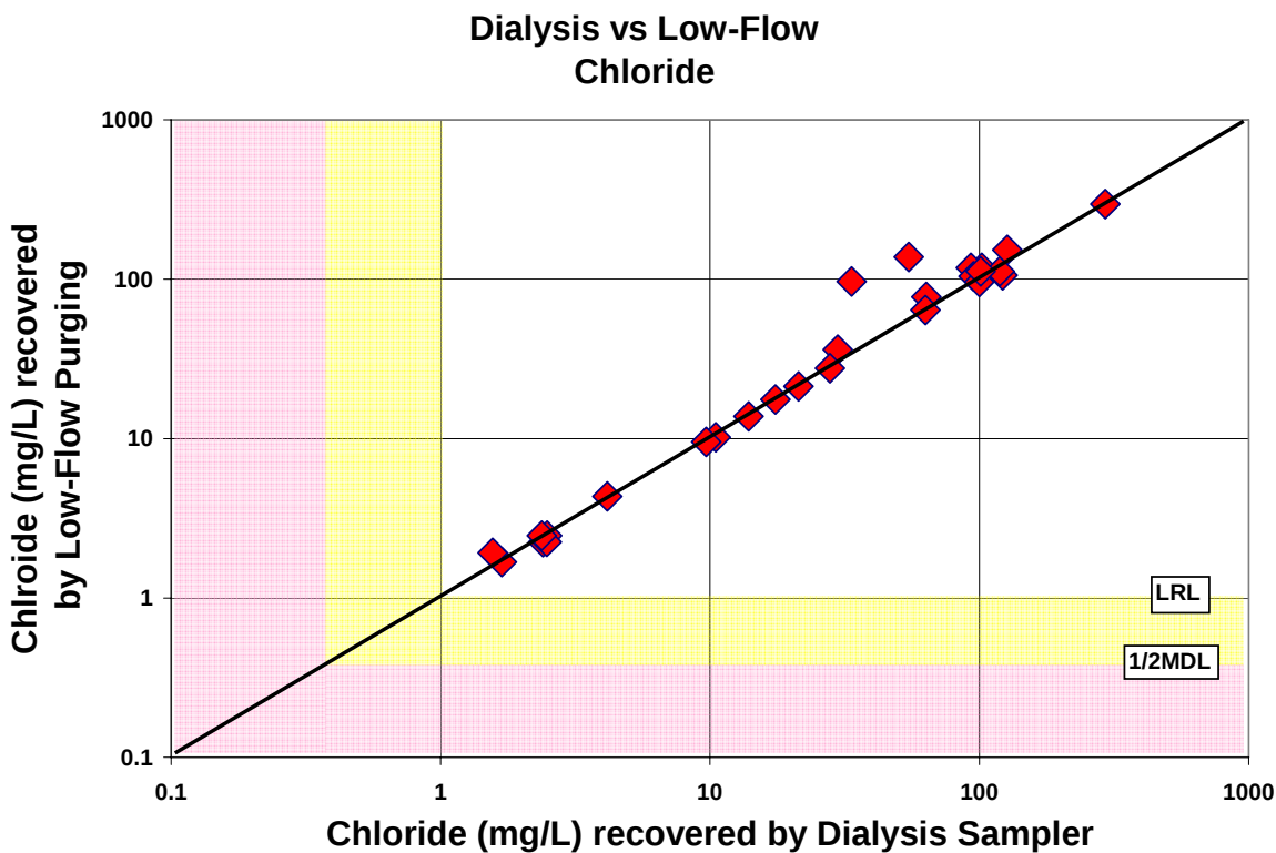
Figure 4-10. Dialysis Sampler Versus Low-Flow Purging Results For Chloride
