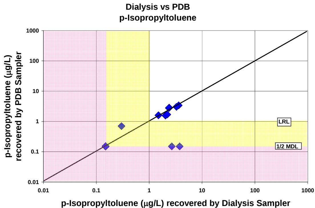
Figure A-33. Comparison of p-isopropyltoluene concentrations recovered by the dialysis sampler and the polyethylene diffusion bag (PDB) sampler
