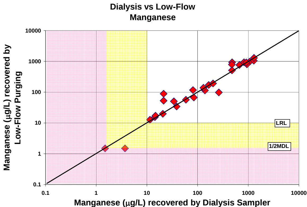
Figure 4-12. Dialysis Sampler Versus Low-Flow Purging Results For Manganese
