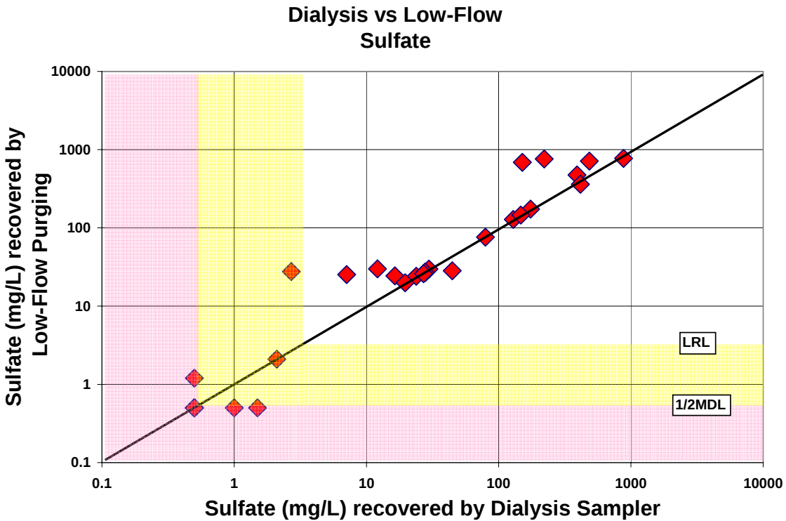
Figure A-56. Comparison of sulfate concentrations recovered by the dialysis sampler and low-flow purging
