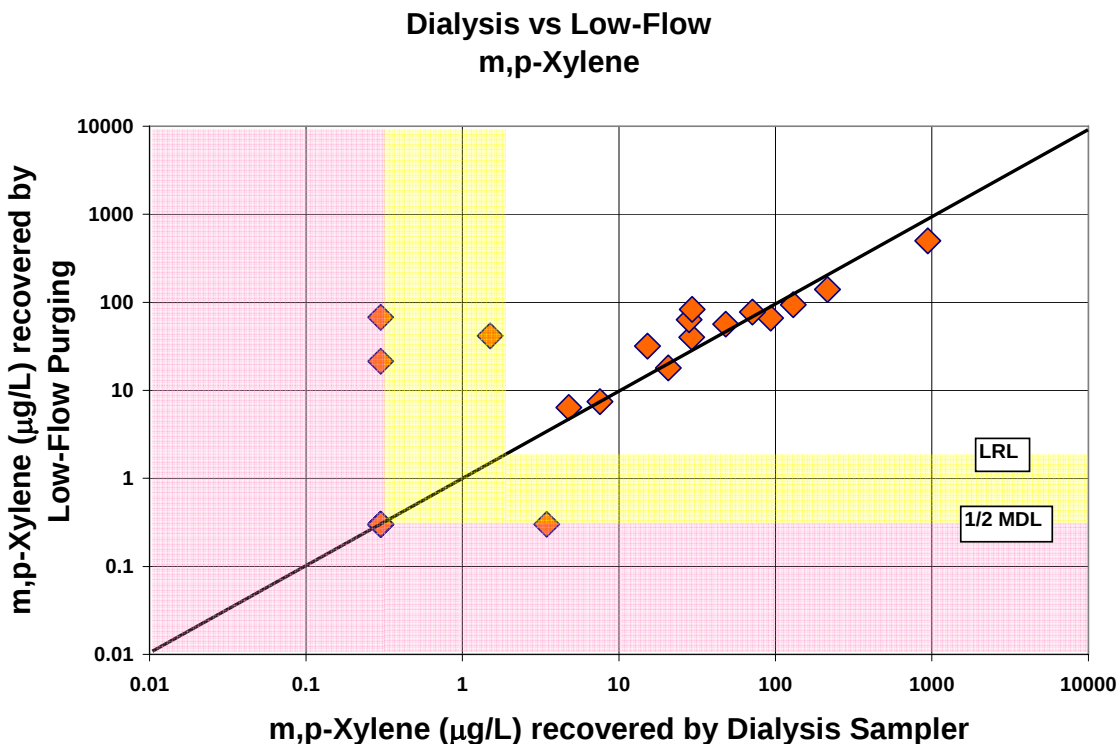
Figure A-22. Comparison of m,p-xylene concentrations recovered by the dialysis sampler and low-flow purging
