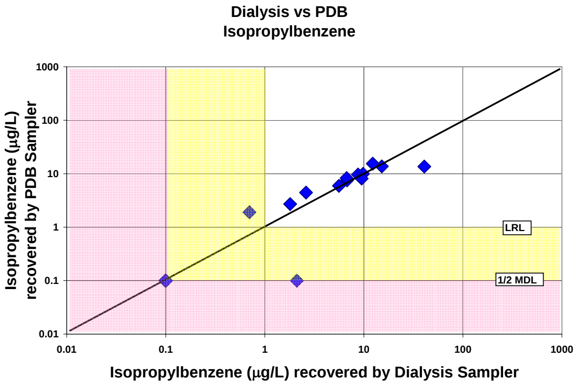
Figure A-19. Comparison of isopropylbenzene concentrations recovered by the dialysis sampler and the polyethylene diffusion bag (PDB) sampler
