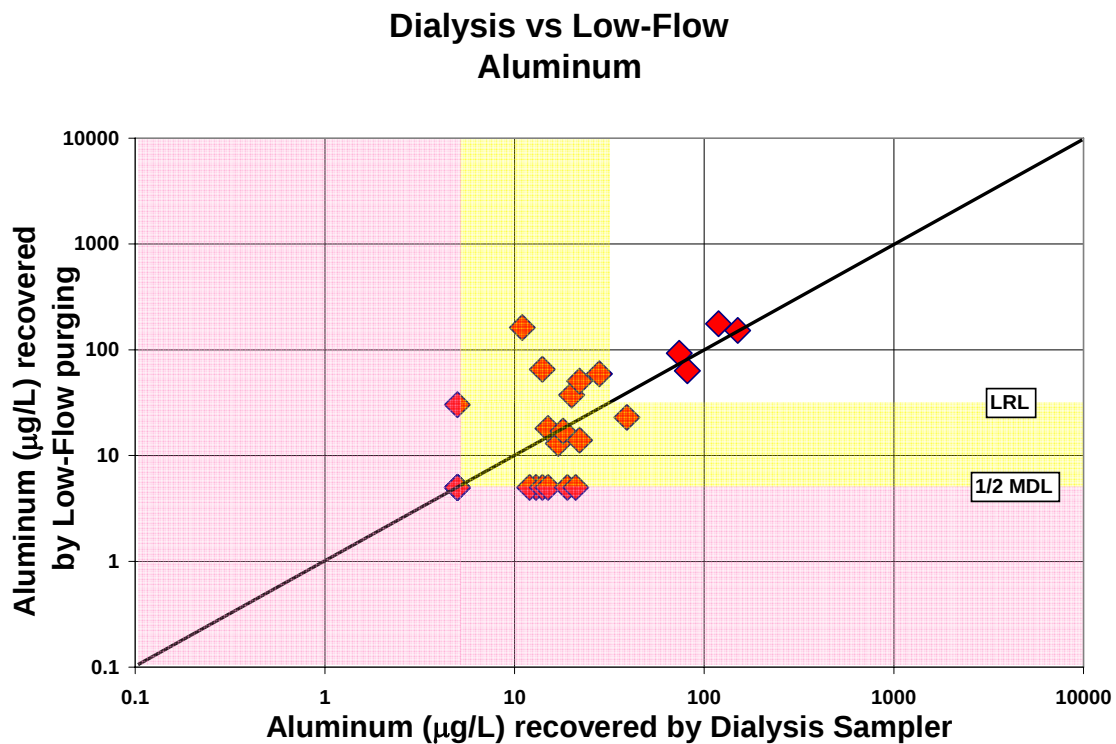
Figure A-61. Comparison of aluminum concentrations recovered by the dialysis sampler and low-flow purging
