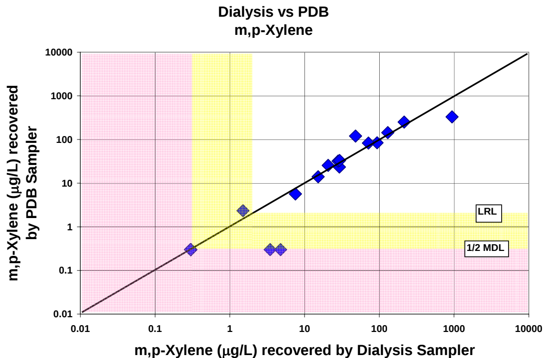
Figure A-21. Comparison of m,p-xylene concentrations recovered by the dialysis sampler and the polyethylene diffusion bag (PDB) sampler
