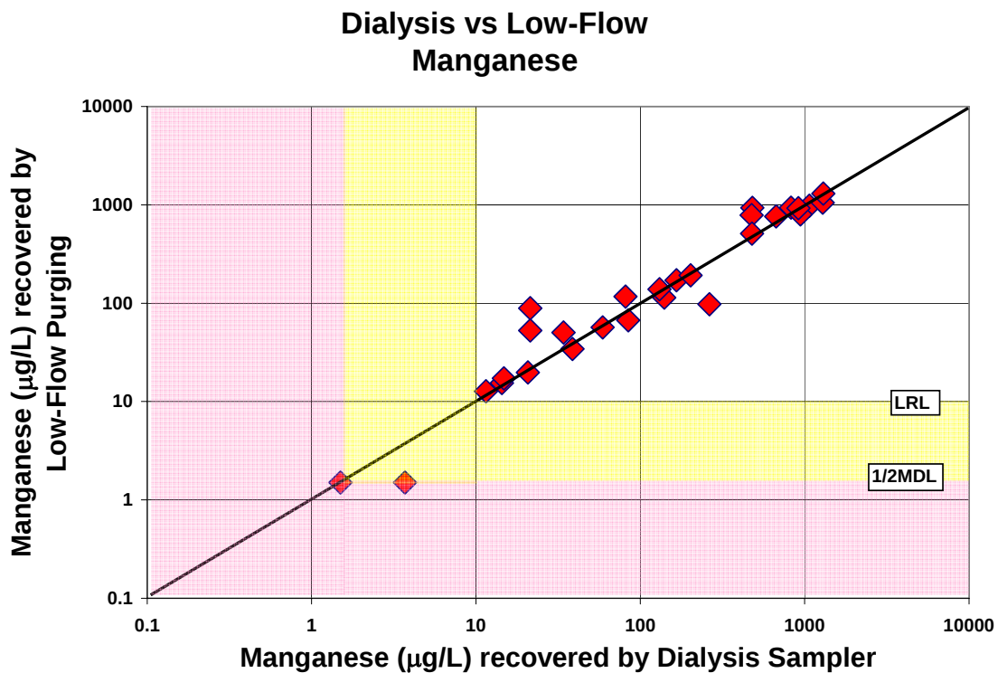
Figure A-67. Comparison of manganese concentrations recovered by the dialysis sampler and low-flow purging
