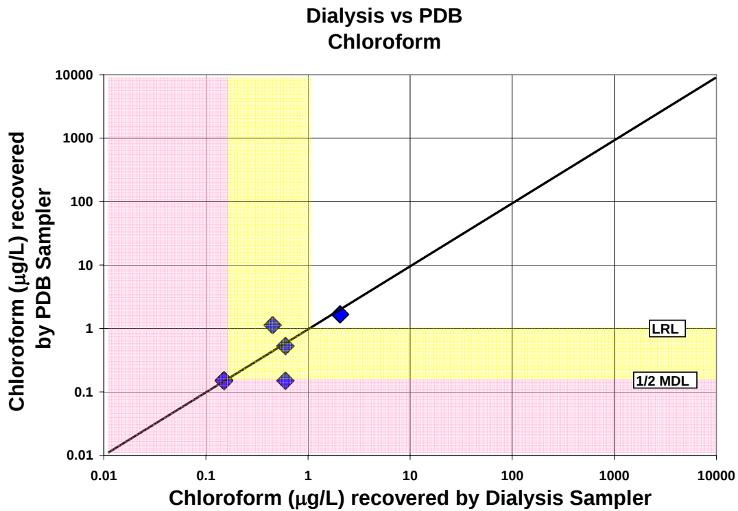
Figure A-13. Comparison of chloroform concentrations recovered by the dialysis sampler and the polyethylene diffusion bag (PDB) sampler
