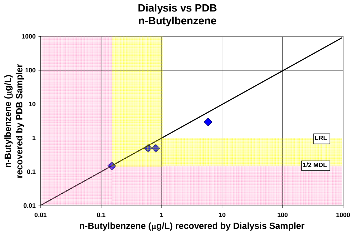
Figure A-27. Comparison of n-butylbenzene concentrations recovered by the dialysis sampler and the polyethylene diffusion bag (PDB) sampler
