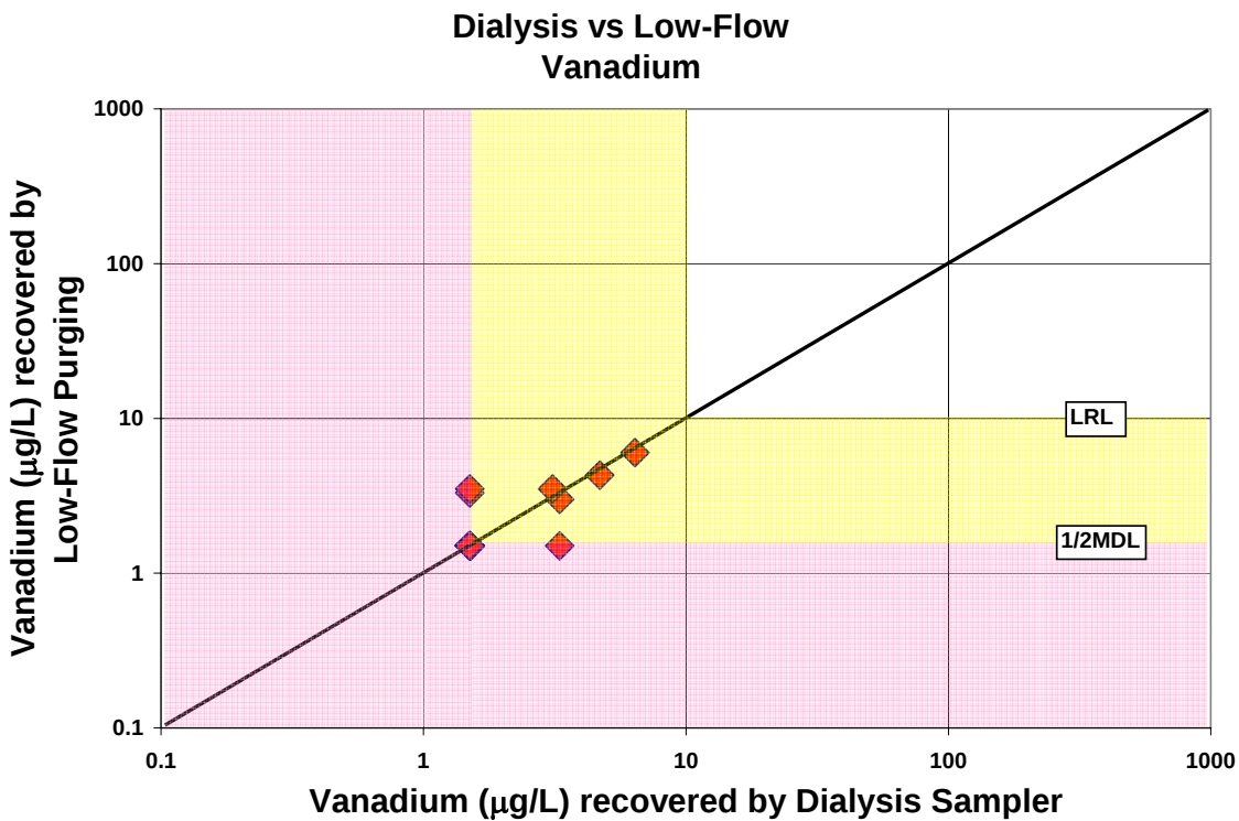
Figure A-72. Comparison of vanadium concentrations recovered by the dialysis sampler and low-flow purging
