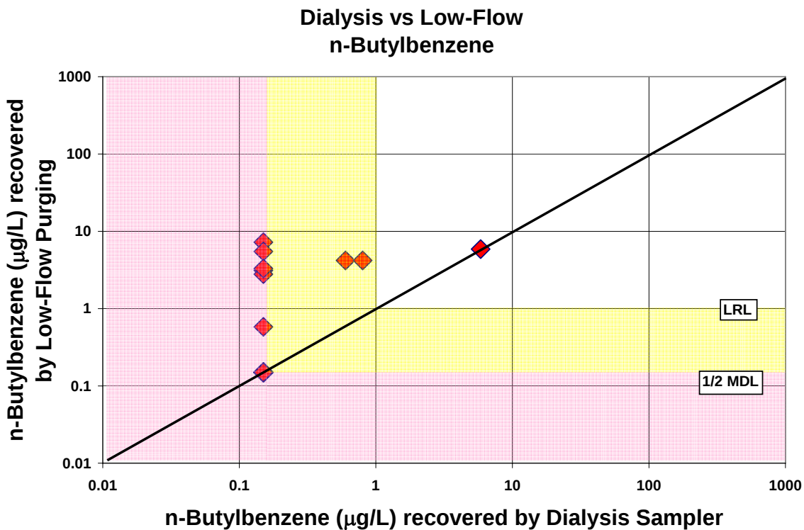
Figure 4-8. Dialysis Sampler Versus Low-Flow Purging Results For n-Butylbenzene
