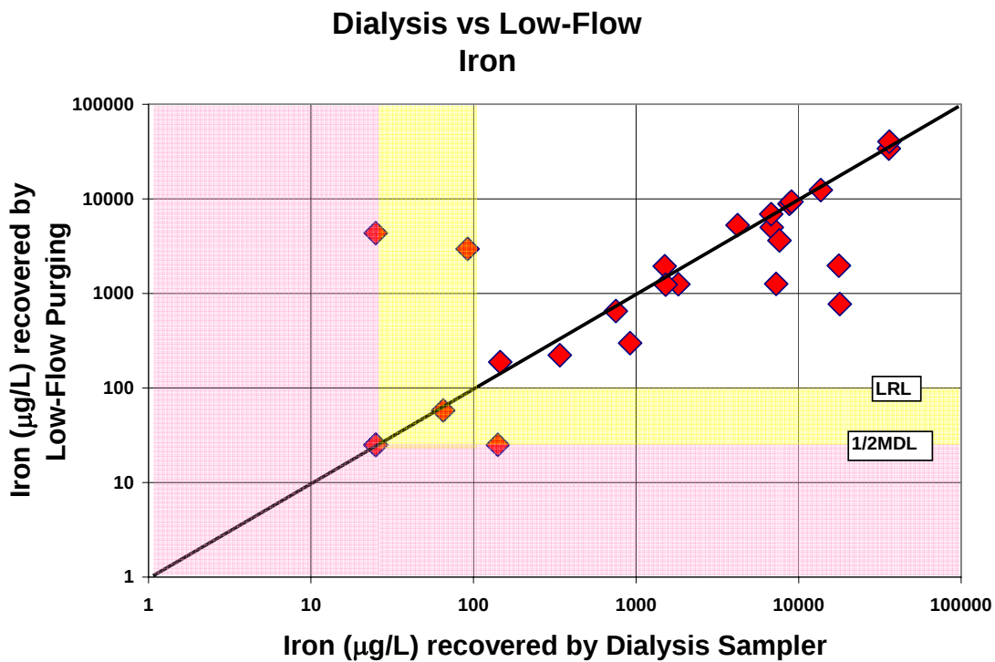
Figure A-66. Comparison of iron concentrations recovered by the dialysis sampler and low-flow purging
