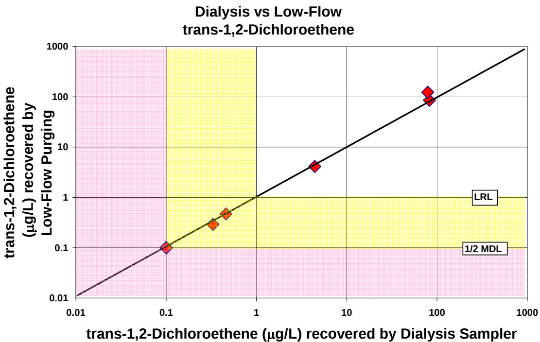
Figure A-46. Comparison of trans-1,2-dichloroethene concentrations recovered by the dialysis sampler and low-flow purging
