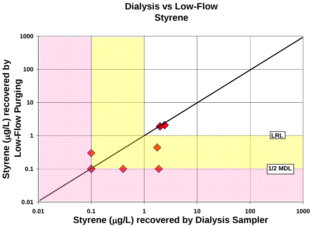
Figure A-38. Comparison of styrene concentrations recovered by the dialysis sampler and low-flow purging
