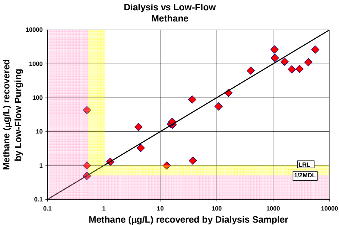
Figure A-76. Comparison of methane concentrations recovered by the dialysis sampler and low-flow purging
