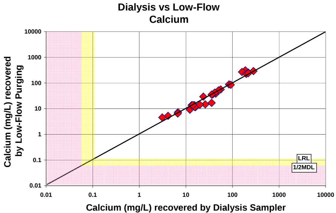
Figure A-50. Comparison of calcium concentrations recovered by the dialysis sampler and low-flow purging
