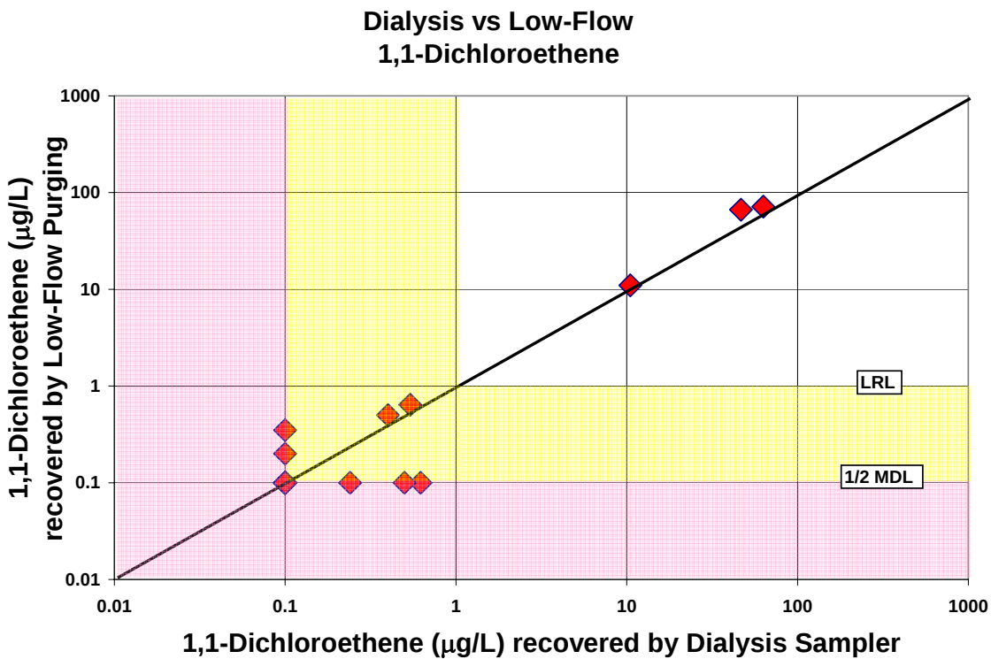
Figure A-4. Comparison of 1,1-dichloroethene concentrations recovered by the dialysis sampler and low-flow purging
