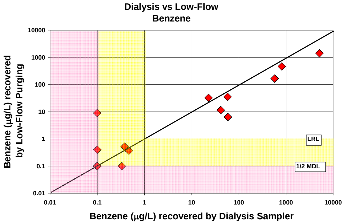
Figure A-10. Comparing of benzene concentrations recovered by the dialysis sampler and low-flow purging
