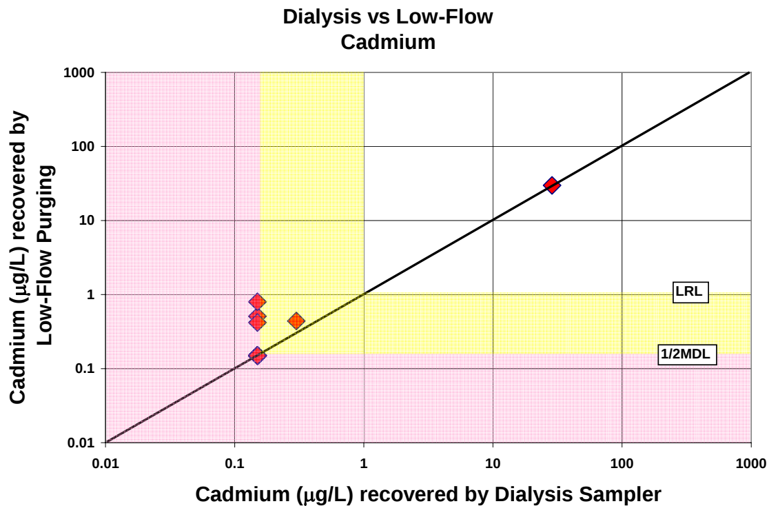
Figure A-64. Comparison of cadmium concentrations recovered by the dialysis sampler and low-flow purging
