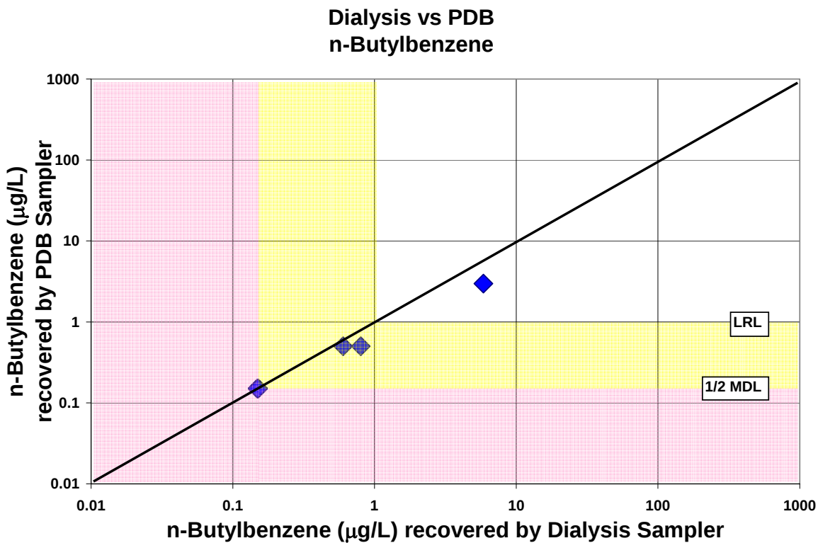
Figure 4-7. Dialysis Sampler Versus Polyethylene Diffusion Bag (PDB) Sampler Results For n-Butylbenzene
