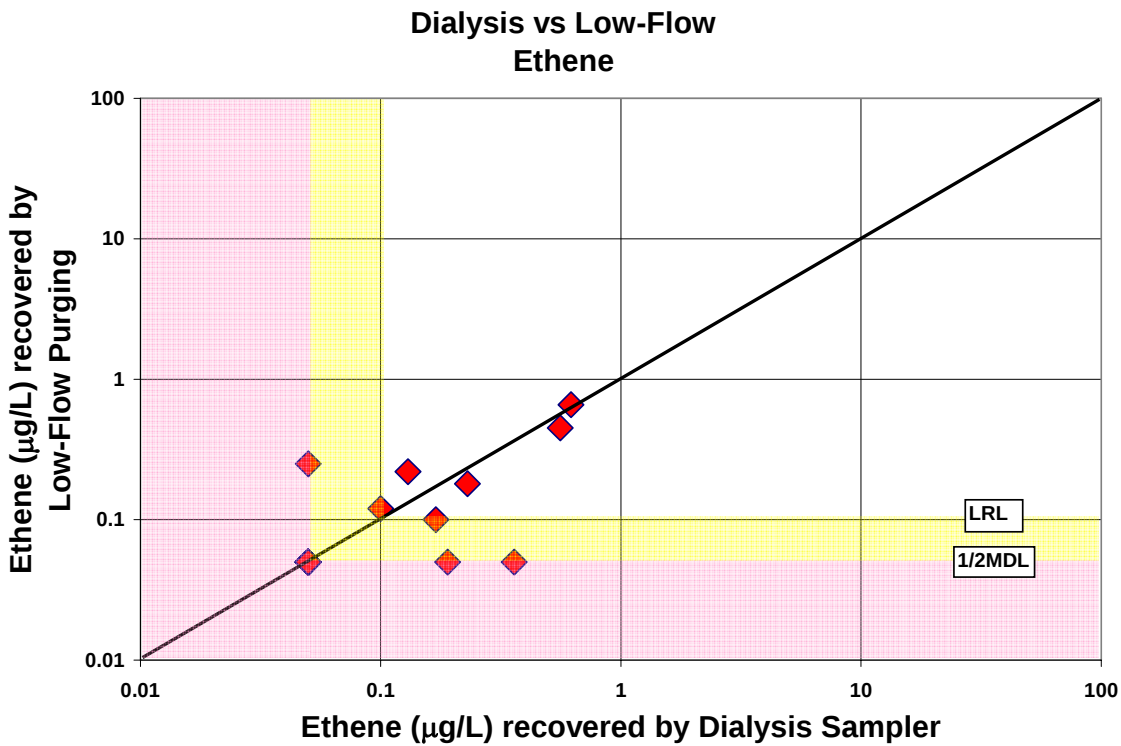
Figure A-75. Comparison of ethene concentrations recovered by the dialysis sampler and low-flow purging
