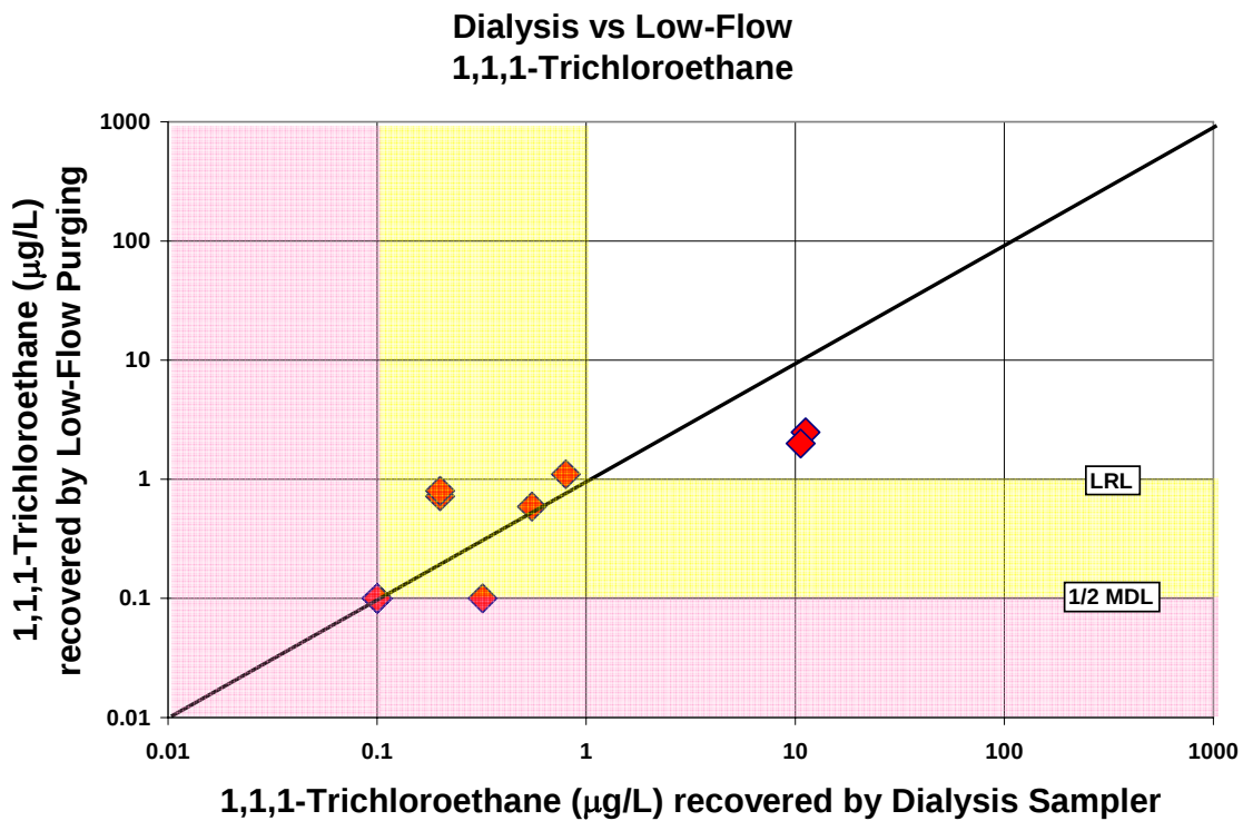
Figure A-2. Comparison of 1,1,1-trichloroethane concentrations recovered by the dialysis sampler and low-flow purging
