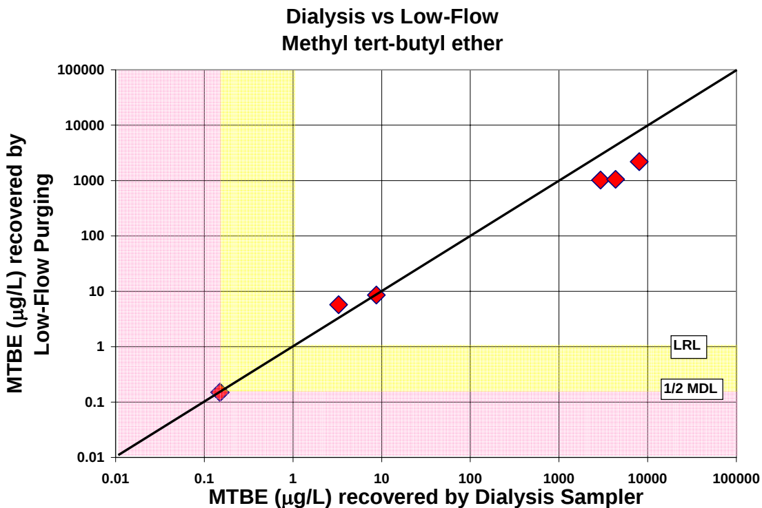
Figure 4-6. Dialysis Sampler Versus Low-Flow Purging Results For Methyl Tert-Butyl Ether
