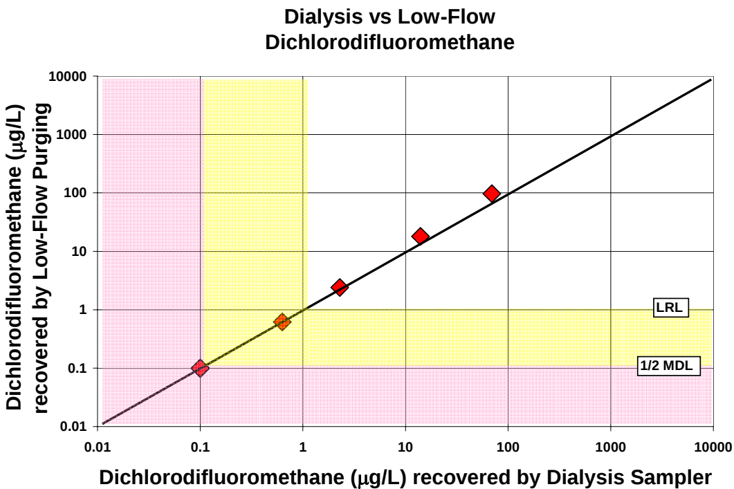
Figure A-16. Comparison of dichlorodifluoromethane concentrations recovered by the dialysis sampler and low-flow purging
