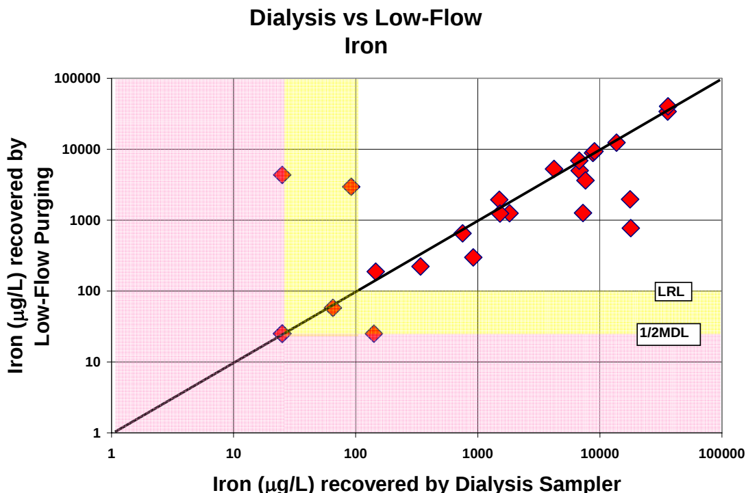
Figure 4-13. Dialysis Sampler Versus Low-Flow Purging Results For Iron
