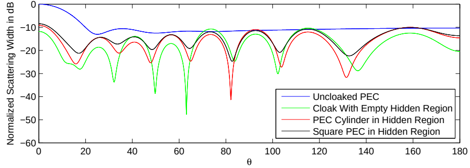
Figure 4.2: Normalized scattering width for a simplified cloak with various hidden objects.
