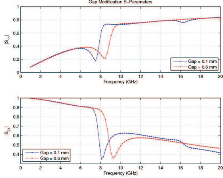
Figure 6.6: S-Parameter Magnitudes for Gap Modifications
