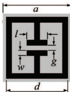
Figure 3.1: ELC Resonator [80]
