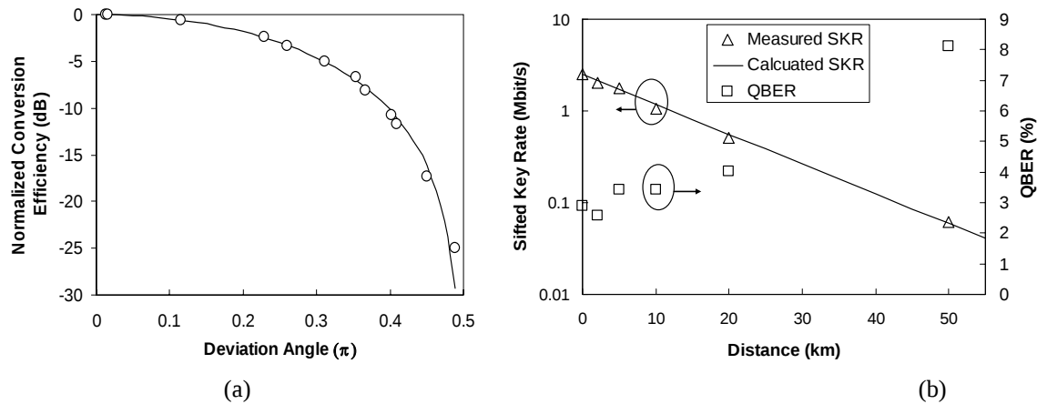
Figure 8. (a) Normalized conversion efficiency as a function of deviation angle of the input 1306-nm signal of the PPLN1. The x-axis shows the deviation angle in unit of \pi -rad. Open circle: Measurement results; Solid line: \cos^2 curve. The PPLN 2 detector exhibits similar behaviors. (b) System performance of the B92 polarization-based QKD system with the 1557-nm pumped up-conversion detector. The solid line (to the left): calculated sifted-key rate; The triangles: sifted-key rate measured in the experiment; The squares (to the right): error rate measured in the experiment.
