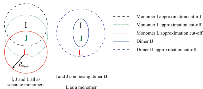
Figure 6. Illustration of FMO approximations applied to three monomers I , J , L (left) and as applied to dimer IJ and monomer L (right).
