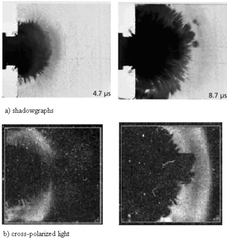
Figure 1. Selection of two shadowgraphs and corresponding crossed polarizers Pictures from impact on AlON at 380 m/s.
