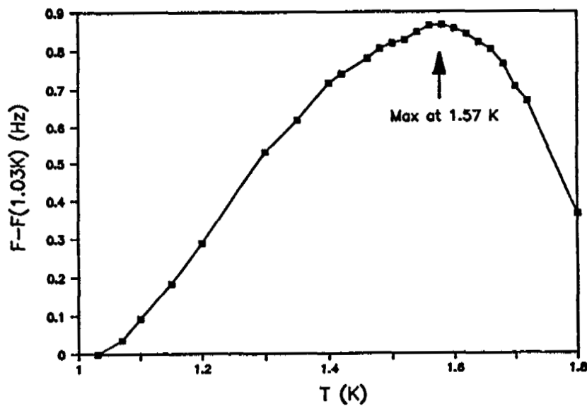
Figure 3. Measured frequency vs Temperature plot for range 1 - 1.8 Kelvin. 0.9 Hz frequency variation is referred to \approx 2.69 GHz reference.
