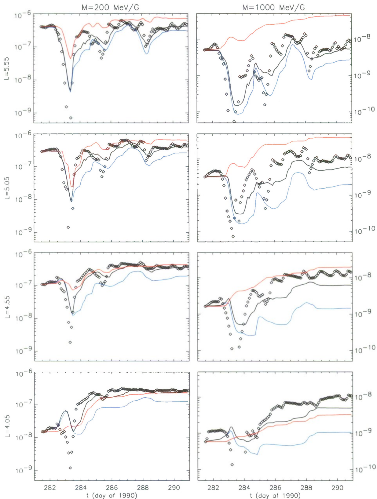
Figure 12. Phase space density, in units of \text{s}^3 \text{ km}^{-6} , as determined from CRRES data (black diamonds), and simulations starting at t = 281.5 , with D_{LL} only (blue curves), with chorus only (red curves), and with both (black curves).
