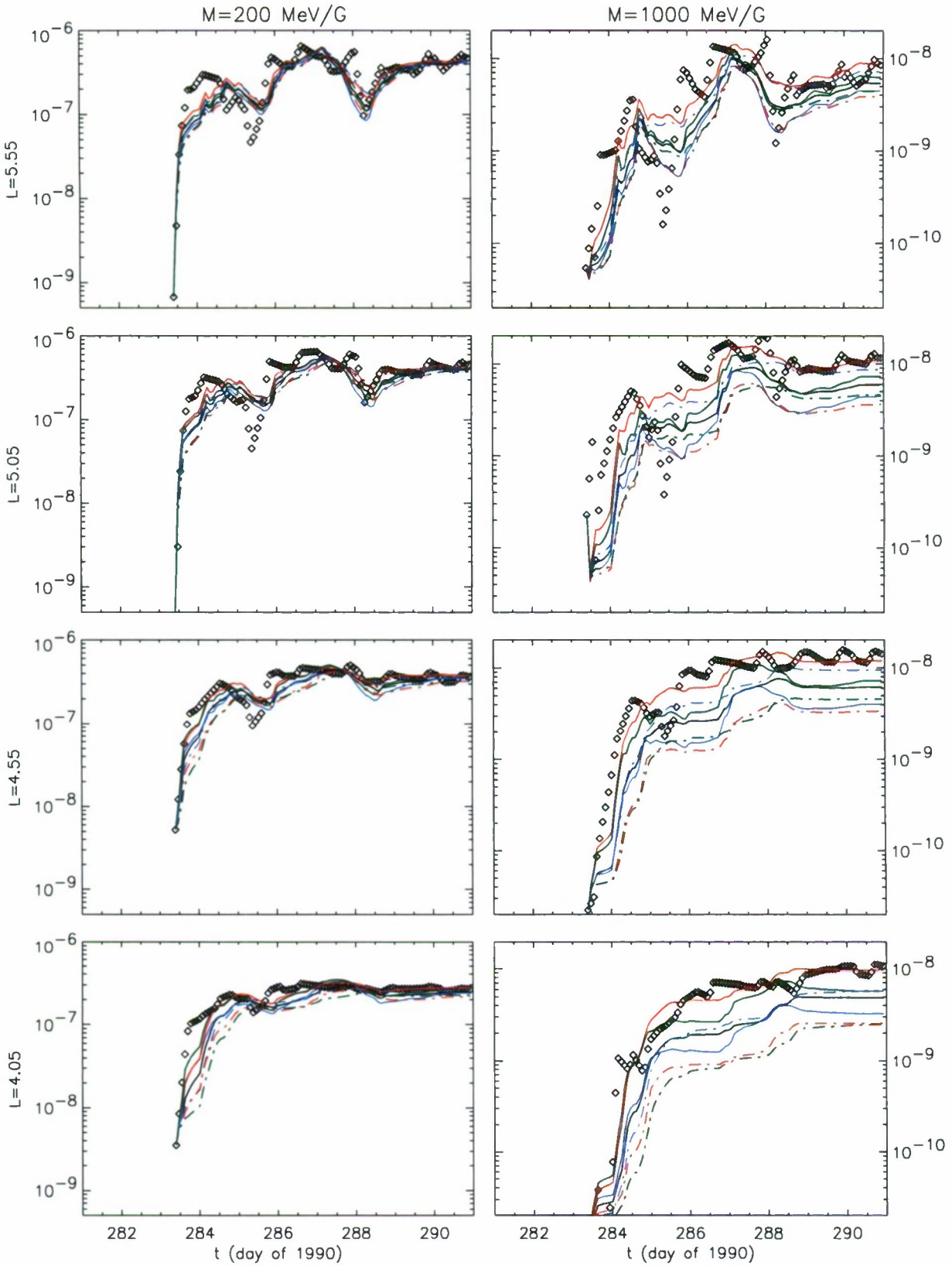
Figure 15. Phase space density as determined from CRRES data (black diamonds) and simulations as in Figure 14, starting at t = 283.4 .
