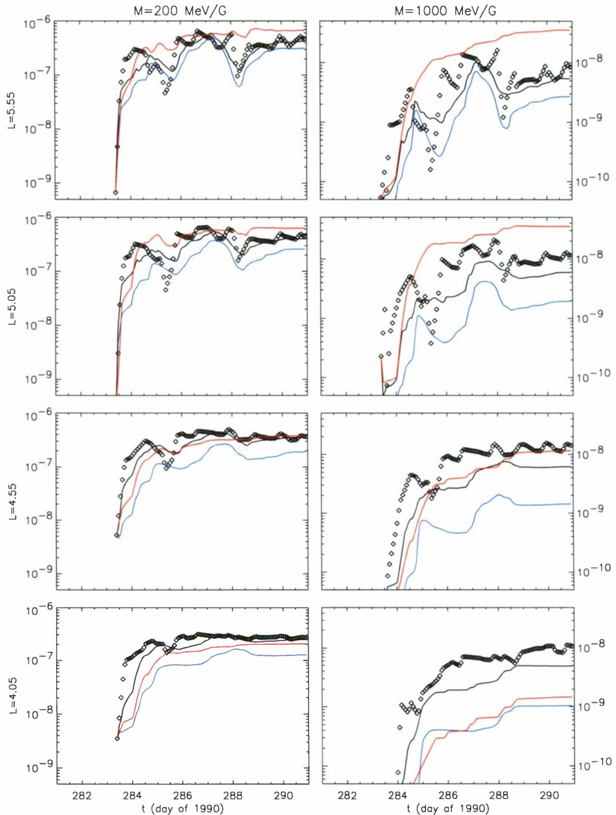
Figure 13. Phase space density, in units of s^3 \text{ km}^{-6} , as determined from CRRES data (black diamonds), and simulations starting at t = 283.4 , with D_{LL} only (blue curves), with chorus only (red curves), and with both (black curves).
