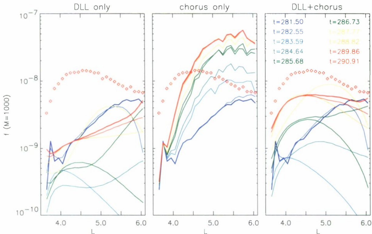
Figure 16. Snapshots of phase space density versus L at various values of t for M = 1000 MeV/G, simulated with D_{LL} only, D_{\text{chorus}} only, and both. CRRES data at the end of the simulation is shown as red diamonds in all three plots.
