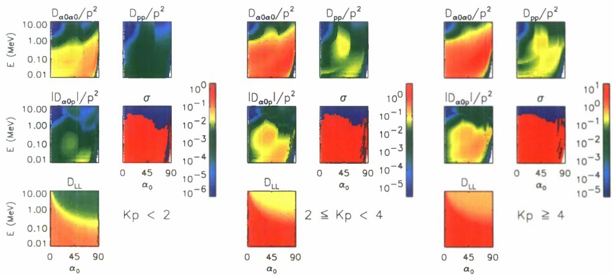
Figure 3. Diffusion coefficients at L = 4.55 , units are per day. The sign of D_{\alpha_0 p} is indicated by \sigma (red for positive, blue for negative). D_{LL} is evaluated at Kp = 1 , Kp = 3 , and Kp = 5 .
