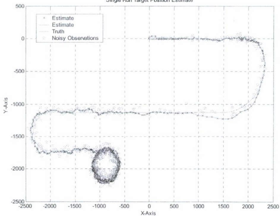
Figure 5. Noisy Observations
