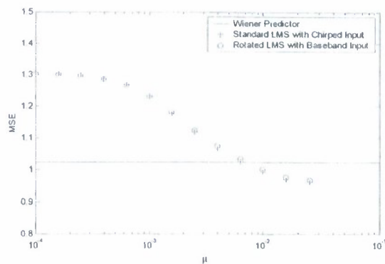
Figure 3. MSEs of Wiener predictor, standard LMS with chirped AR1 input signal, and rotated LMS with stationary input signal. The signal pole location is at a = 0.9 , filter length M = 10 , the prediction distance is 5, chirp rate is \psi = 5e - 4 .
