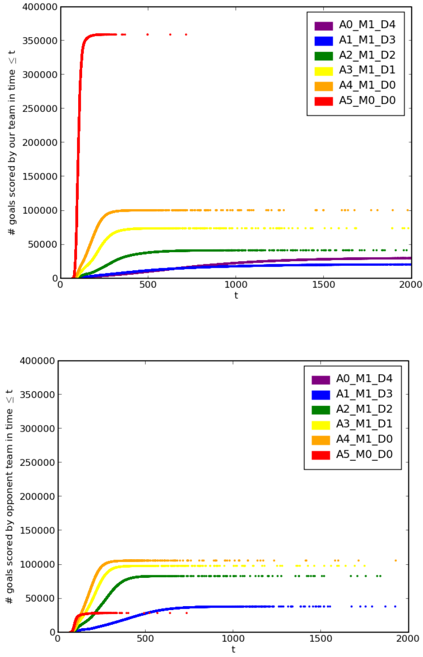
Figure B.9: Time-to-score distributions for the blue team (top) and for the red team (bottom) when the blue team plays A4_M1_D0, for each possible red play.
