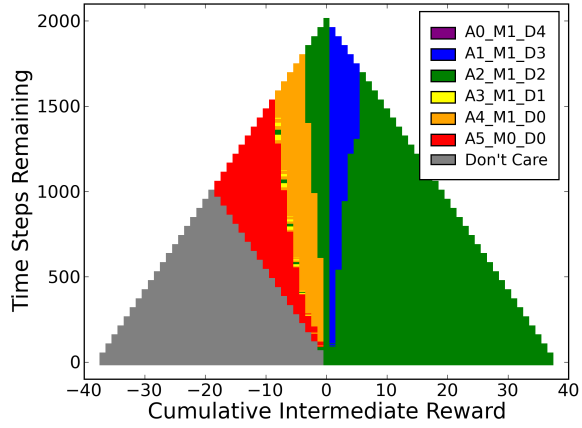
(c) Threshold-plus-linear-10 threshold function.
