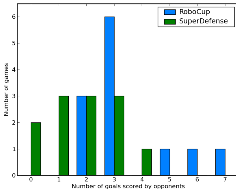
Figure 5.9: Histogram of the number of goals scored per game for the two conditions. When our team uses the SUPERDEFENSE play, the opponents score significantly fewer goals.
