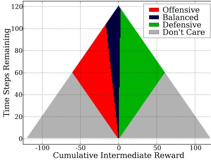
Figure 3.3: The optimal policy for M (shown in Figure 3.1), with time horizon h = 120 steps.
