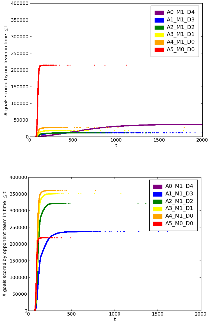
Figure B.11: Time-to-score distributions for the blue team (top) and for the red team (bottom) when the blue team plays A5_M0_D0, for each possible red play.
