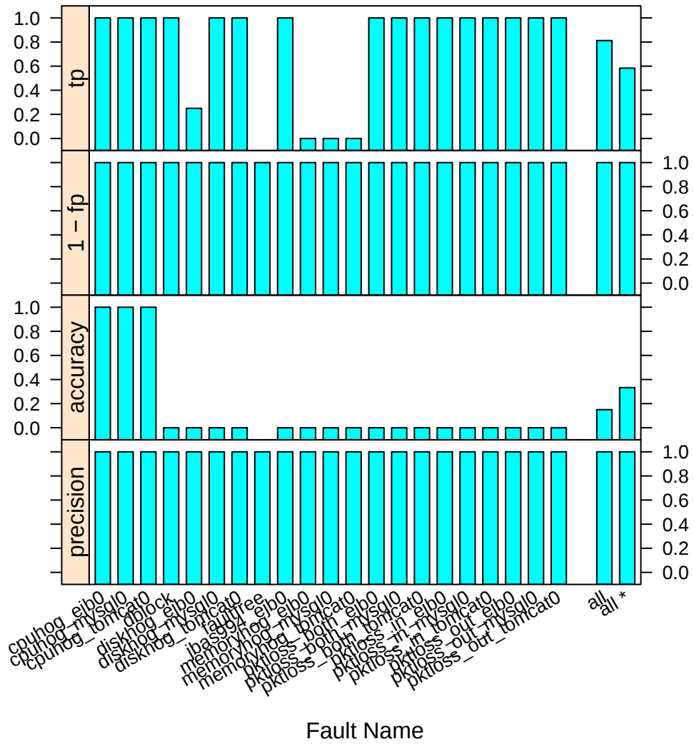
Figure 7.12: Results for Technique 1 with limited labeling.
