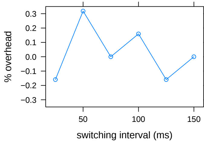
Figure 7.16: Overheads introduced by instrumentation: with multiplexing.
