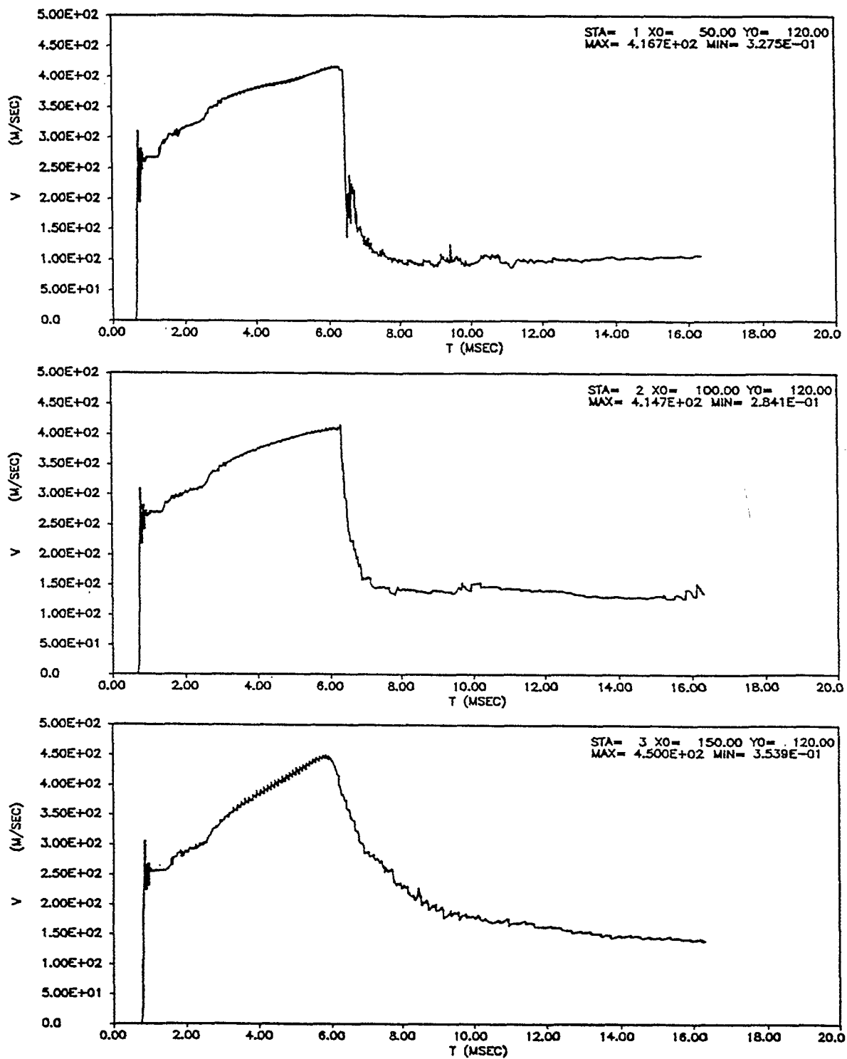
Figure 11. Velocity Histories at Several Lagrangian Stations for a Representative Test Simulation Computation.
