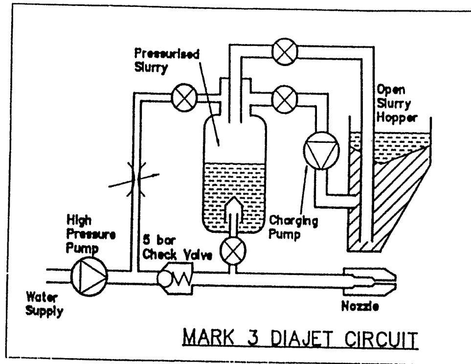
FIGURE 1 RMCS WATER JET SYSTEM
