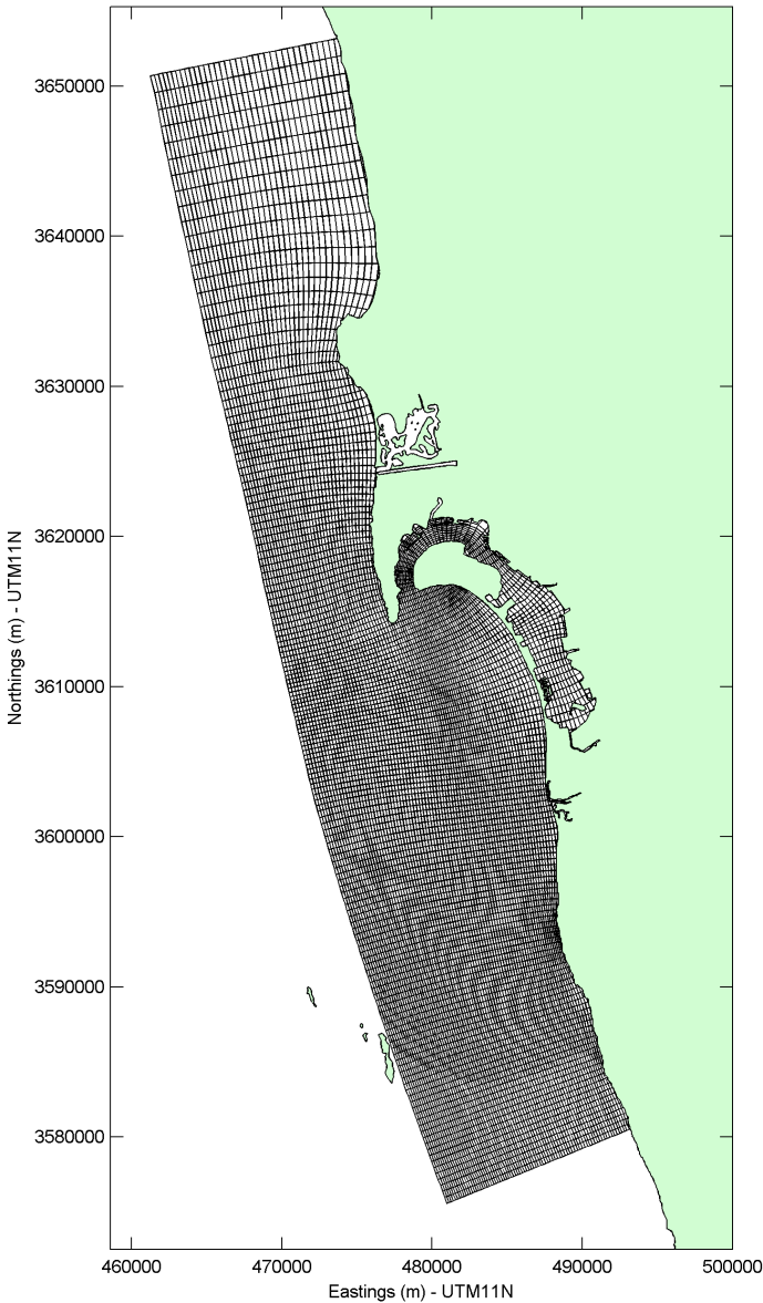
Figure 1. The Delft 3D Model domain used for assessing model performance and for the development of assimilation techniques for REMUS AUV based observation.
