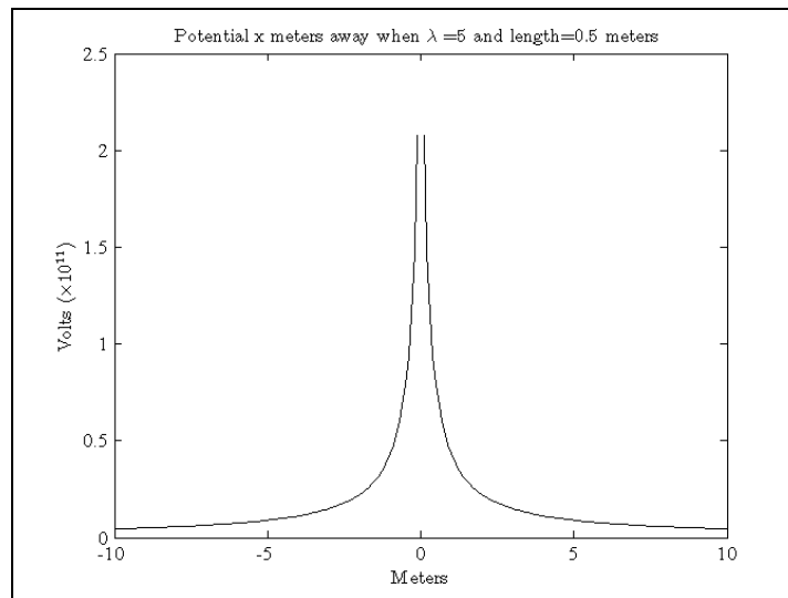
FIGURE 1. Line Charge Problem Results, Voltage vs. Distance From Line. The line charge was centered at x = 0 , and the distances were varied only in the y direction.
