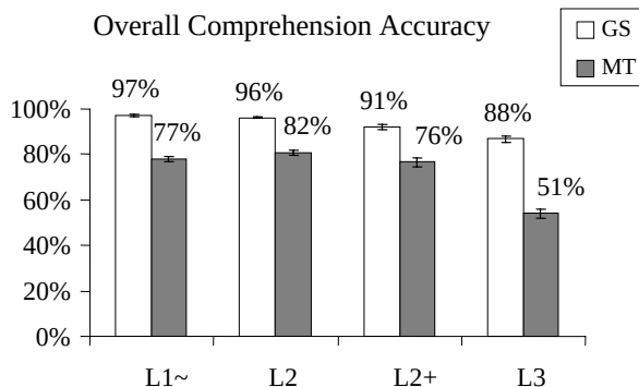
Figure 2. Comprehension Accuracy per Level.
