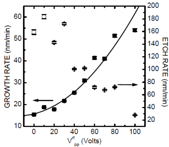
Fig. 11 Growth (solid) and etch (open) rate variation with applied rf peak-to-peak voltage ( V_{pp}^{rf} ).
