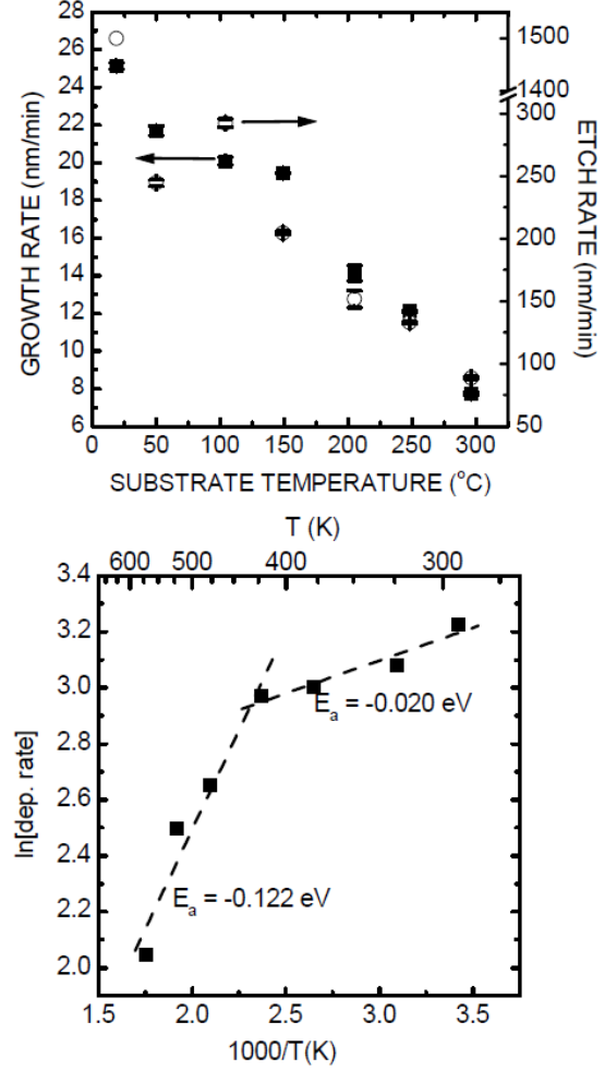
Fig. 9 (Top) Growth (solid) and etch (open) rate variation with substrate temperature and, (bottom) Arrhenius-type plot of growth rate data. The calculated activation energies ( E_a ) are shown on their respective linear fits.
