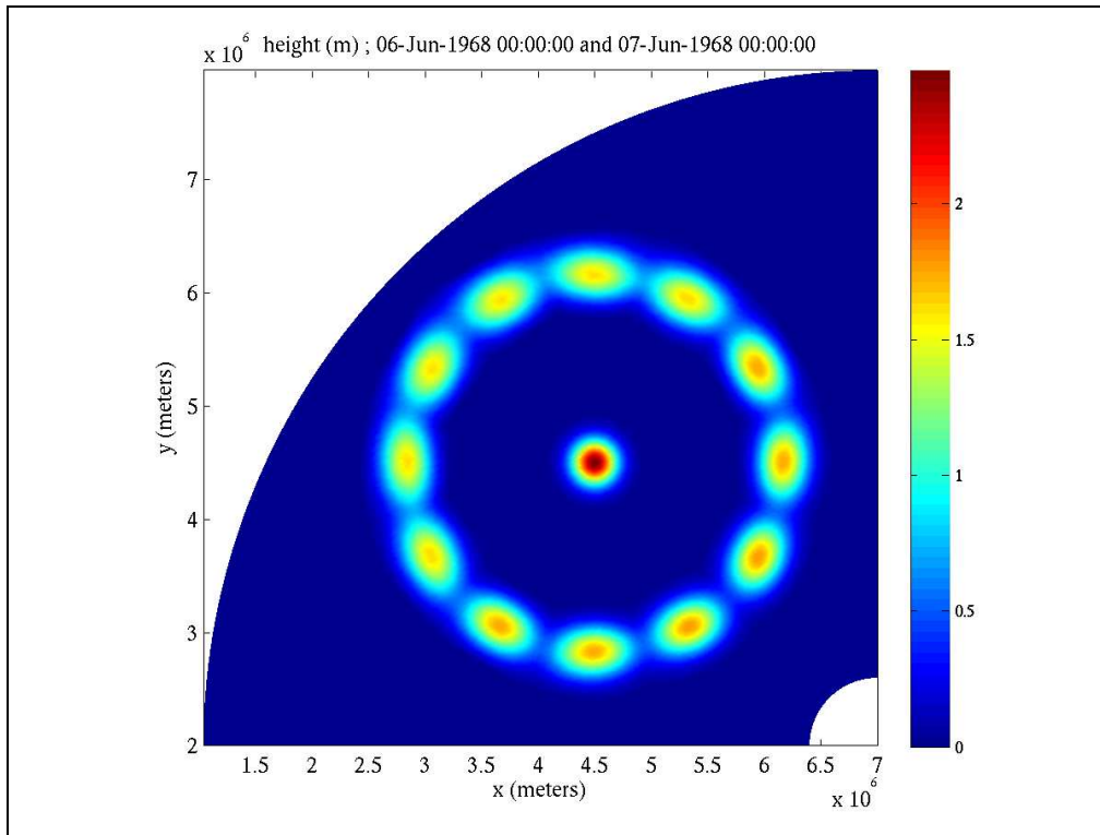
Figure 4-8 Test case 2.1c, PR3 w/default GSE settings, \alpha_s = \alpha_n = 1.50 . H_{m0} (m) plotted.
