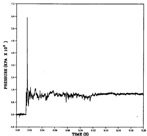
Figure 19. Experimental data overpressure record from Station 17, in the left adit near the entrance to Chamber #2
