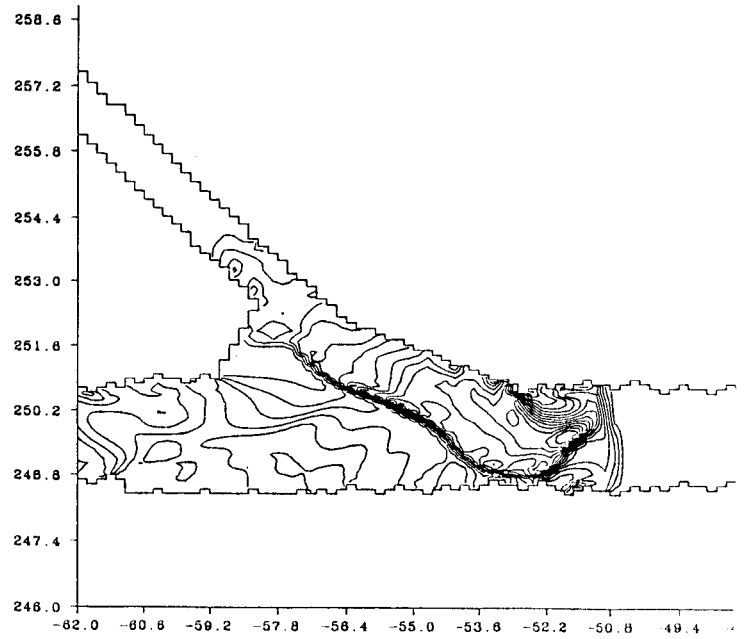
Figure 8. Calculational representation of the entrance to Chamber #2 access tunnel
