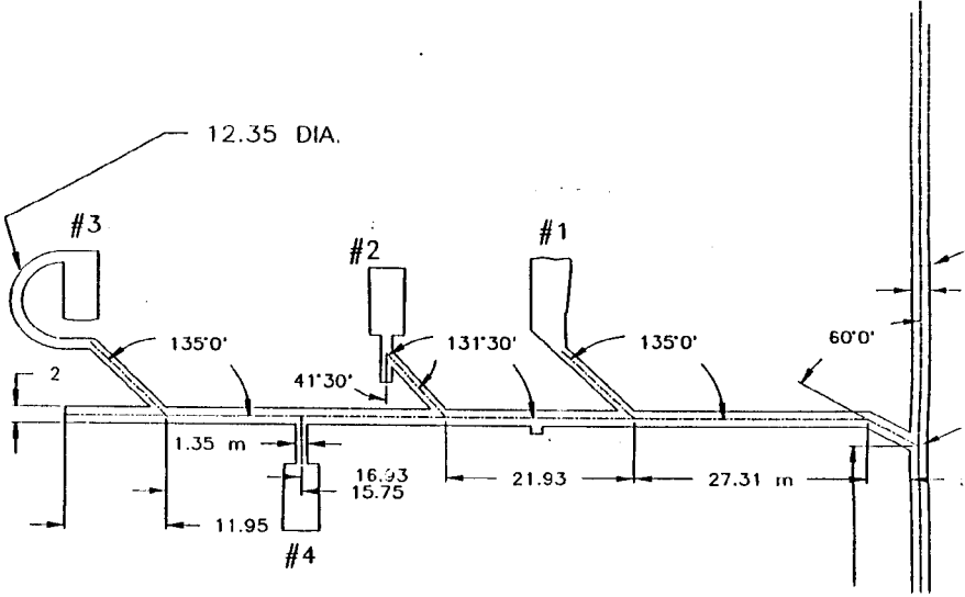
Figure 2. Detail view of left adit, with test chambers #1 through #4
