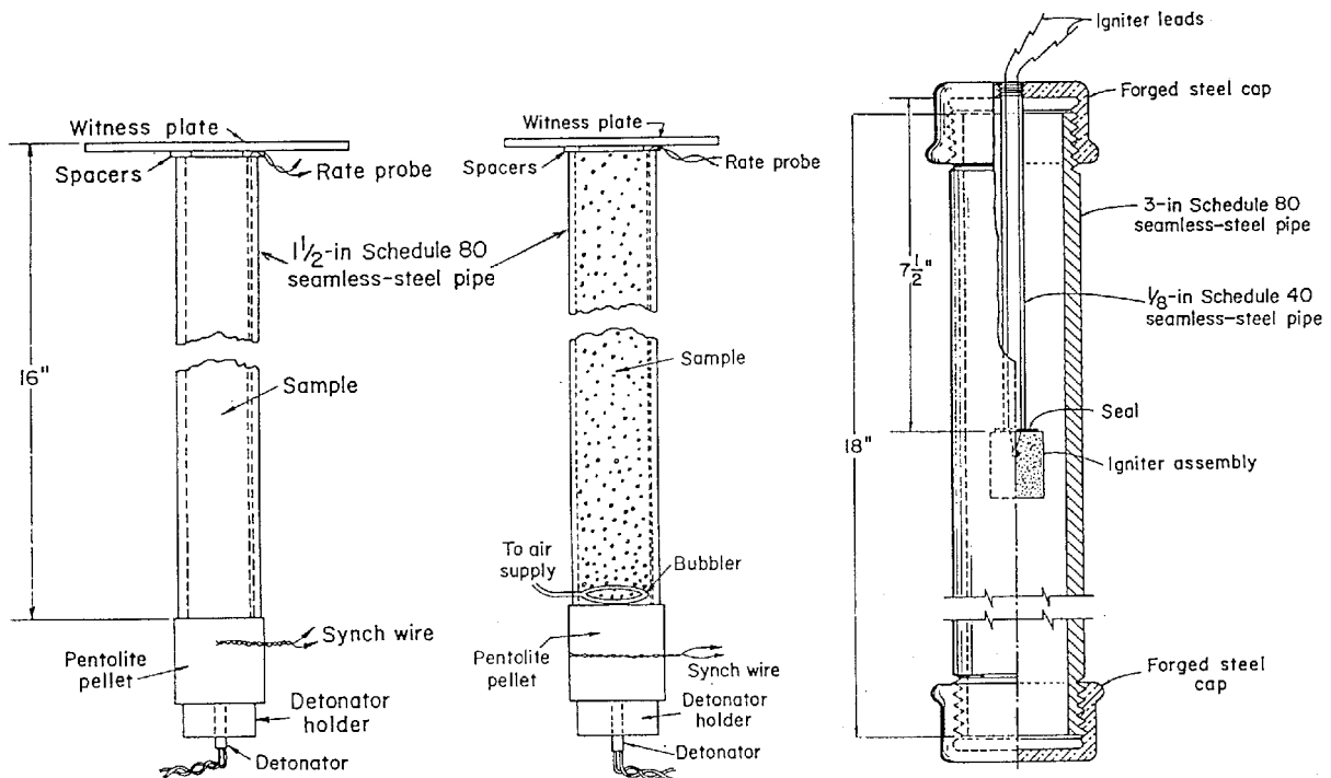
Figure 3.—Bureau of Mines' internal ignition test.
