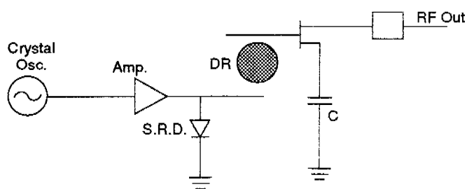
Figure 9a. Injection Locked DRO
