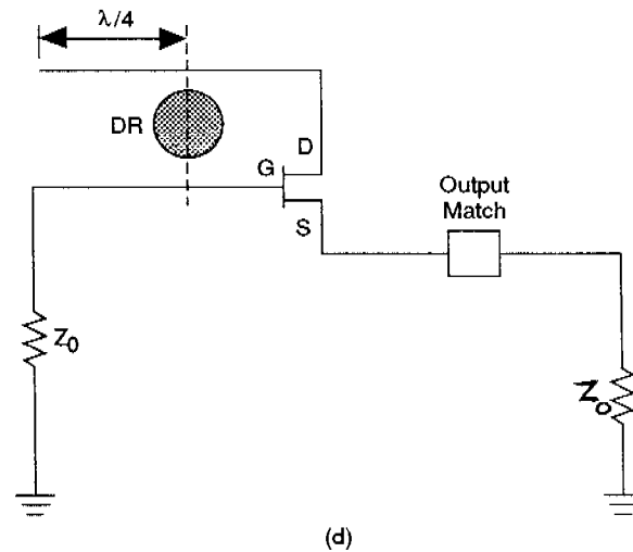
Figure 7. Stable DRO Configurations
