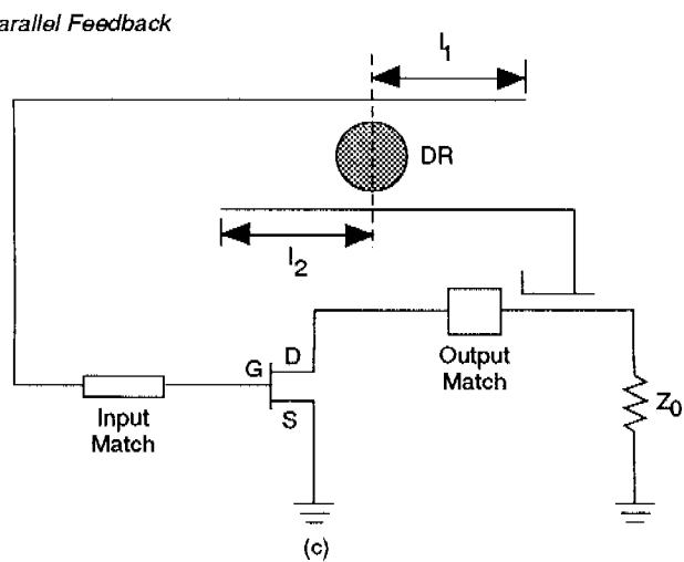
Figure 7. Stable DRO Configurations
