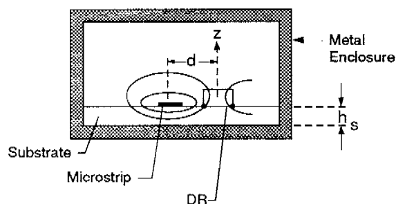
Figure 2. Dielectric Resonator Coupled to a Microstrip Line
