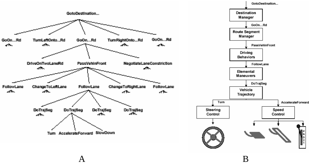
Figure 2-5. NIST Knowledge Representation Schemes for On-road Driving. A) Task decomposition decision tree. B) Hierarchy of agent control modules (source: Barbera et al. 2004a, Figures 3 and 4).
