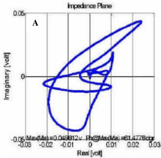
Figure 10: Impedance plane at 0.25" crack & 0.50" thick composite (A) & Summary of test results on detecting titanium layer cracks through graphic epoxy components (B)
