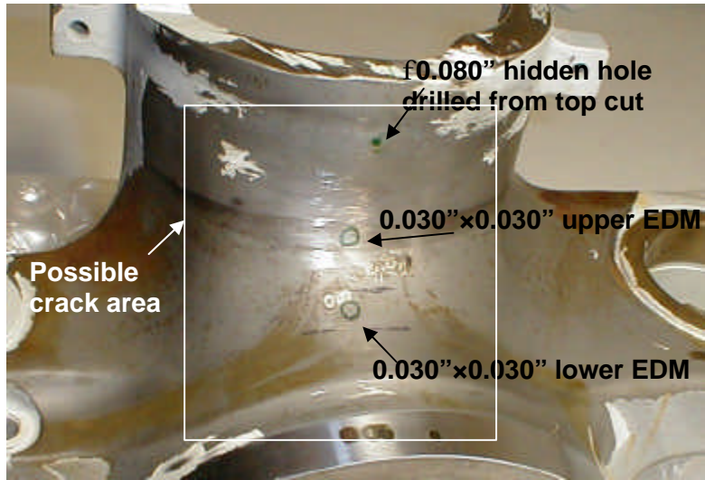
Figure 16: Specimen cut from Airbus A-320 landing gear with two 0.030'' (L) × 0.030'' (D) EDM notches and a φ0.080'' hidden hole on its curved surface
