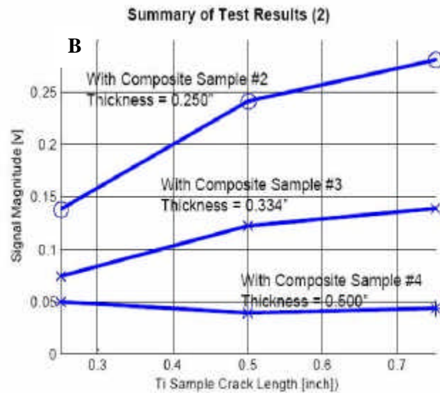
Figure 10: Impedance plane at 0.25" crack & 0.50" thick composite (A) & Summary of test results on detecting titanium layer cracks through graphic epoxy components (B)
