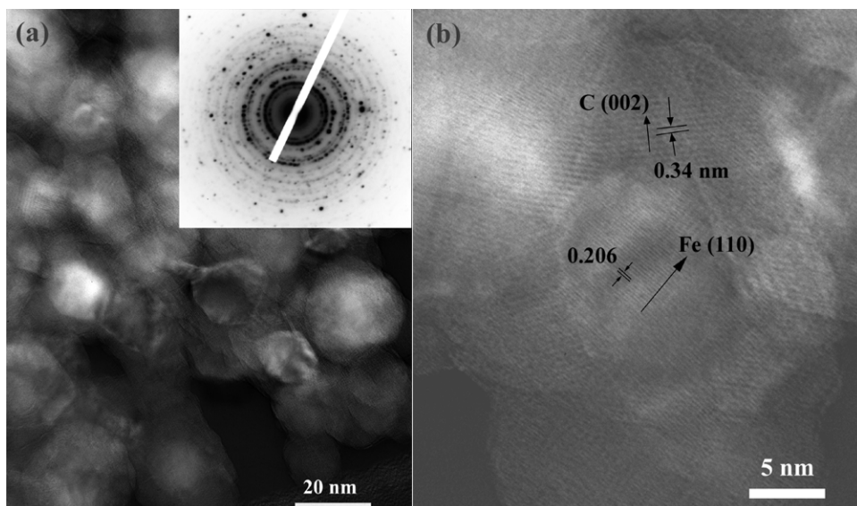
Fig. 2. (a) TEM and (b) HRTEM micrographs of the nanocomposite with a 65 wt% loading after heat treatment at 450 °C. The inset shows SAED.
