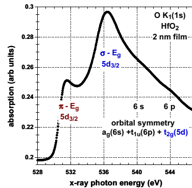
Figure 7(b). O K_1 edge XAS spectrum of \text{HfO}_2 for a film with a physical thickness of 2 nm. The band edge Hf 5d_{3/2} state appears a single feature with no J-T splitting.
