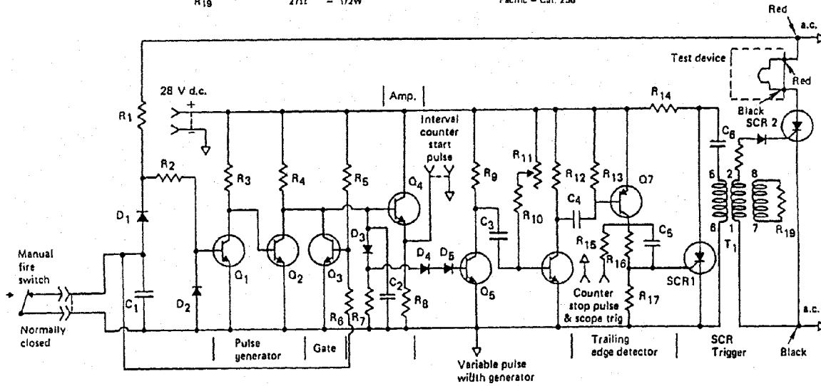
FIGURE 2 - 110, 208, and 440 V a.c. - 60 Hz Firing System.
