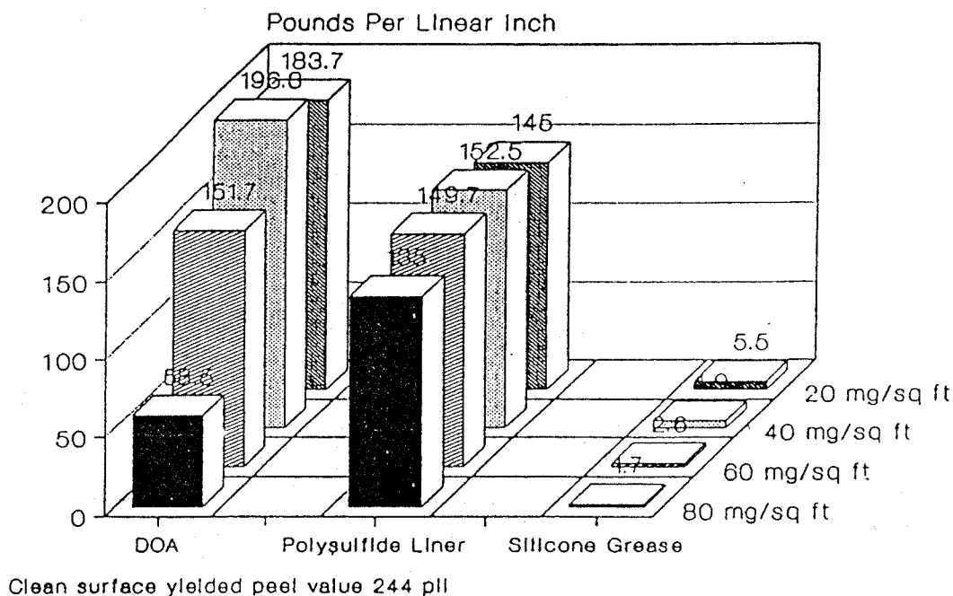
Figure 10: Thiokol/MICOM Data on Sensitivity of Steel Case/HTPB Liner Bond Strength to Various Contaminants
