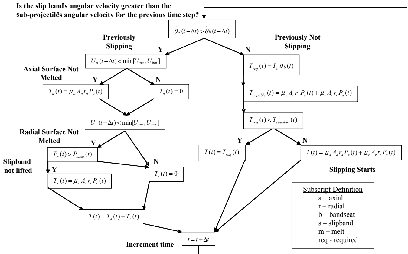
Figure 2. Program logic for calculating the transmitted torque T(t) to the band seat, thus sub-projectile, from the slip band.
